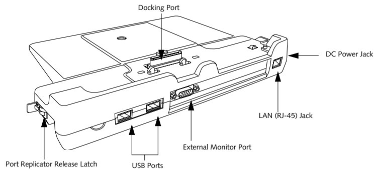
Figure 4-13. Optional Port Replicator rear panel
