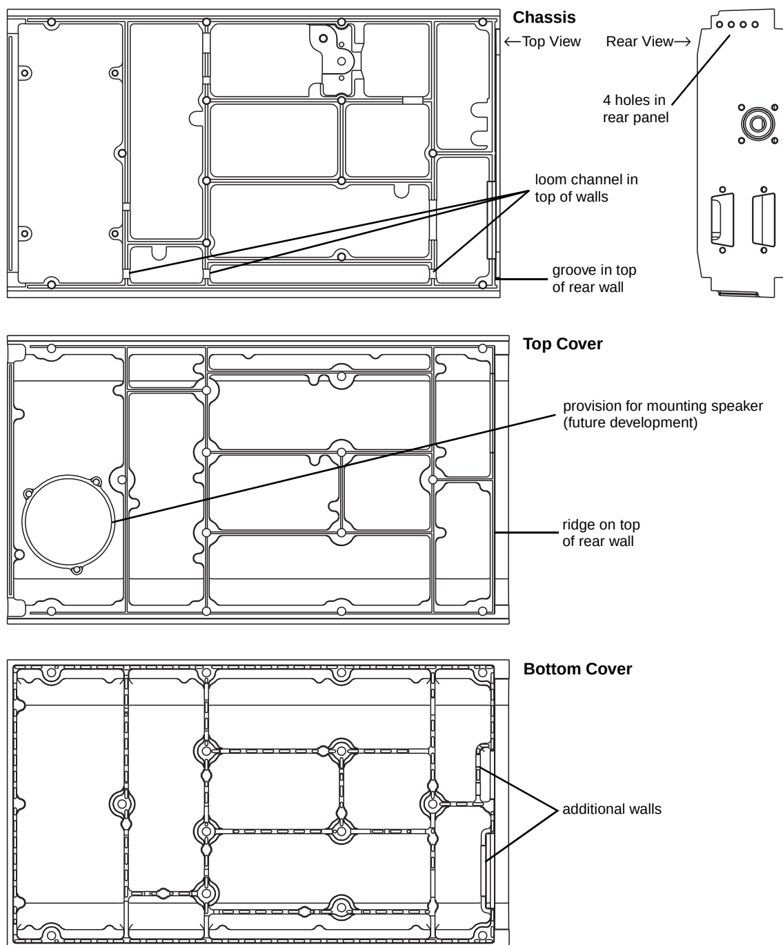
Figure 2.4 Identification Of New-Design Chassis & Covers
