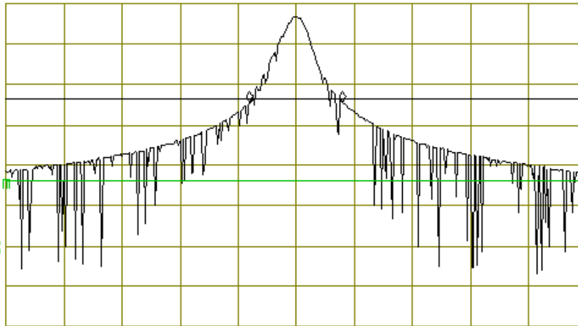
Figure 6.1 Occupied Bandwidth
