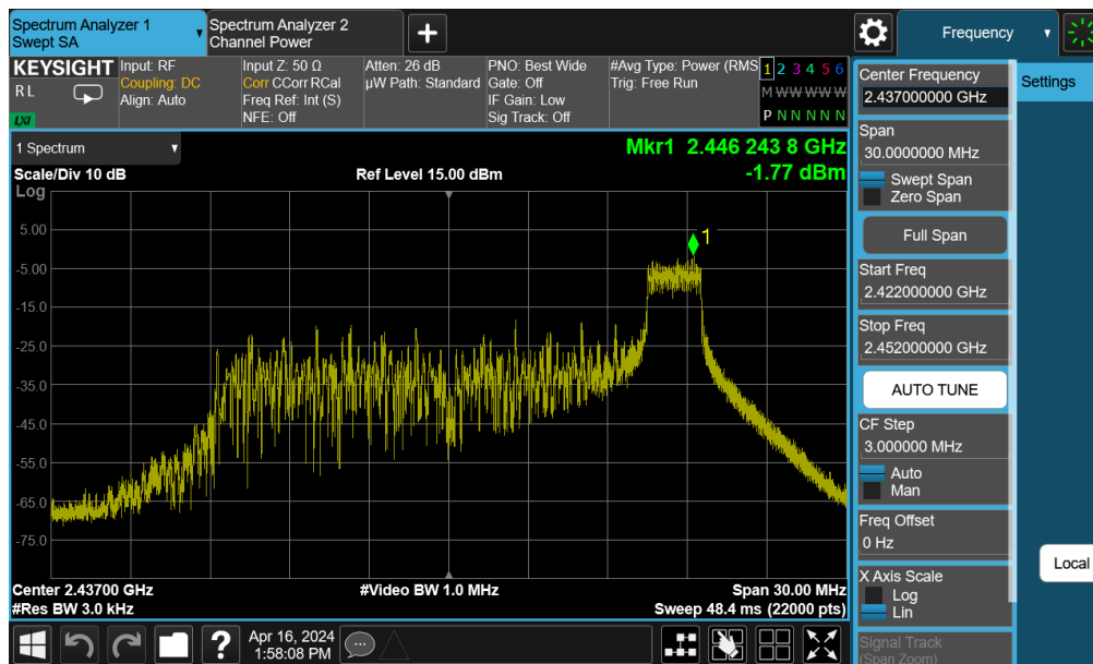
Plot 7-21. Power Spectral Density Plot SISO ANT2 (802.11 be OFDMA – 26 Tones – Ch. 6)
