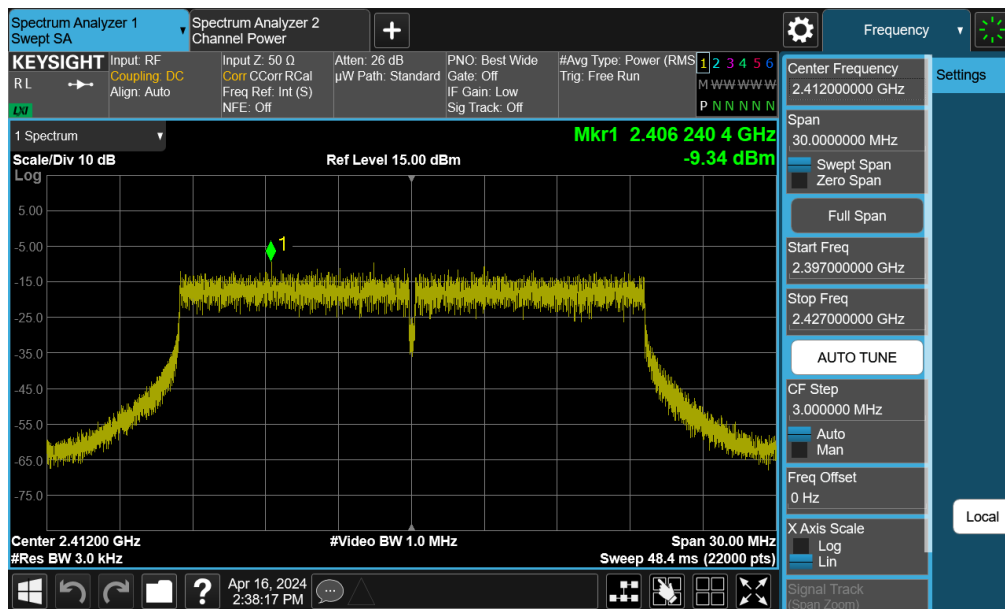
Plot 7-23. Power Spectral Density Plot SISO ANT2 (802.11 be OFDMA – 242 Tones – Ch. 1)
