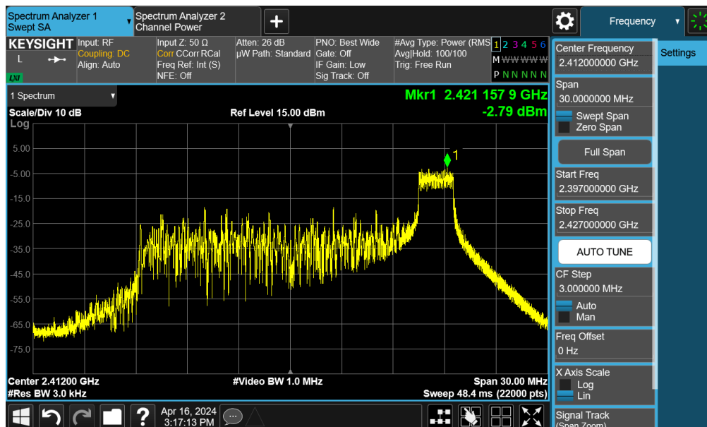
Plot 7-32. Power Spectral Density Plot MIMO ANT2 (802.11be OFDMA – 26 Tones – Ch. 1)
