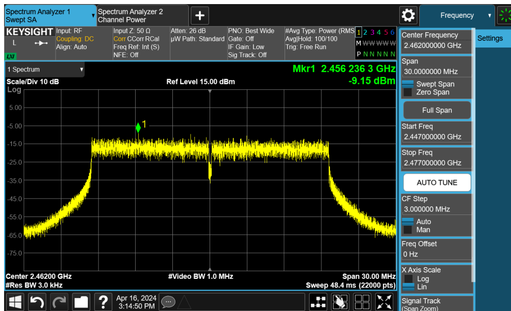
Plot 7-37. Power Spectral Density Plot MIMO ANT2 (802.11be OFDMA – 242 Tones – Ch. 11)
