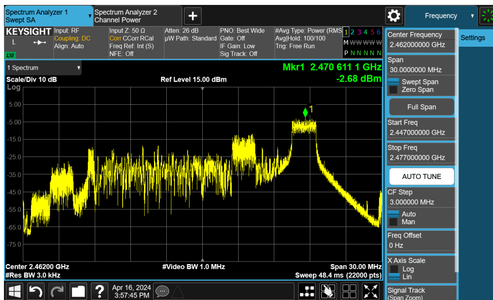
Plot 7-28. Power Spectral Density Plot MIMO ANT1 (802.11be OFDMA – 26 Tones – Ch. 11)
