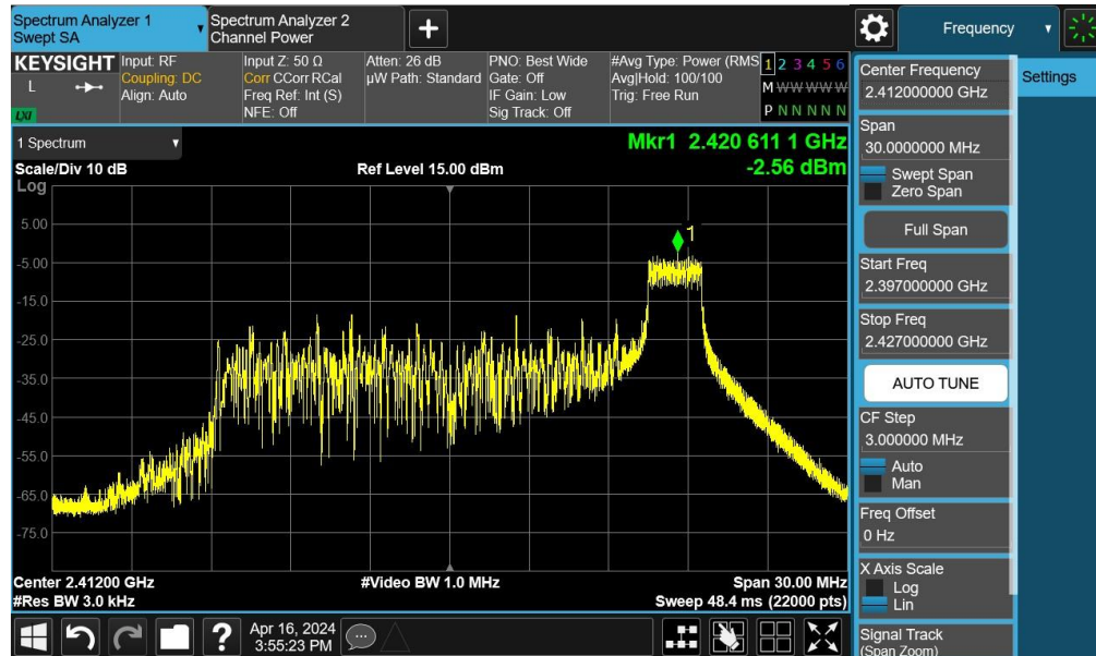
Plot 7-26. Power Spectral Density Plot MIMO ANT1 (802.11be OFDMA – 26 Tones – Ch. 1)
