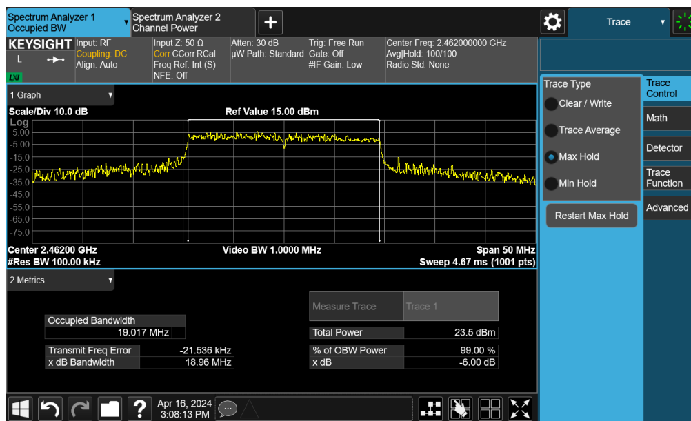
Plot 7-19. 6dB Bandwidth Plot MIMO ANT2 (802.11be OFDMA – 242Tones – Ch. 11)
