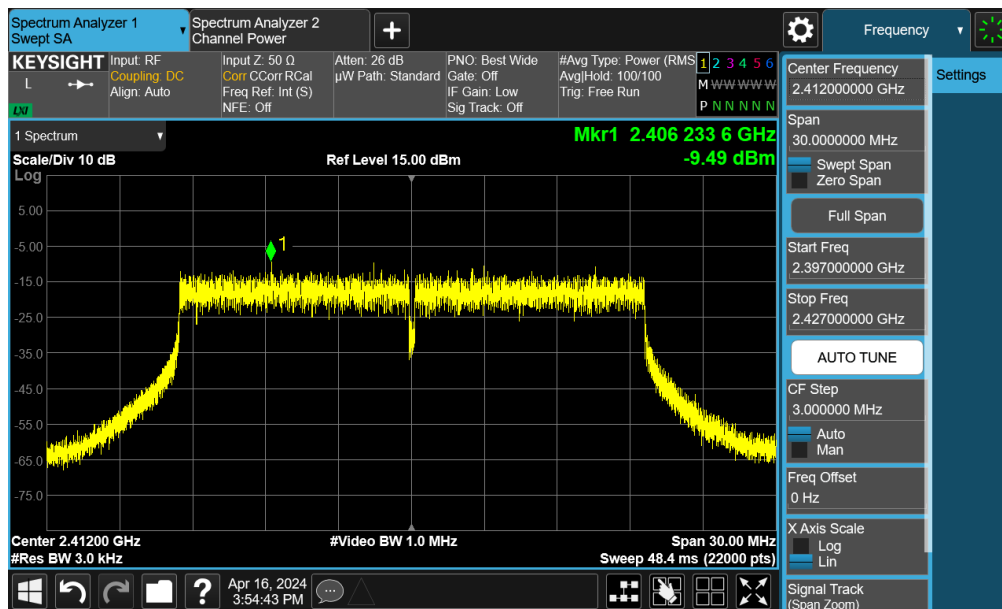
Plot 7-29. Power Spectral Density Plot MIMO ANT1 (802.11be OFDMA – 242 Tones – Ch. 1)
