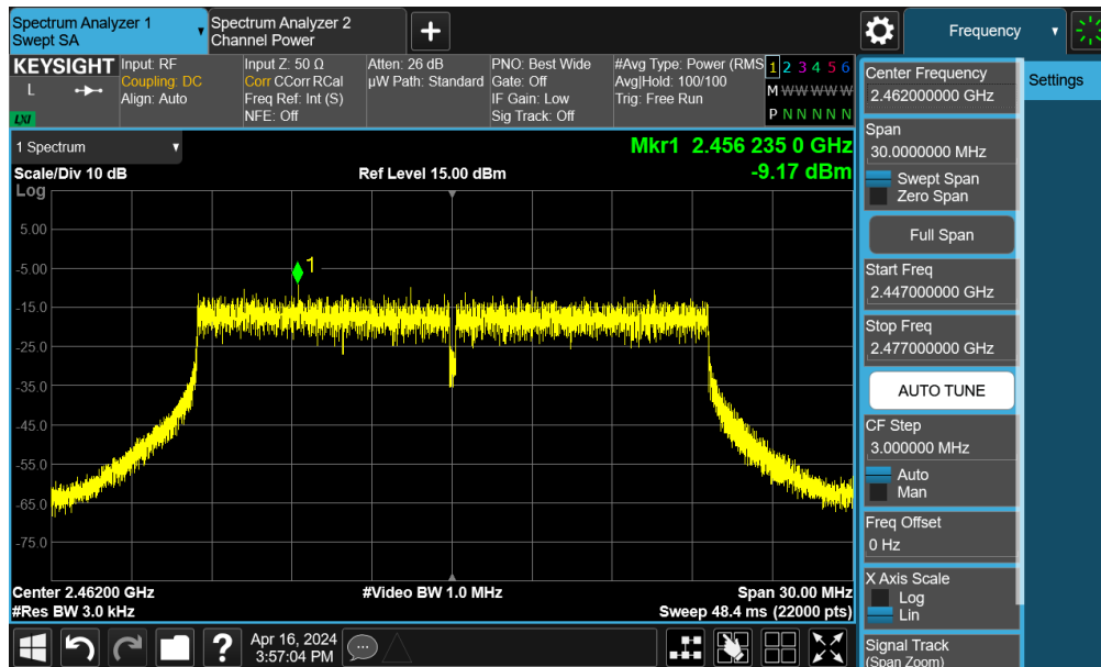
Plot 7-31. Power Spectral Density Plot MIMO ANT1 (802.11be OFDMA – 242 Tones – Ch. 11)
