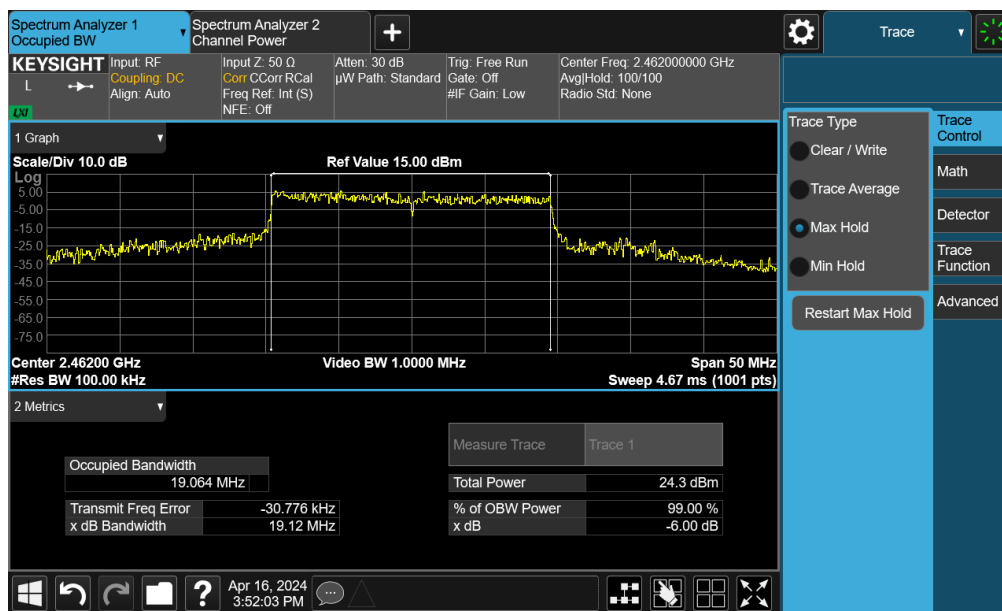
Plot 7-13. 6dB Bandwidth Plot MIMO ANT1 (802.11be OFDMA – 242Tones – Ch. 11)
