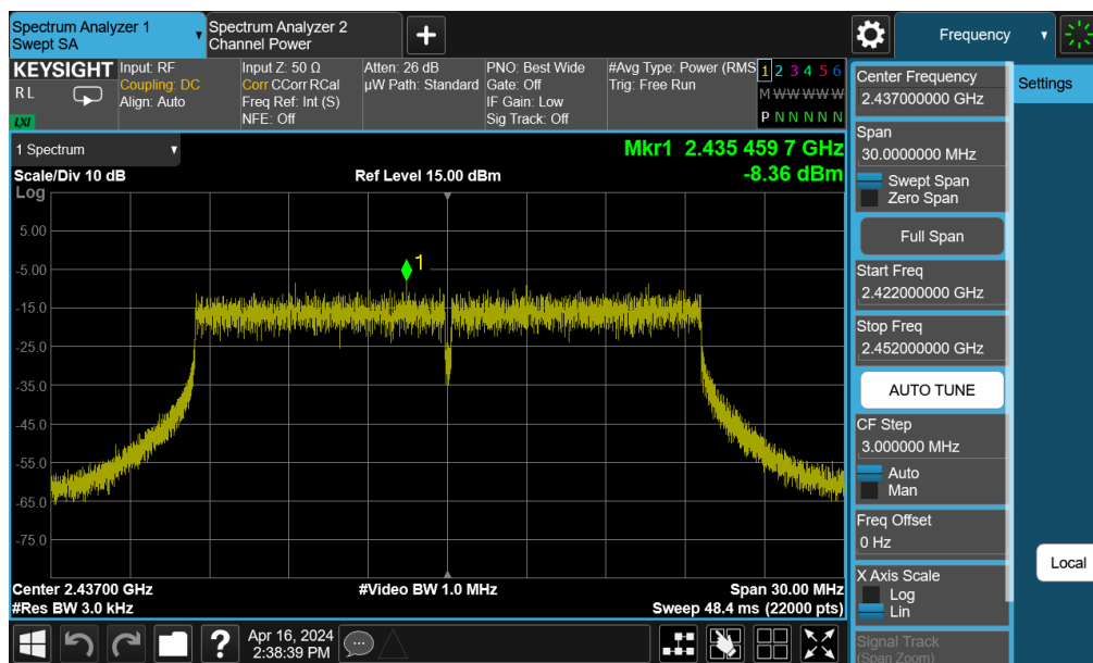
Plot 7-24. Power Spectral Density Plot SISO ANT2 (802.11 be OFDMA – 242 Tones – Ch. 6)
