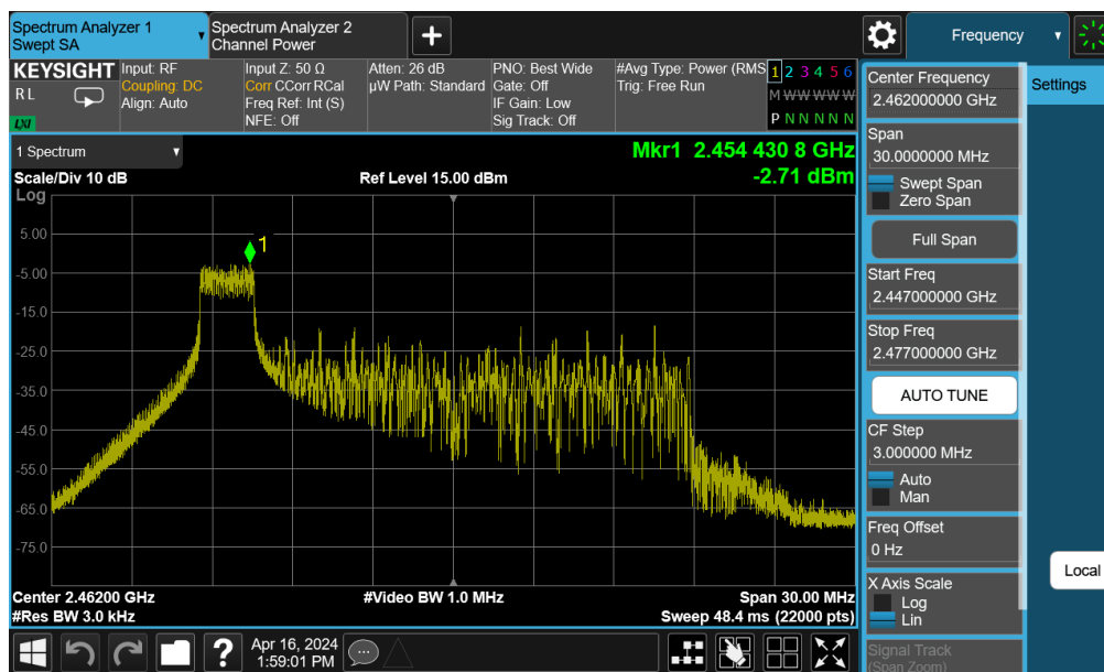
Plot 7-22. Power Spectral Density Plot SISO ANT2 (802.11 be OFDMA – 26 Tones – Ch. 11)
