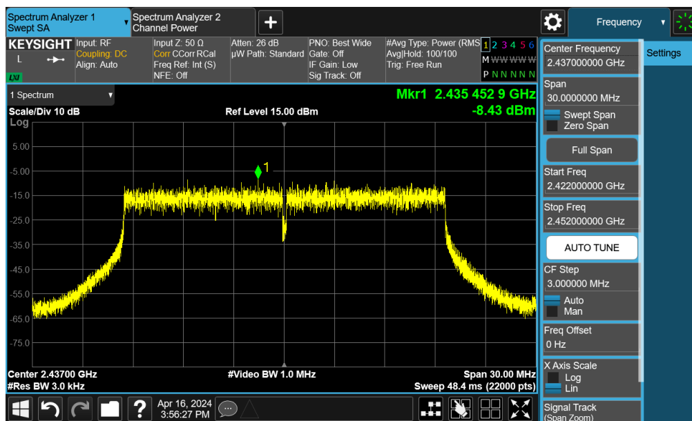
Plot 7-30. Power Spectral Density Plot MIMO ANT1 (802.11be OFDMA – 242 Tones – Ch. 6)
