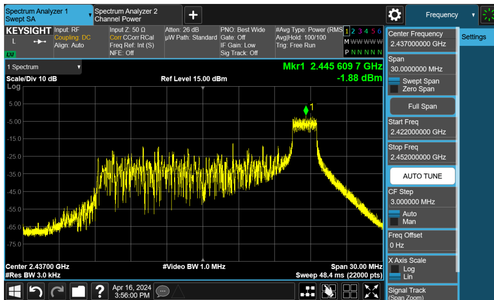
Plot 7-27. Power Spectral Density Plot MIMO ANT2 (802.11be OFDMA – 26 Tones – Ch. 6)
