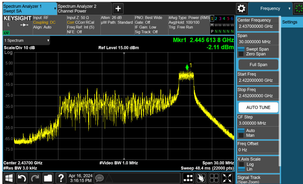
Plot 7-33. Power Spectral Density Plot MIMO ANT2 (802.11be OFDMA – 26 Tones – Ch. 6)
