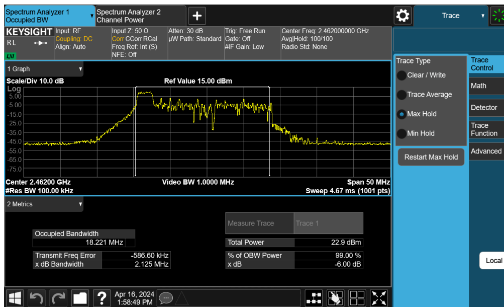
Plot 7-4. 6dB Bandwidth Plot SISO ANT2 (802.11be OFDMA – 26 Tones – Ch. 11)
