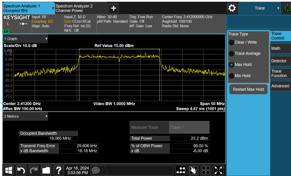
Plot 7-11. 6dB Bandwidth Plot MIMO ANT1 (802.11be OFDMA – 242Tones – Ch. 1)
