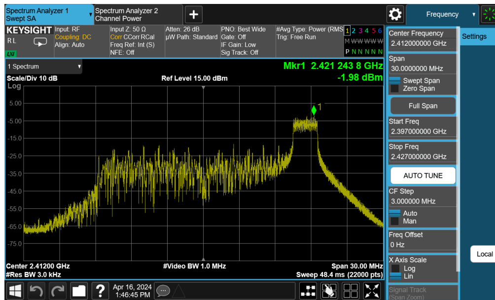
Plot 7-20. Power Spectral Density Plot SISO ANT2 (802.11be OFDMA – 26 Tones – Ch. 1)
