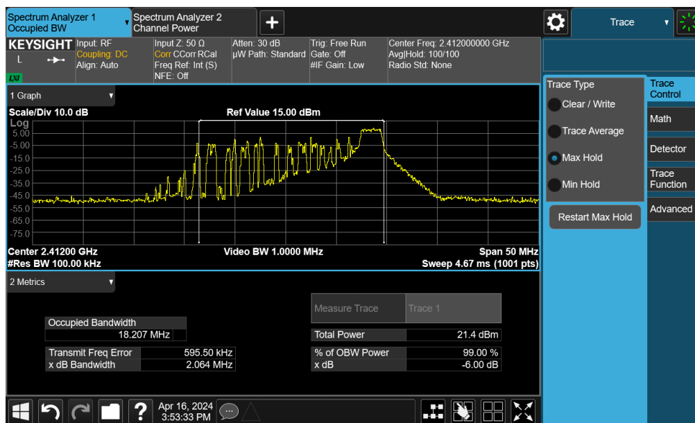
Plot 7-8. 6dB Bandwidth Plot MIMO ANT1 (802.11be OFDMA – 26Tones – Ch. 1)
