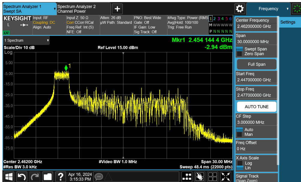
Plot 7-34. Power Spectral Density Plot MIMO ANT2 (802.11be OFDMA – 26 Tones – Ch. 11)
