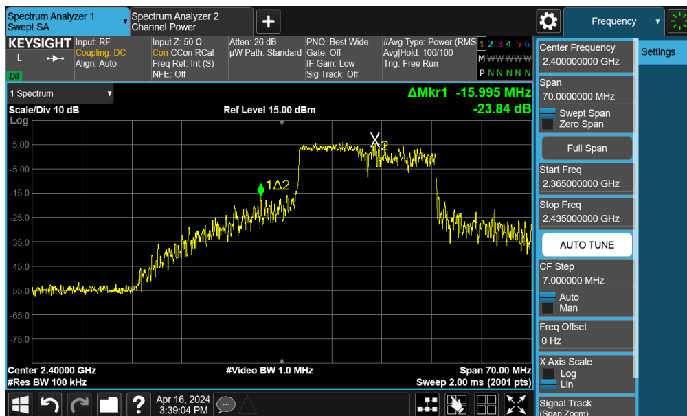
Plot 7-46. Band Edge Plot MIMO ANT1 (802.11be OFDMA – 106 Tones – Ch. 1)
