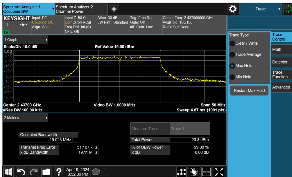
Plot 7-12. 6dB Bandwidth Plot MIMO ANT1 (802.11be OFDMA – 242Tones – Ch. 6)
