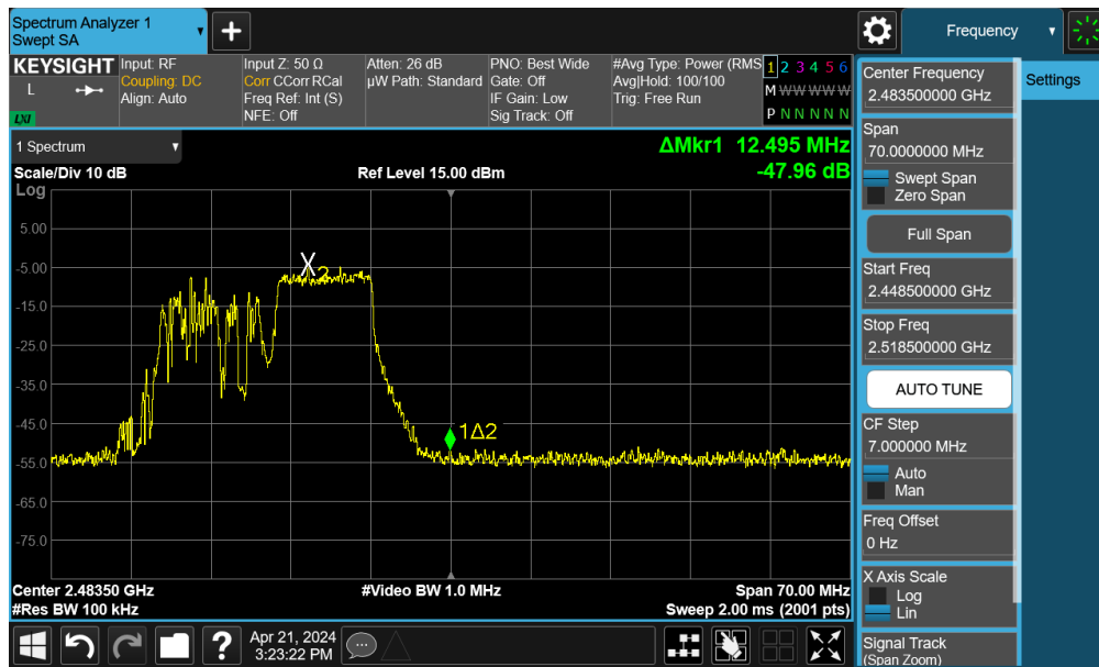
Plot 7-40. Band Edge Plot SISO ANT2 (802.11be OFDMA – 106 Tones – Ch. 12)
