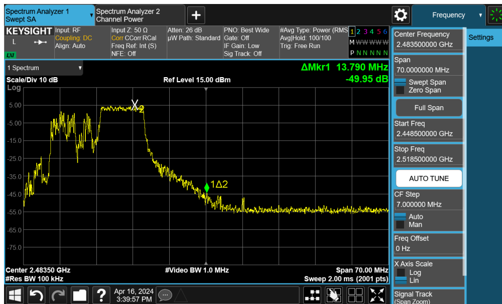
Plot 7-47. Band Edge Plot MIMO ANT1 (802.11be OFDMA – 106 Tones – Ch. 11)
