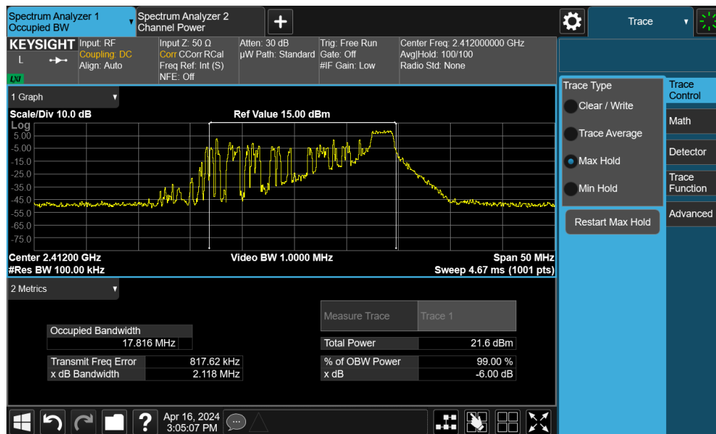
Plot 7-14. 6dB Bandwidth Plot MIMO ANT2 (802.11be OFDMA – 26Tones – Ch. 1)
