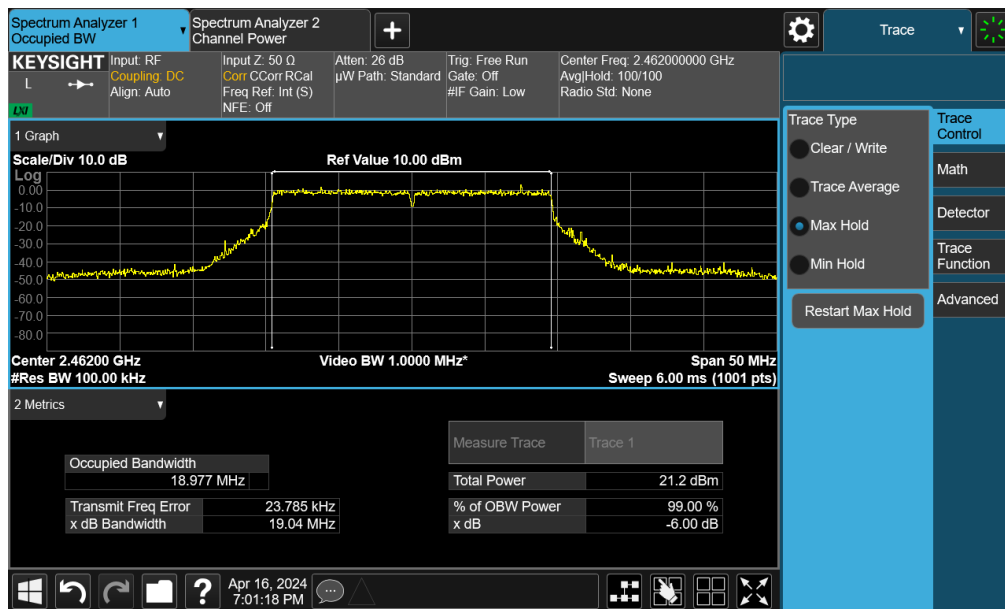
Plot 7-7. 6dB Bandwidth Plot SISO ANT2 (802.11be OFDMA – 242 Tones – Ch. 11)
