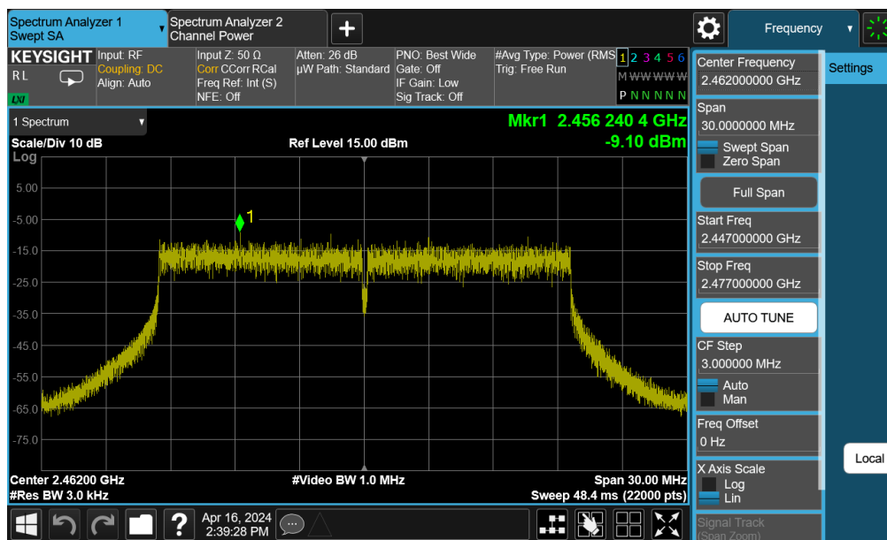
Plot 7-25. Power Spectral Density Plot SISO ANT2 (802.11 be OFDMA – 242 Tones – Ch. 11)
