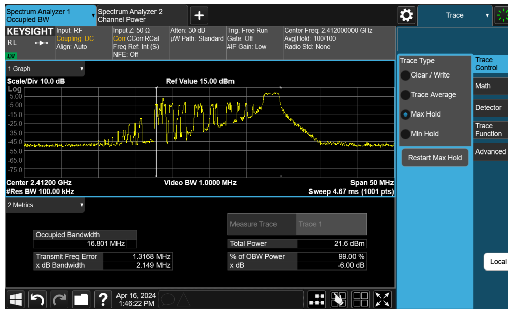
Plot 7-2. 6dB Bandwidth Plot SISO ANT2 (802.11be OFDMA – 26 Tones – Ch. 1)
