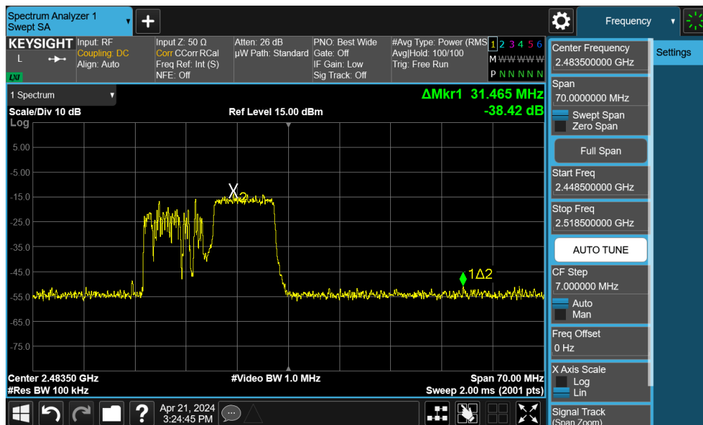
Plot 7-41. Band Edge Plot SISO ANT2 (802.11be OFDMA – 106 Tones – Ch. 13)
