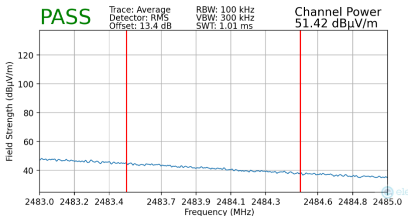
Plot 7-1. Radiated Restricted Upper Band Edge Measurement MIMO (Average) - (Spot-check)
