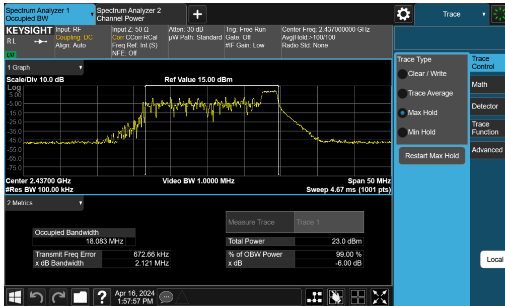
Plot 7-3. 6dB Bandwidth Plot SISO ANT2 (802.11be OFDMA – 26 Tones – Ch. 6)
