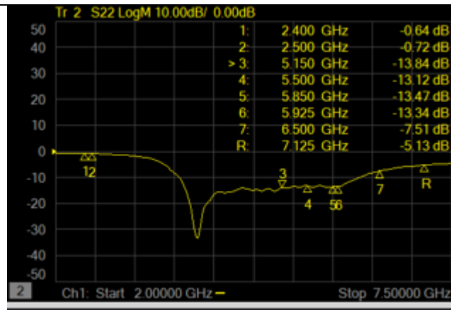
Ant2
