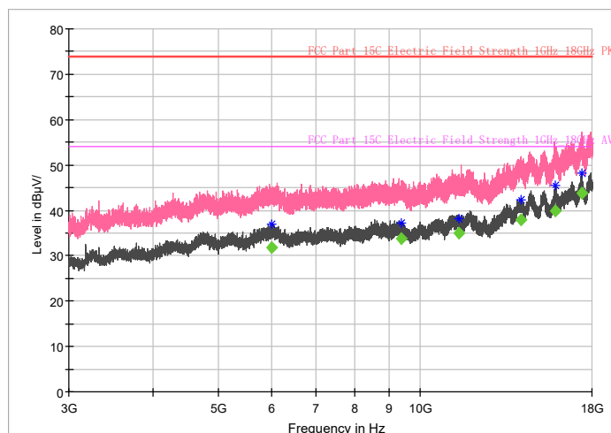
Full Spectrum
