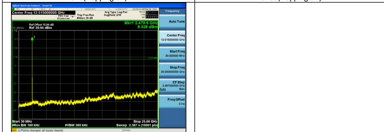
CH78(Hopping off)
