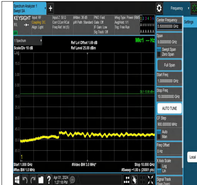
Band5-4182-1-1000~10000MHz-PASS
