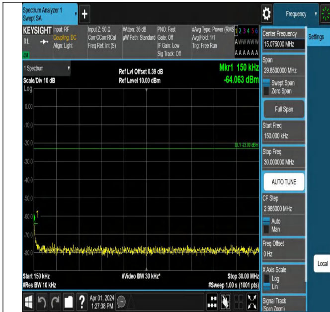
Band5-4233-1-0.15~30MHz-PASS
