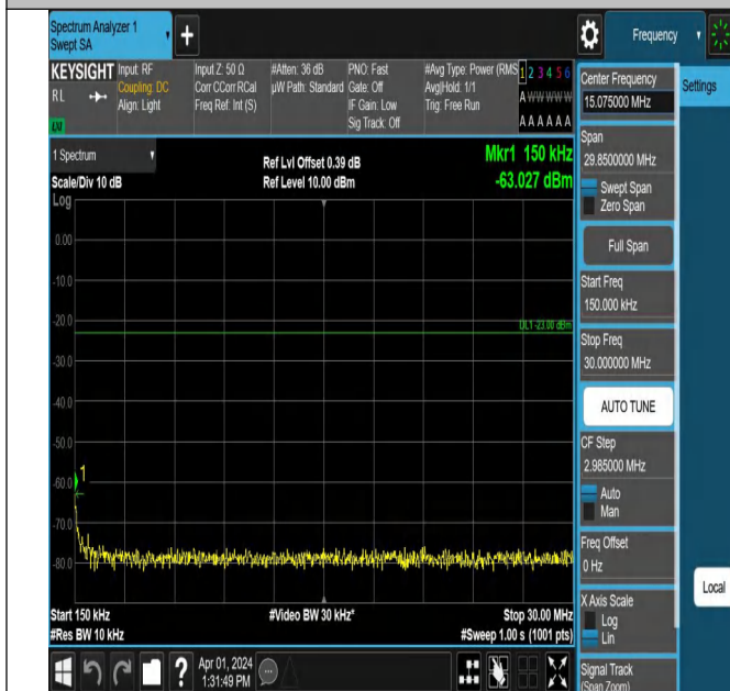
Band5-4233-3-0.15~30MHz-PASS
