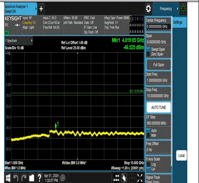
Band5-4132-4-1000~10000MHz-PASS
