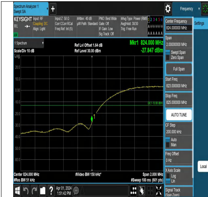
Band5-4132-5-PASS
