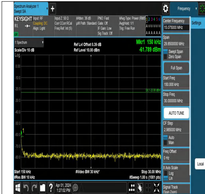
Band5-4182-1-0.15~30MHz-PASS
