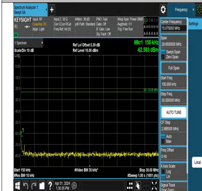
Band5-4132-3-0.15~30MHz-PASS
