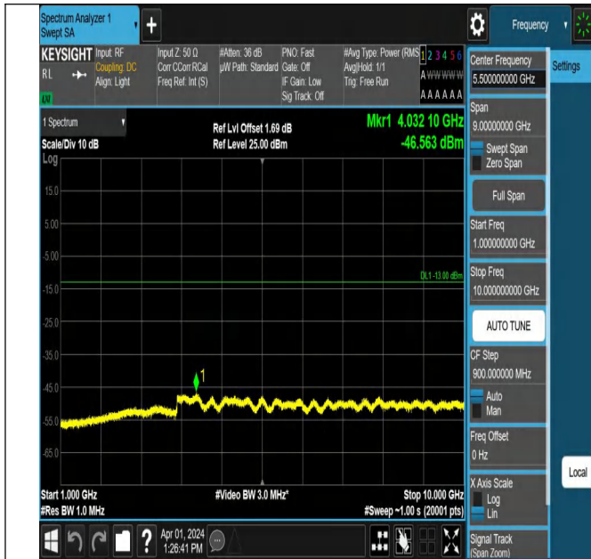
Band5-4132-1-1000~10000MHz-PASS
