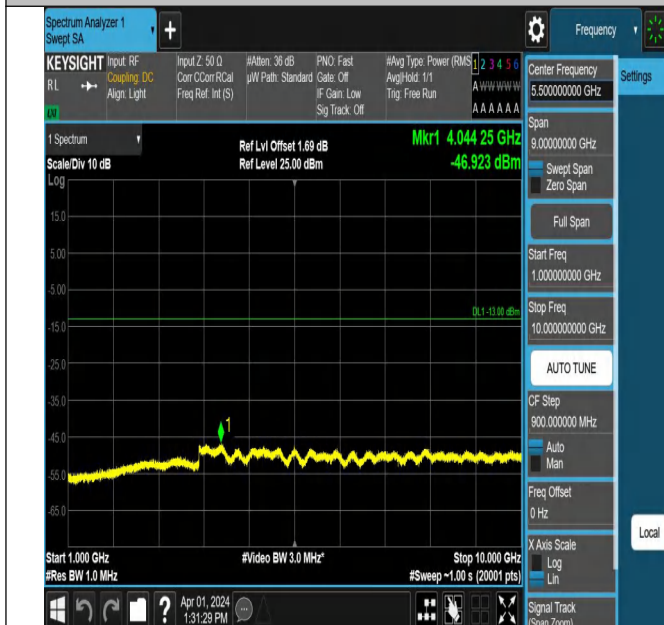
Band5-4182-3-1000~10000MHz-PASS
