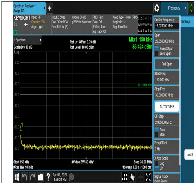
Band5-4132-1-0.15~30MHz-PASS
