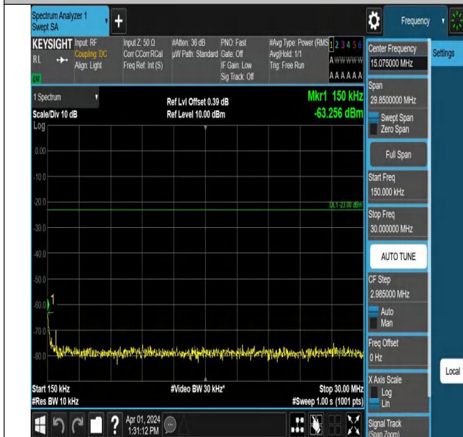
Band5-4182-3-0.15~30MHz-PASS
