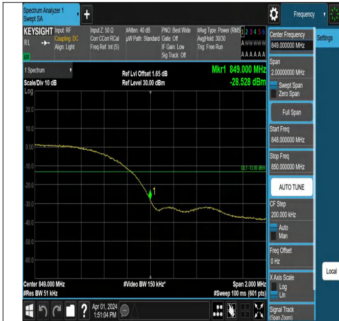
Band5-4233-4-PASS
