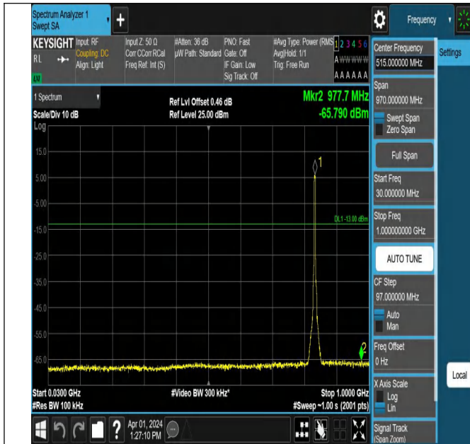
Band5-4182-1-30~1000MHz-PASS
