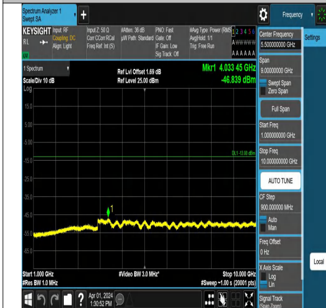
Band5-4132-3-1000~10000MHz-PASS
