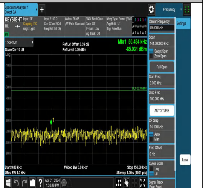
Band5-4233-4-0.009~0.15MHz-PASS
