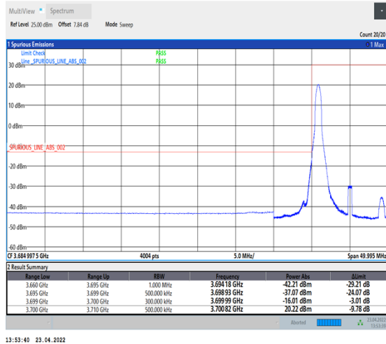
1-N77-3700-3980-PC2-30-10-L-4-CP-QPSK-Edge_1RB_Left-1@0-Ant1-PASS-see graph
