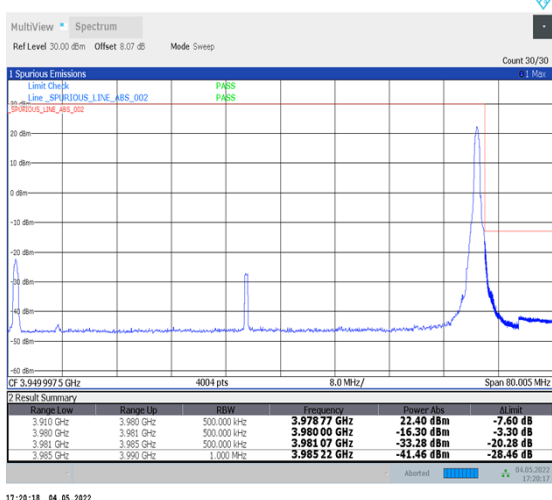
1-N77-3700-3980--30-70-H-5-CP-QPSK-Edge_1RB_Right-1@188-Ant1-PASS-see graph
