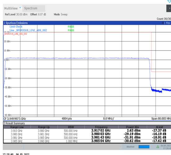
1-N77-3700-3980--30-70-H-6-CP-QPSK-Outer_Full-189@0-Ant1-PASS-see graph
