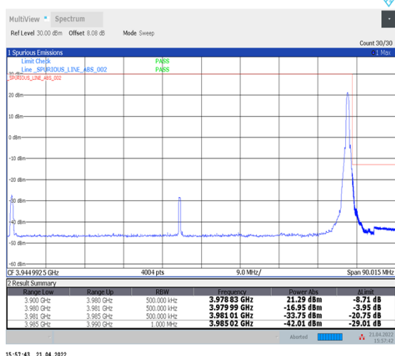
1-N77-3700-3980--30-80-H-5-CP-QPSK-Edge_1RB_Right-1@216-Ant1-PASS-see graph
