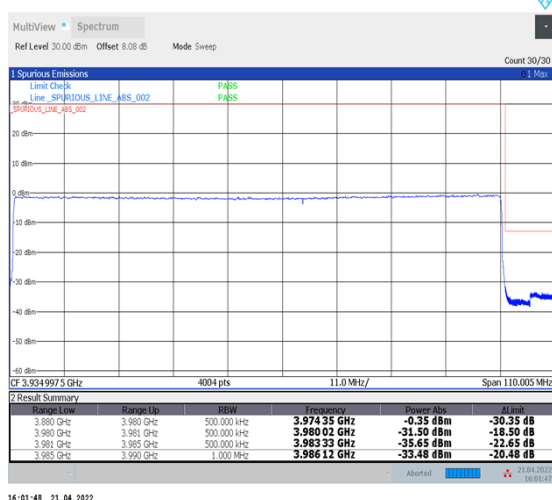
1-N77-3700-3980--30-100-H-6-CP-QPSK-Outer_Full-273@0-Ant1-PASS-see graph
