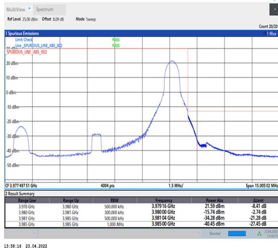
1-N77-3700-3980-PC2-30-10-H-5-CP-QPSK-Edge_1RB_Right-1@23-Ant1-PASS-see graph
