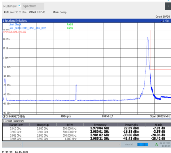
1-N77-3700-3980--30-70-H-2-DFT-PI2BPSK-Edge_1RB_Right-1@188-Ant1-PASS-see graph
