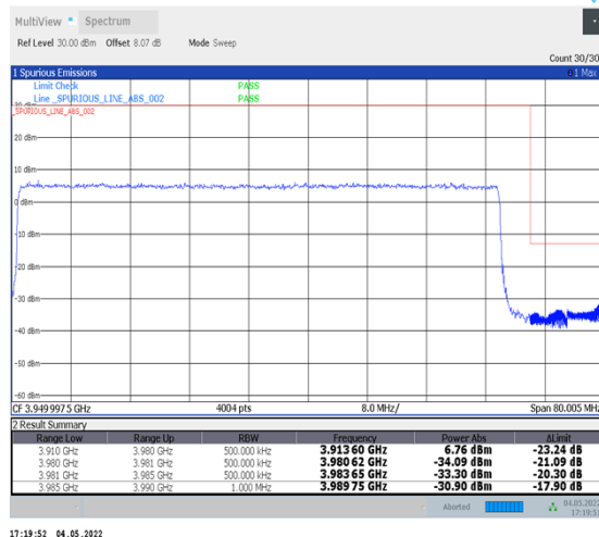
1-N77-3700-3980--30-70-H-3-DFT-PI2BPSK-Outer_Full-180@0-Ant1-PASS-see graph
