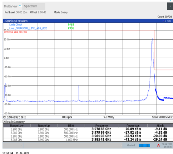
1-N77-3700-3980--30-80-H-2-DFT-PI2BPSK-Edge_1RB_Right-1@216-Ant1-PASS-see graph
