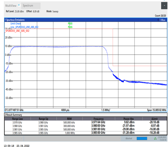
1-N77-3700-3980-PC2-30-10-H-6-CP-QPSK-Outer_Full-24@0-Ant1-PASS-see graph
