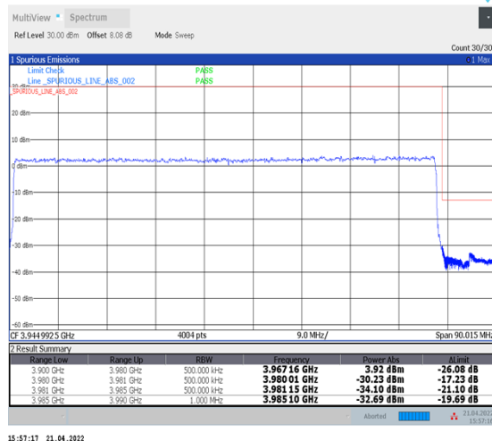
1-N77-3700-3980--30-80-H-3-DFT-PI2BPSK-Outer_Full-216@0-Ant1-PASS-see graph
