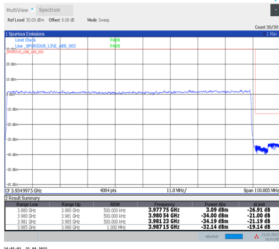
1-N77-3700-3980--30-100-H-3-DFT-PI2BPSK-Outer_Full-270@0-Ant1-PASS-see graph
