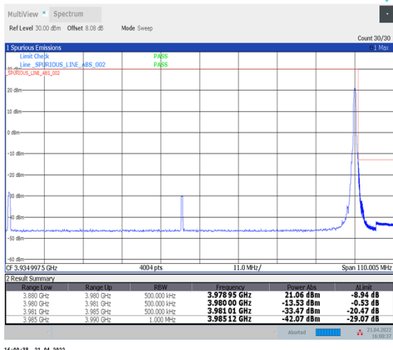
1-N77-3700-3980--30-100-H-2-DFT-PI2BPSK-Edge_1RB_Right-1@272-Ant1-PASS-see graph
