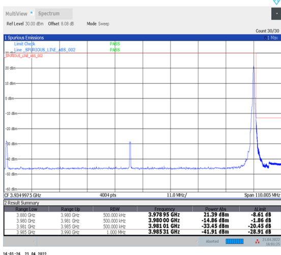
1-N77-3700-3980--30-100-H-5-CP-QPSK-Edge_1RB_Right-1@272-Ant1-PASS-see graph
