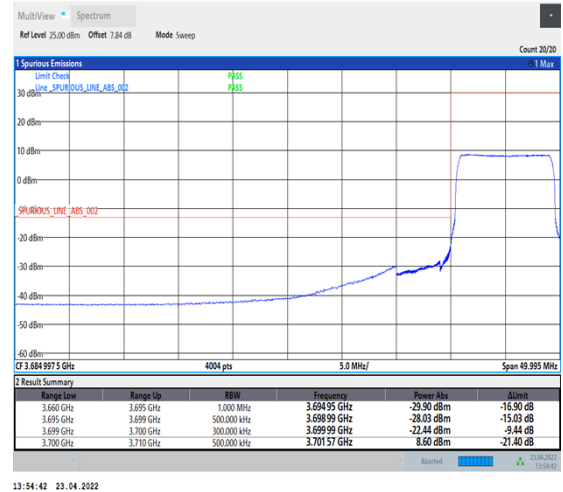
1-N77-3700-3980-PC2-30-10-L-6-CP-QPSK-Outer_Full-24@0-Ant1-PASS-see graph
