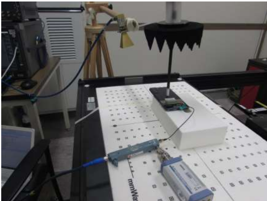
Test setup photo- (9-4 mmW NR radiated power density measurement)
