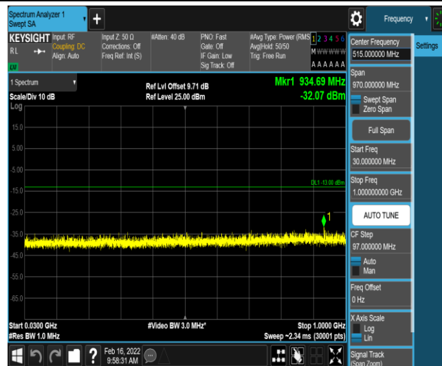
Band66-5MHz-QPSK-132647-1-0-High-30-1000--32.07-PASS
