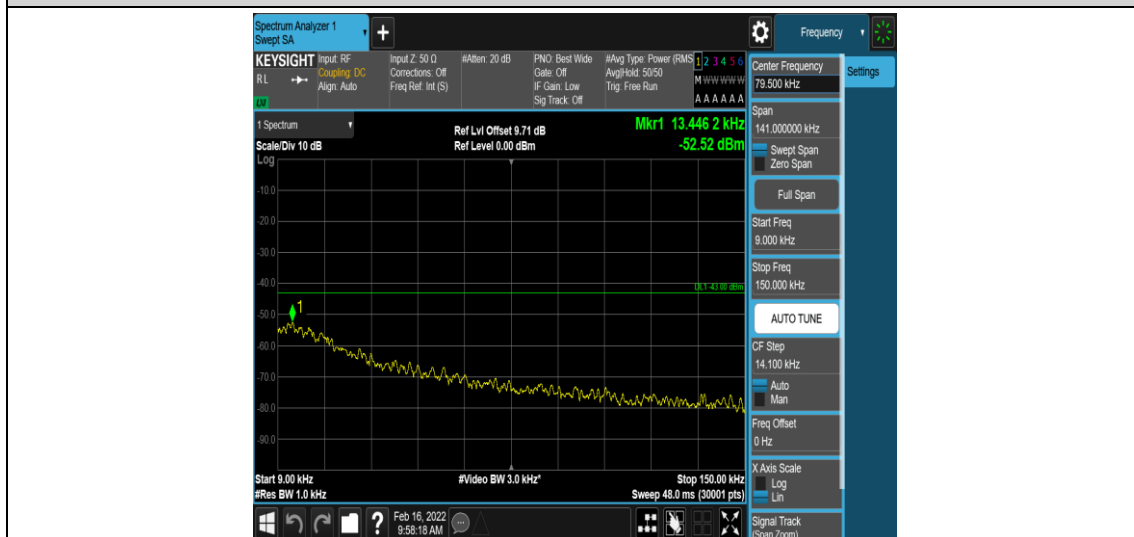
Band66-5MHz-QPSK-132647-1-0-High-0.009-0.15--52.52-PASS
