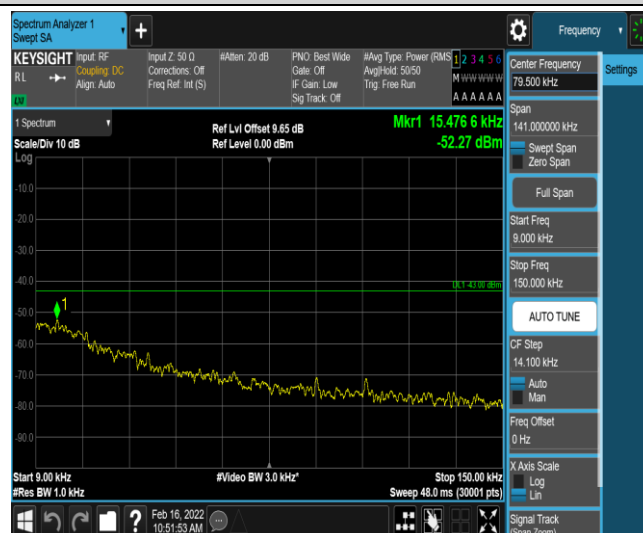
Band66-10MHz-16QAM-132322-1-0-Low-0.009-0.15--52.27-PASS
