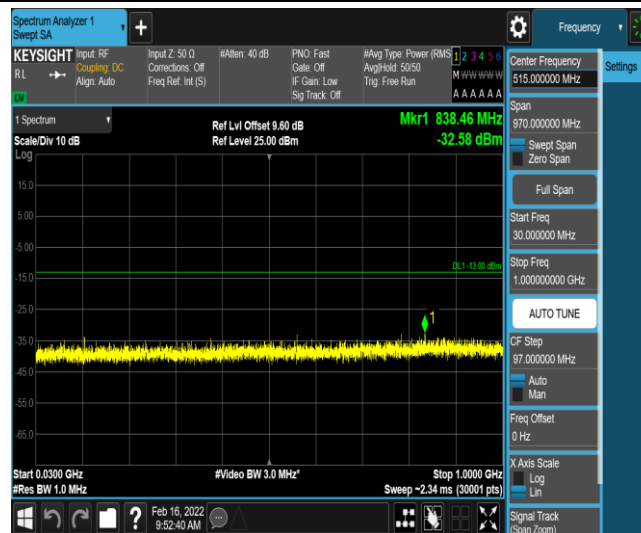
Band66-5MHz-QPSK-131997-1-0-Low-30-1000--32.58-PASS
