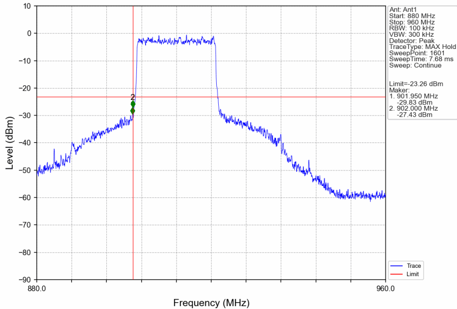
20M_LCH_912MHz_Ant1_NTNV
