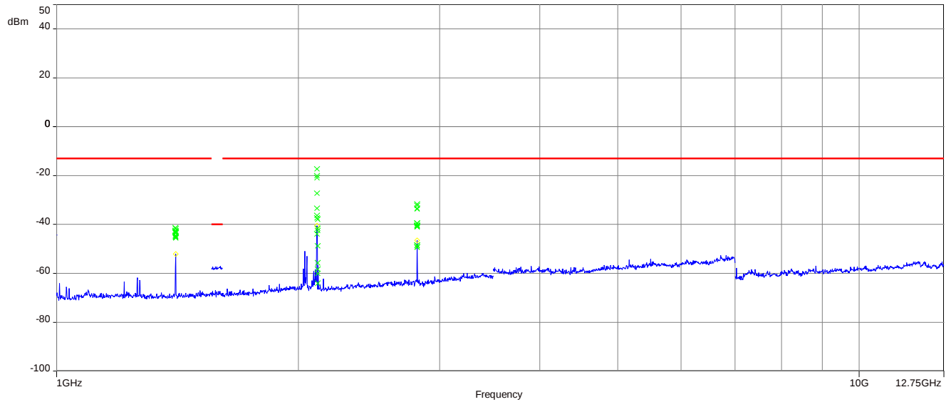
Plot 3: Mid channel (1 GHz – 12.75 GHz)
