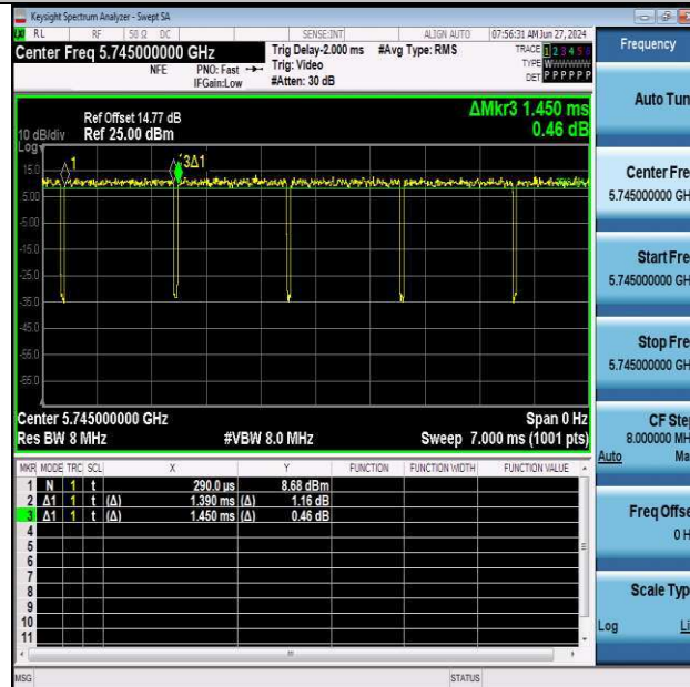
NTNV-11A-Ant2-5745
