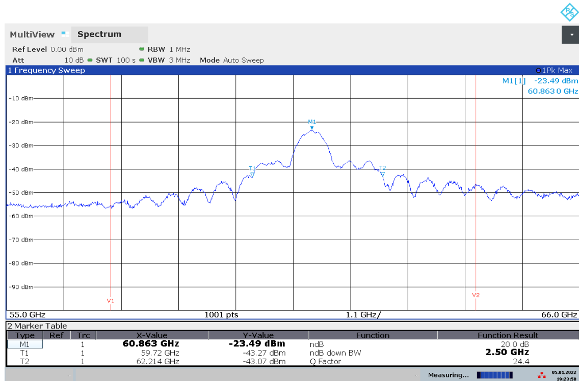
Plot 14: 20 dB Bandwidth at T_{\max}
