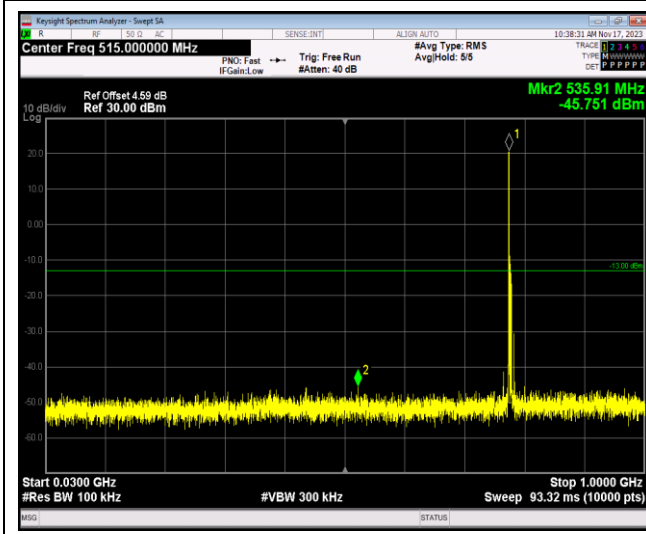
Band13-5MHz-16QAM-23230-1RB#0-Range3:30~1000MHz
