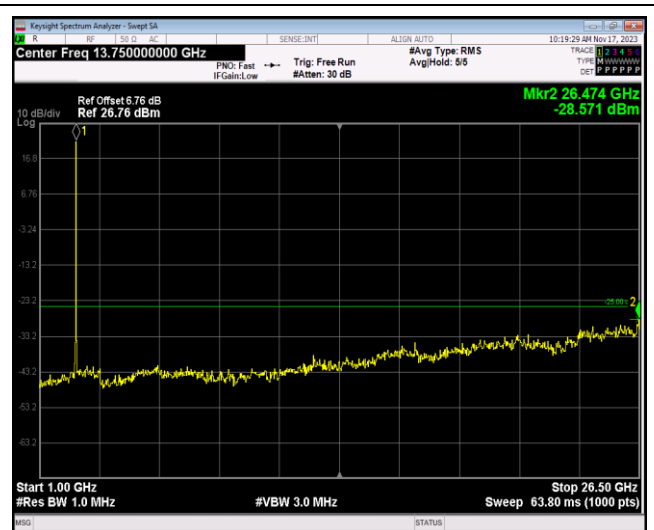
Band7-20MHz-16QAM-20850-1RB#0-Range2:1000~26500MHz
