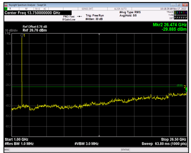
Band7-20MHz-16QAM-21100-1RB#0-Range2:1000~26500MHz
