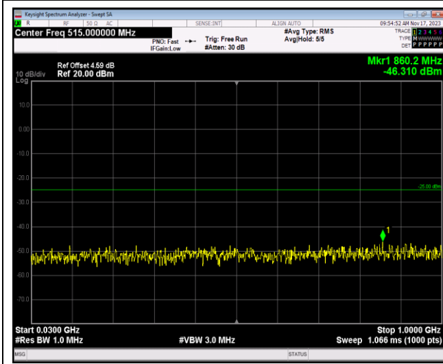
Band7-5MHz-QPSK-20775-1RB#0-Range1:30~1000MHz
