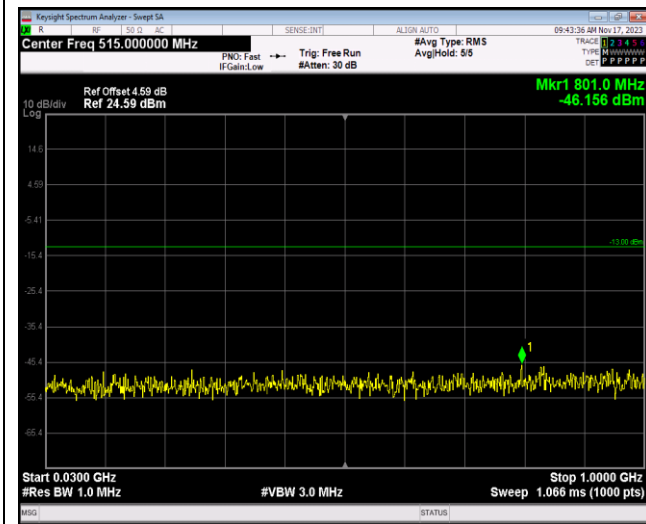
Band7-5MHz-QPSK-20775-1RB#0-Range1:30~1000MHz
