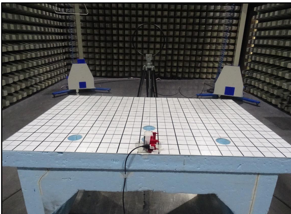
Photo 2 Radiated Test Setup from 9 kHz to 30 MHz
