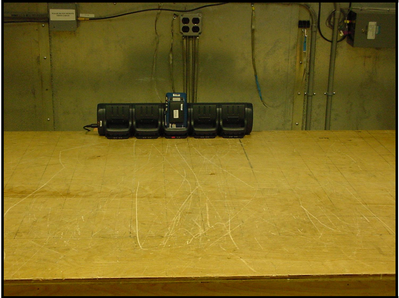
PHOTOGRAPH 4: CONDUCTED EMISSION FRONT VIEW
