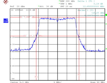
26 dB Bandwidth
