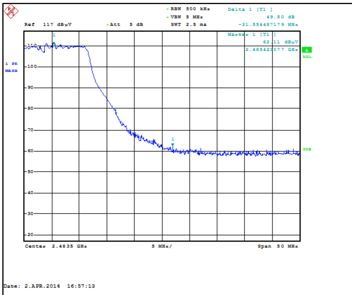
Plot 4-4: In Band Emissions - Channel 13 (2462 MHz); 802.11g (54 Mbps)
