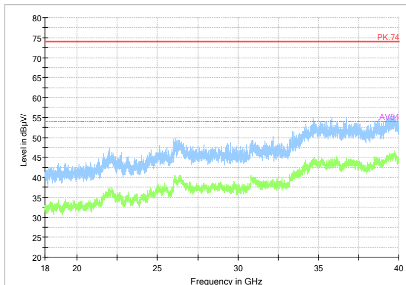
Pic7. Radiated emission (18GHz –40GHz)
