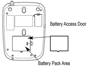
Figure 4 - Battery installation.
