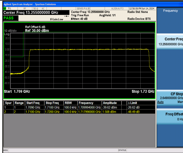
Band66_10MHz_QPSK_132022_50RB#0
