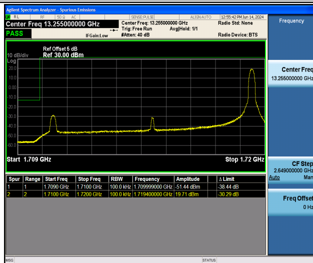
Band66_10MHz_QPSK_132022_1RB#49
