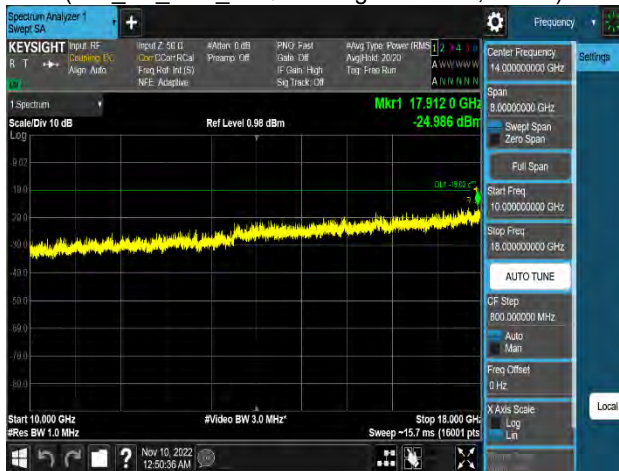
Plot 8-43. Conducted Spurious Emission Plot 10 GHz to 18 GHz (n66_1C_10M_16QAM - High Channel, Port 2)
