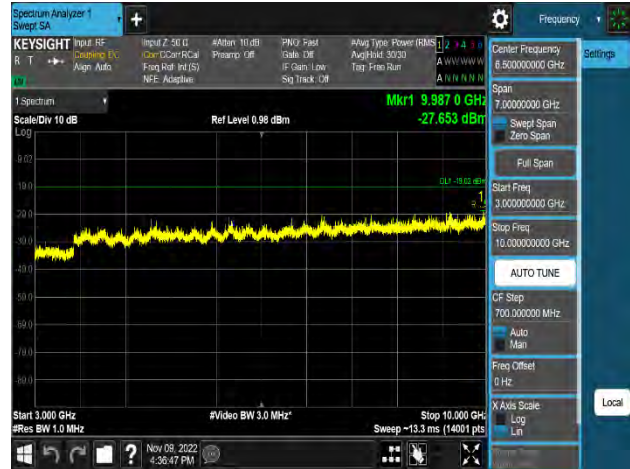
Plot 8-52. Conducted Spurious Emission Plot 3 GHz to 10 GHz (n66_2C_5M+5M_256QAM - Low Channel, Port 0)
