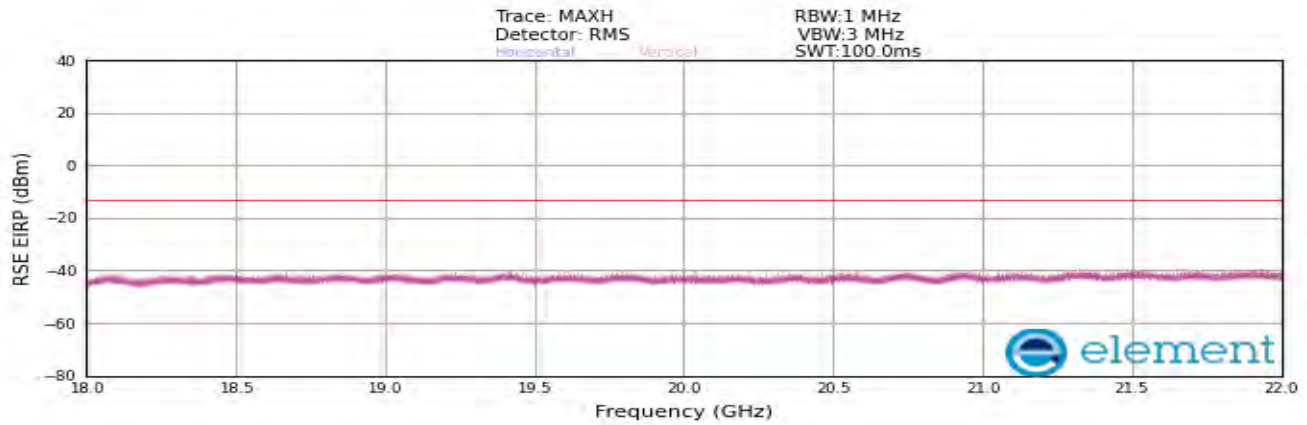
Plot 8-74. Radiated spurious emission Plot_18 GHz to 22 GHz (n66_2C_5M+5M_Mid Channel)
