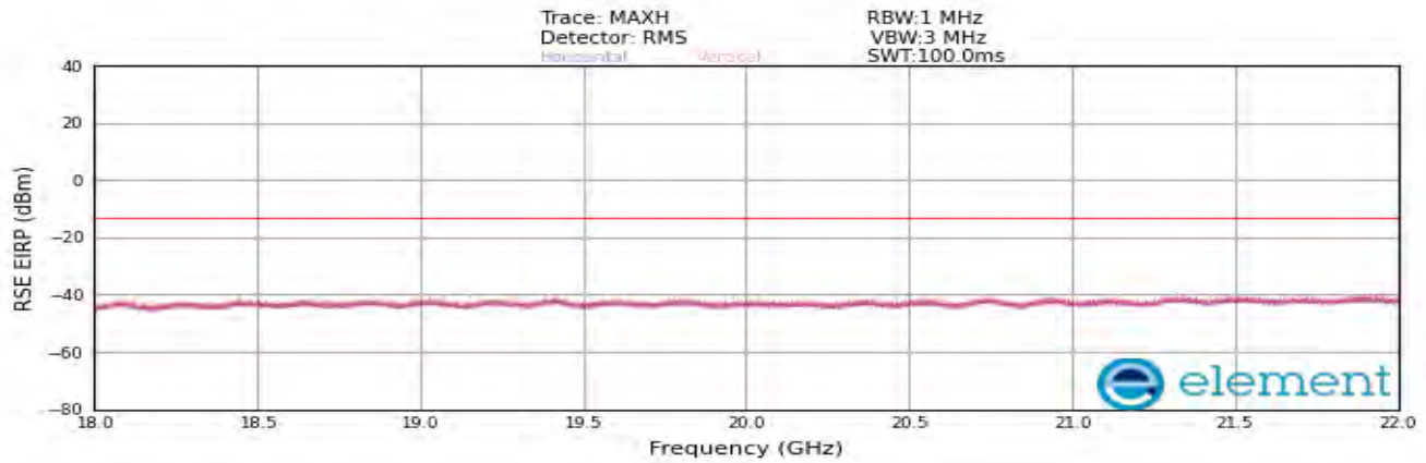
Plot 8-78. Radiated spurious emission Plot_18 GHz to 22 GHz (n66_2NC_5M+5M_Mid Channel)
