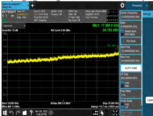
Plot 8-53. Conducted Spurious Emission Plot 10 GHz to 18 GHz (n66_2C_5M+5M_256QAM - Low Channel, Port 0)
