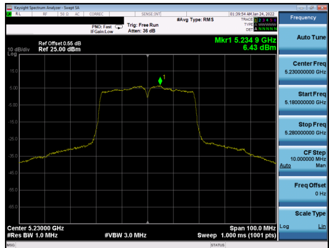
Plot 7-366. PSD SDM Antenna WF7a (40MHz BW 802.11n – Ch. 46, MCS11)
