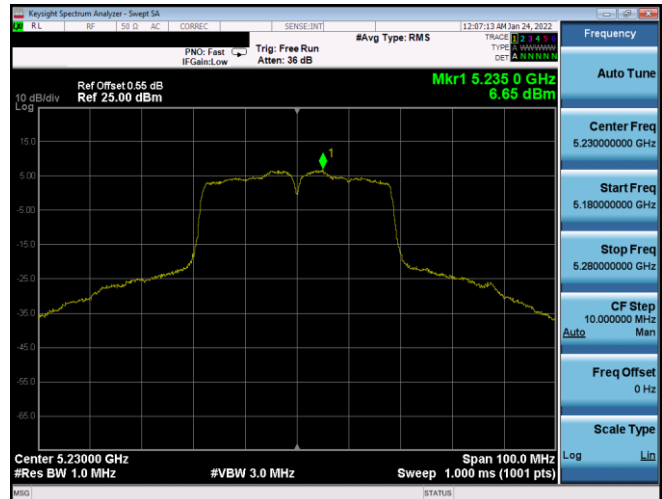
Plot 7-365. PSD SDM Antenna WF8 (40MHz BW 802.11n – Ch. 46, MCS11)
