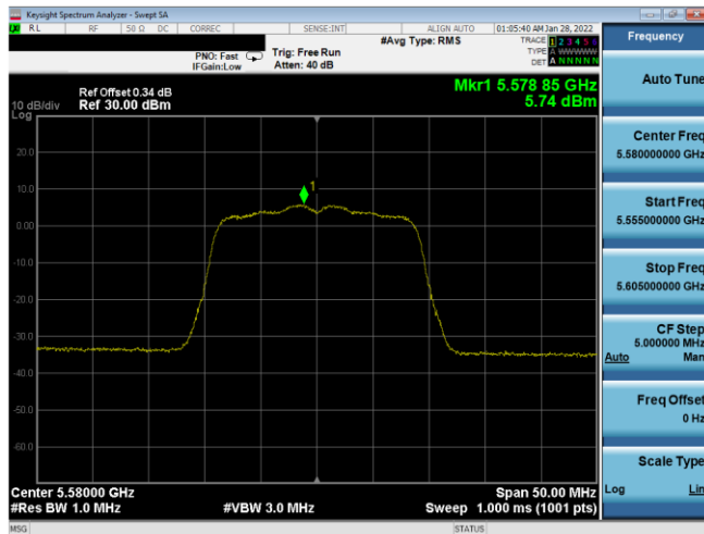
Plot 7-386. PSD SDM Antenna WF7a (20MHz BW 802.11n – Ch. 116, MCS11)
