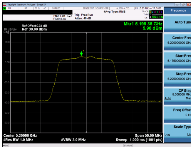
Plot 7-362. PSD SDM Antenna WF7a (20MHz BW 802.11n – Ch. 40, MCS11)
