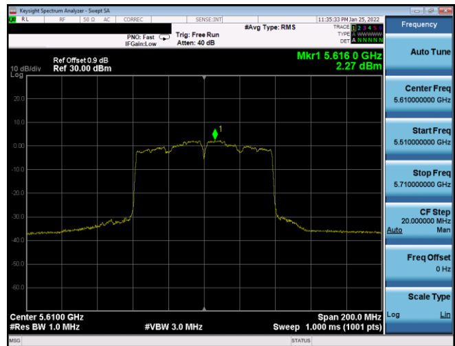
Plot 7-394. PSD CDD Antenna WF7a (80MHz BW 802.11ac – Ch. 122, MCS3)
