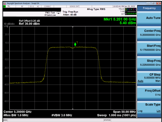
Plot 7-364. PSD SDM Antenna WF7a (20MHz BW 802.11ax(SU) – Ch. 40, MCS3)
