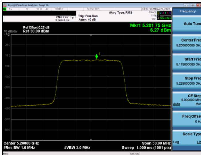
Plot 7-363. PSD SDM Antenna WF8 (20MHz BW 802.11ax(SU) – Ch. 40, MCS3)
