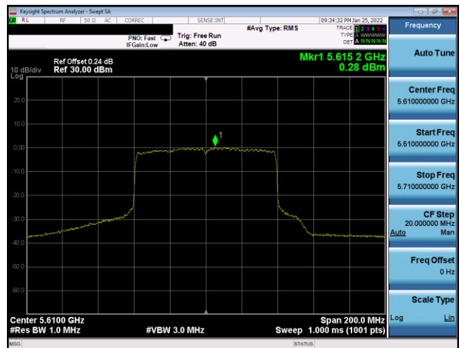
Plot 7-359. PSD CDD Antenna WF8 (80MHz BW 802.11ax(SU) – Ch. 122, MCS0)
