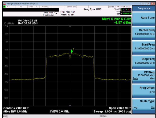
Plot 7-382. PSD CDD Antenna WF7a (80MHz BW 802.11ac – Ch. 58, MCS3)
