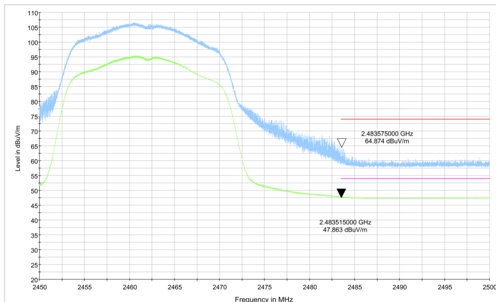
Fig.A.6.2.2 Transmitter Spurious Emission - Radiated (Power): 802.11n-HT20, ch11, 2.45 GHz - 2.50GHz
