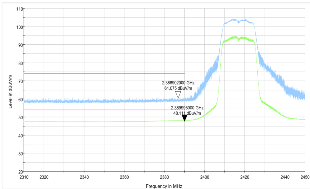
Fig.A.6.2.5 Transmitter Spurious Emission - Radiated (Power): 802.11g, ch1, 2.31 GHz - 2.45GHz
