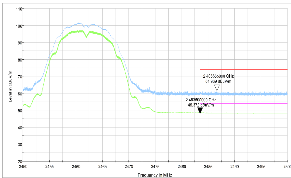
Fig.A.6.2.4 Transmitter Spurious Emission - Radiated (Power): 802.11b, ch11, 2.45 GHz - 2.50GHz
