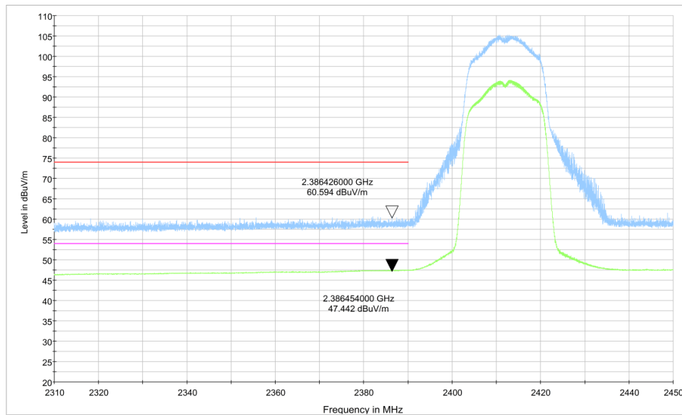
Fig.A.6.2.1 Transmitter Spurious Emission - Radiated (Power): 802.11n-HT20, ch1, 2.31 GHz - 2.45GHz
