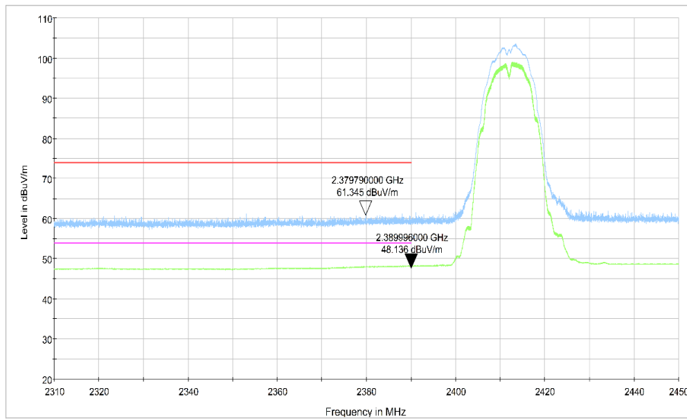
Fig.A.6.2.3 Transmitter Spurious Emission - Radiated (Power): 802.11b, ch1, 2.31 GHz – 2.45GHz
