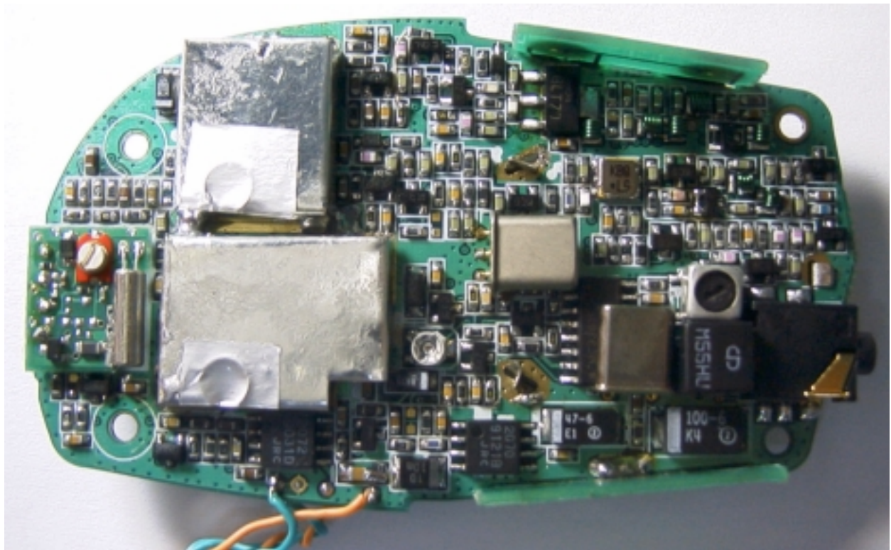
PCB w/Shield
