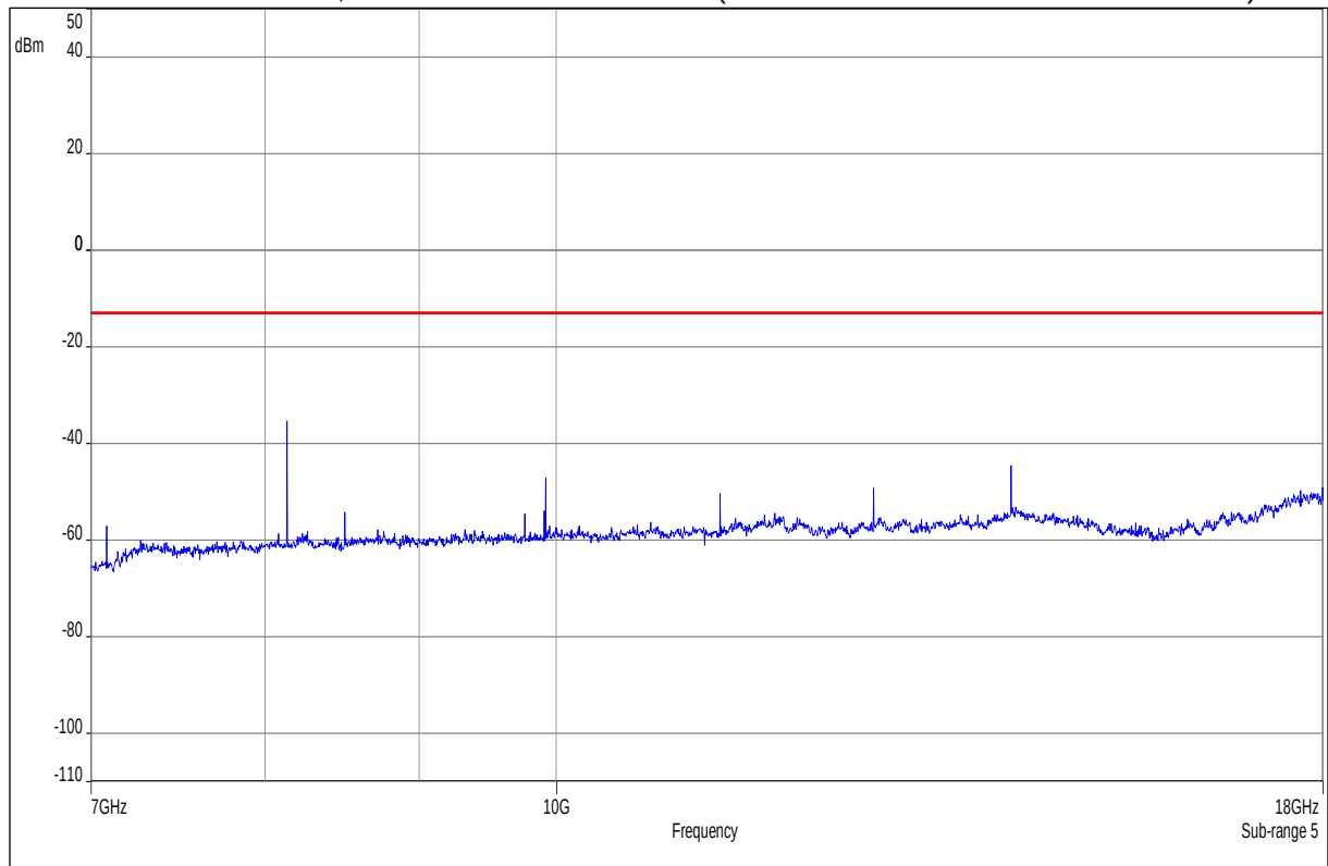
Plot No. 143: 7 GHz – 18 GHz, antenna vertical / horizontal (valid for all channels and all modulations)
