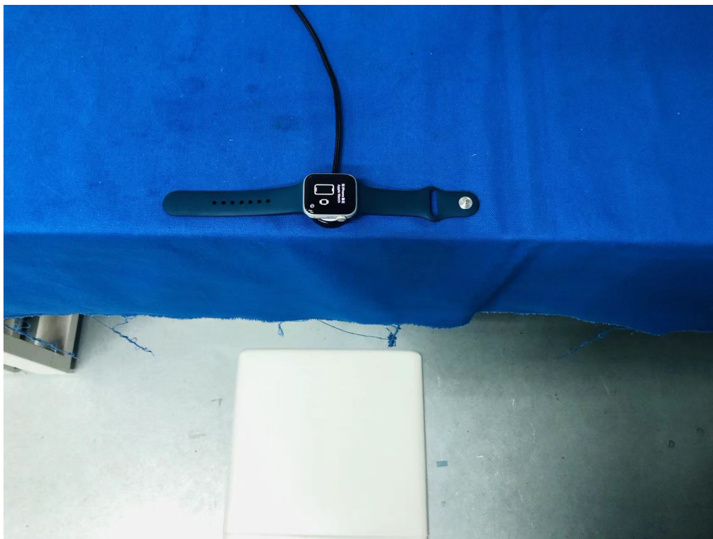
Photograph 4: Set-up for RF Exposure
