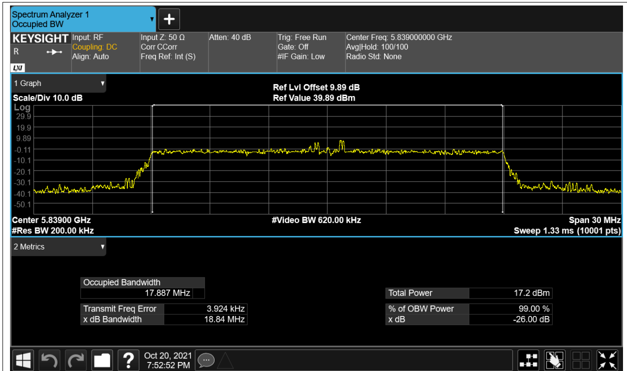
OBW HVHT 5.8G-20M-16QAM 5839MHz Ant2
