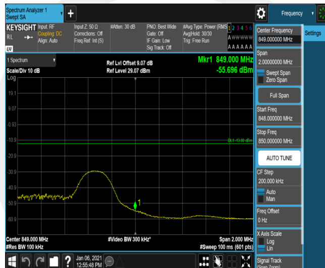
Band5-5MHz-QPSK-20625-1RB#24
