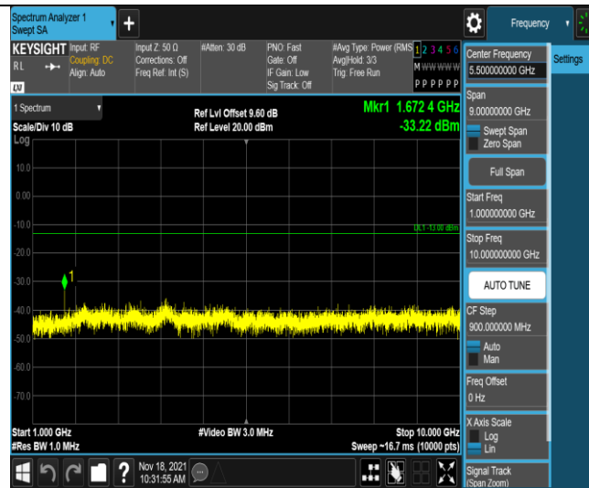
Band5-1.4MHz-QPSK-20525-1RB#0-Range2:1000~10000MHz
