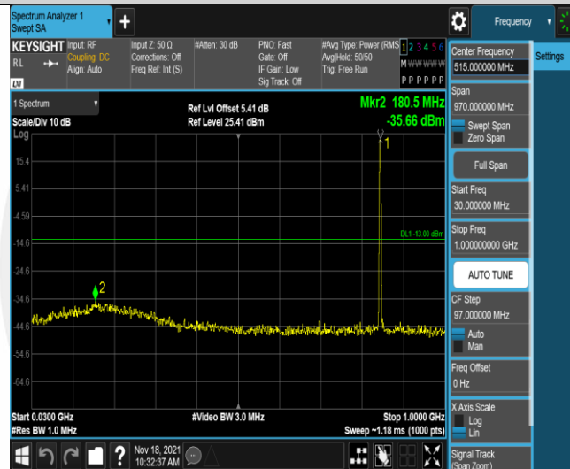
Band5-1.4MHz-QPSK-20643-1RB#0-Range1:30~1000MHz
