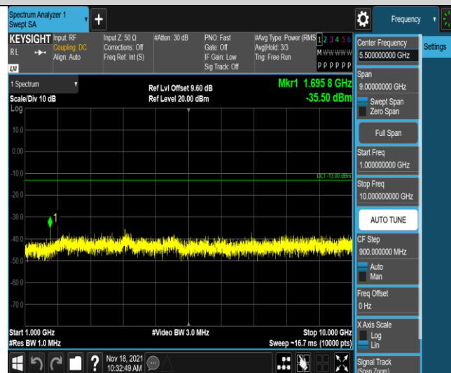
Band5-1.4MHz-QPSK-20643-1RB#0-Range2:1000~10000MHz
