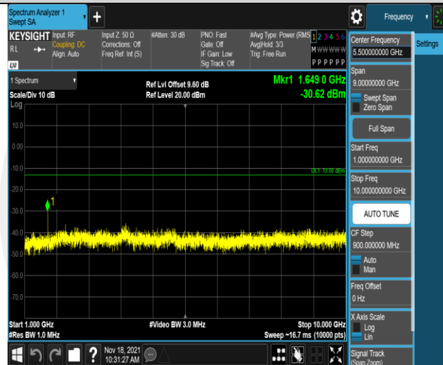
Band5-1.4MHz-16QAM-20407-1RB#0-Range2:1000~10000MHz
