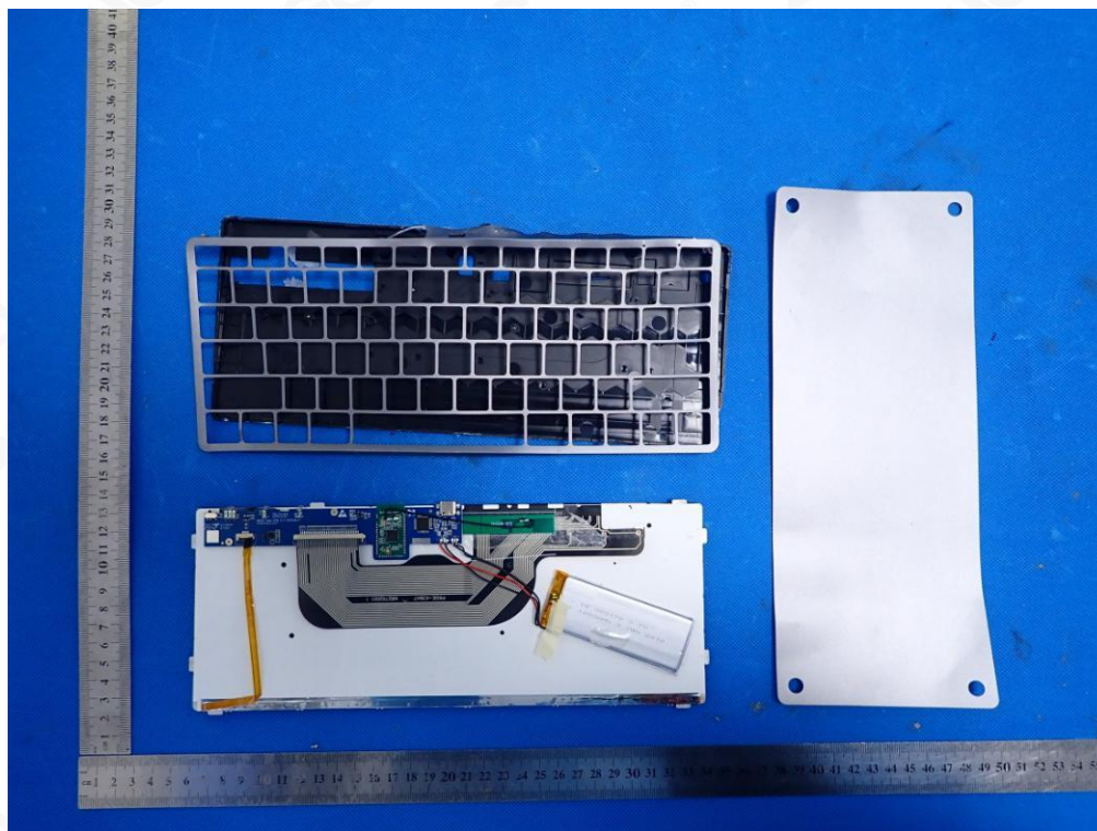
INTERNAL VIEW-1 OF EUT(ST-BTSX1)
