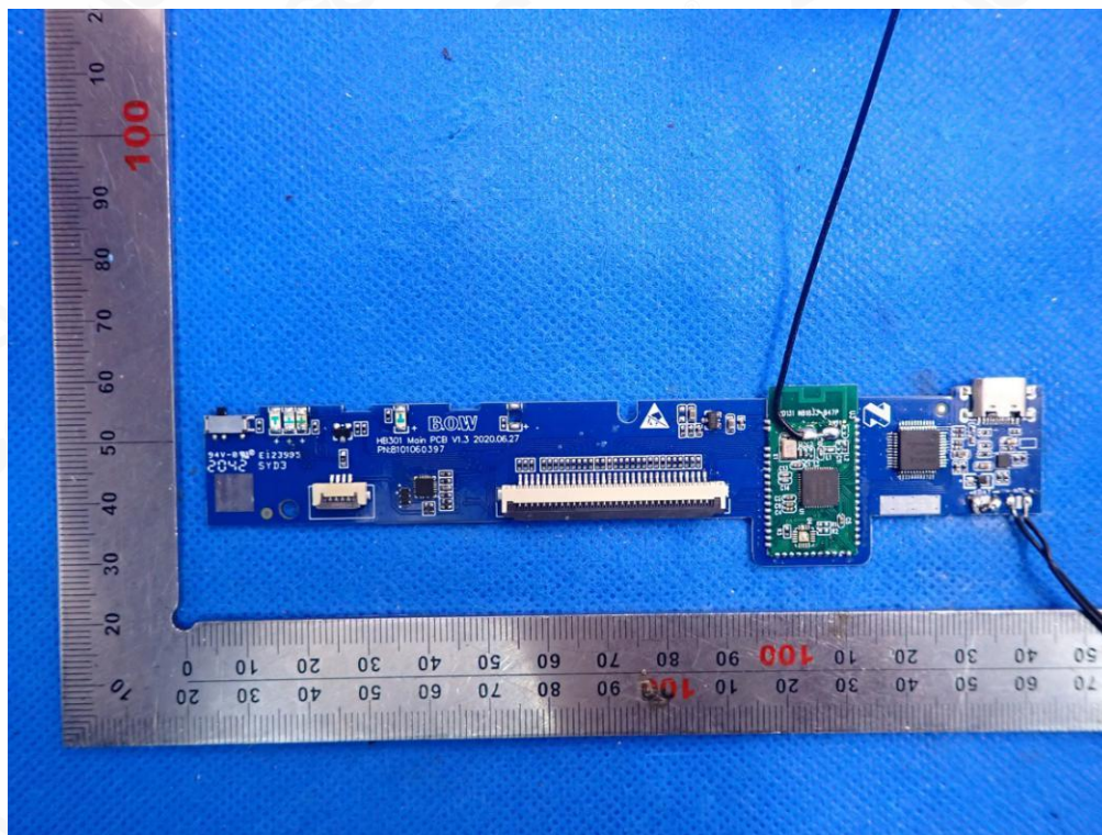
INTERNAL VIEW-3 OF EUT(ST-BTSX1)
