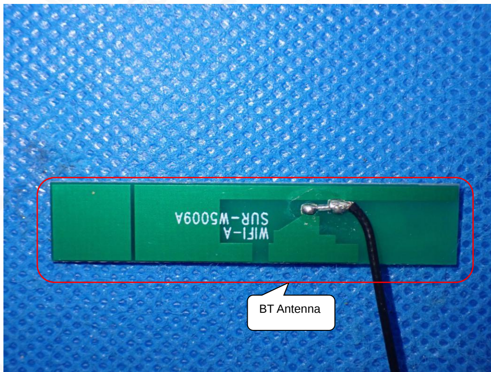
INTERNAL VIEW-7 OF EUT(ST-BTSX2)
