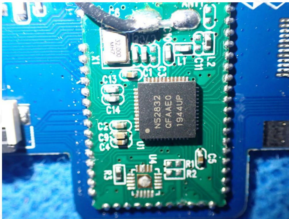
INTERNAL VIEW-5 OF EUT(ST-BTSX1)
