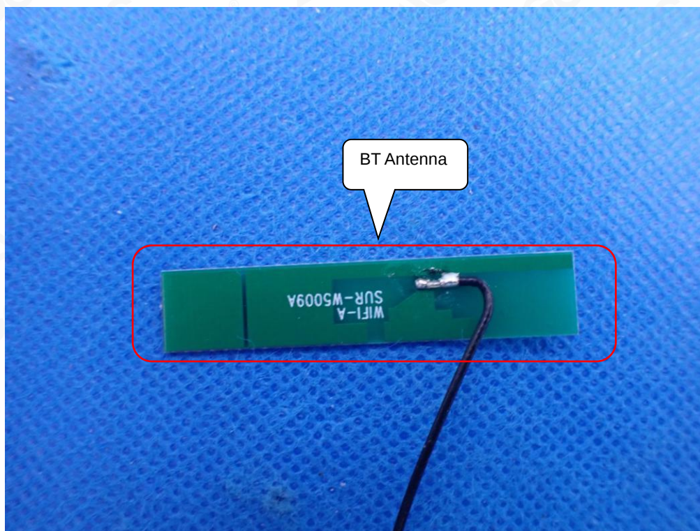
INTERNAL VIEW-7 OF EUT(ST-BTSX1)
