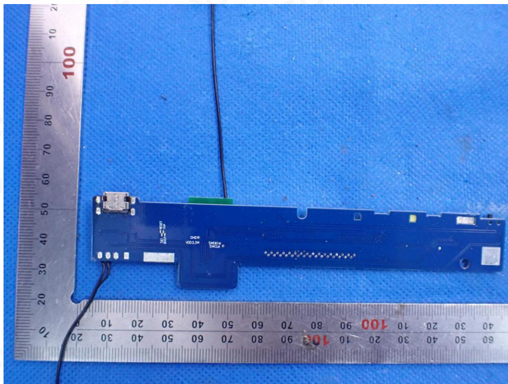
INTERNAL VIEW-5 OF EUT(ST-BTSX3)
