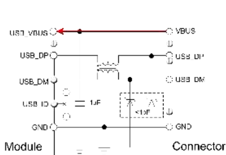
Figure 13: USB reference circuit
