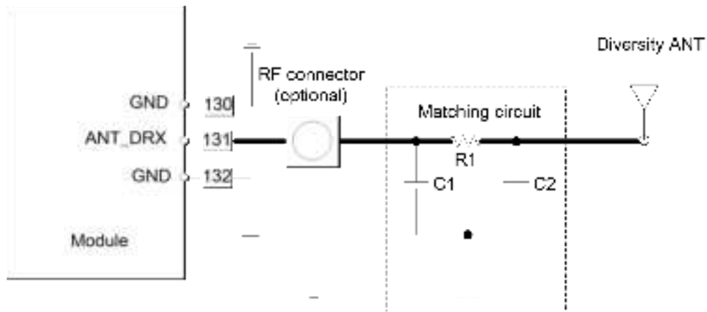
Figure 27: DRX antenna recommended circuit
