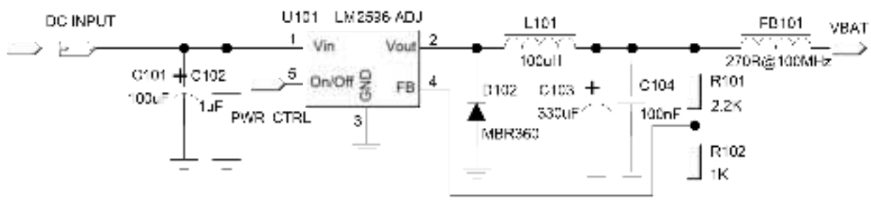
Figure 5: DC-DC power supply reference circuit
