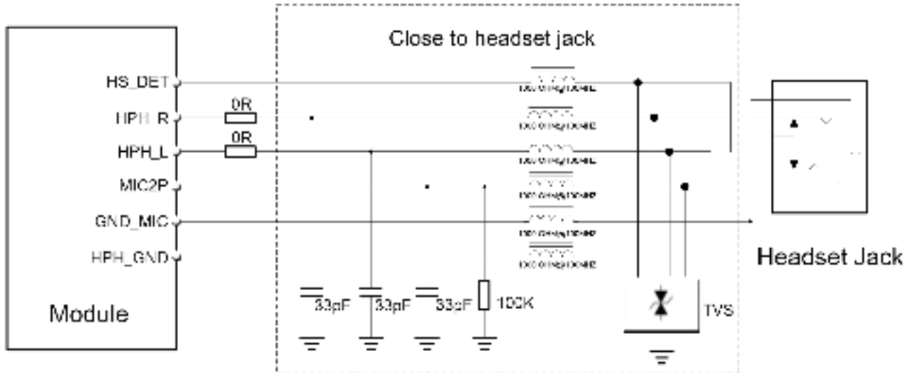
Figure 21: Headset reference circuit
