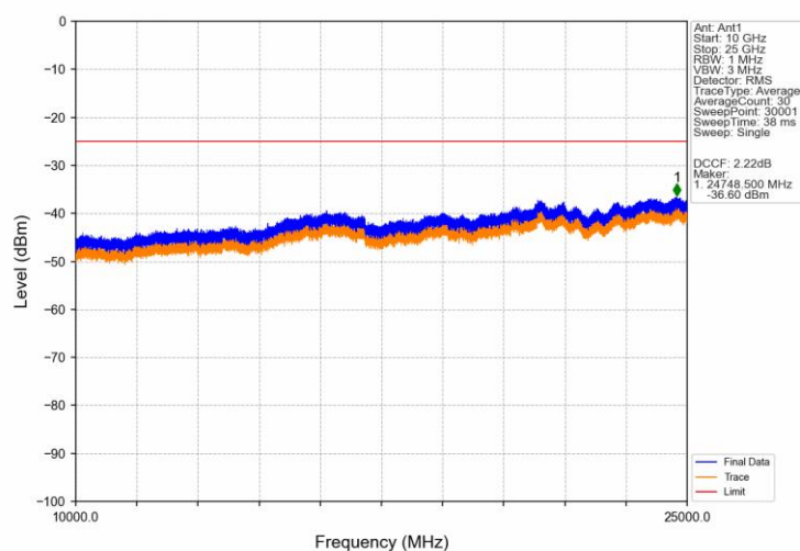
Band41 20MHz 16QAM MCH 2593MHz RB 1 0 NTV
