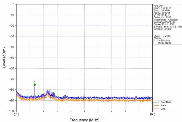
Band41_15MHz_16QAM_LCH_2503.5MHz_RB_1_0_NTNV
