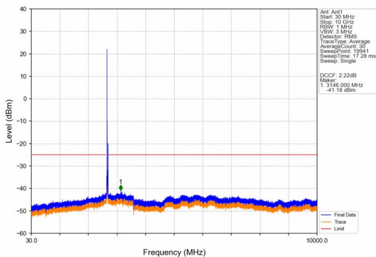
Band41 20MHz 16QAM HCH 2680MHz RB 1 0 NTV
