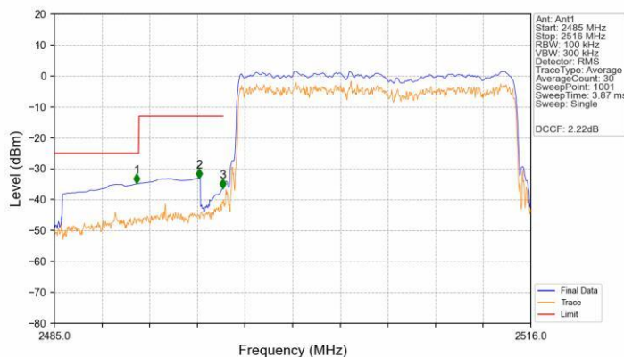
Band41_20MHz_16QAM_LCH_2506MHz_RB_100_0_NTNV
