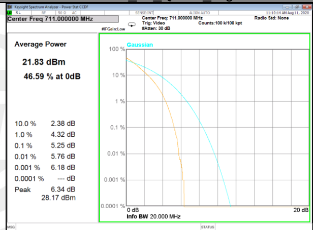
Band12_50_Q16_High
