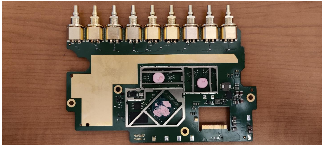
PCB 1 (WiFi board) – Top (identifying antennas)
