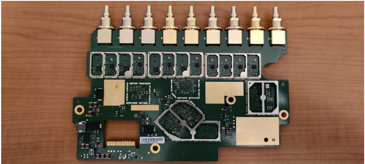
PCB 1 (WiFi board – Bottom (identifying antennas)
