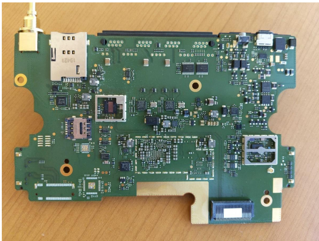
PCB 2 (Main board) – Bottom
