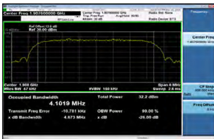
HSDPA_B2_HighCH9538-1907.6
