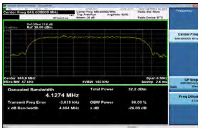
HSDPA_B5_HighCH4233-846.6
