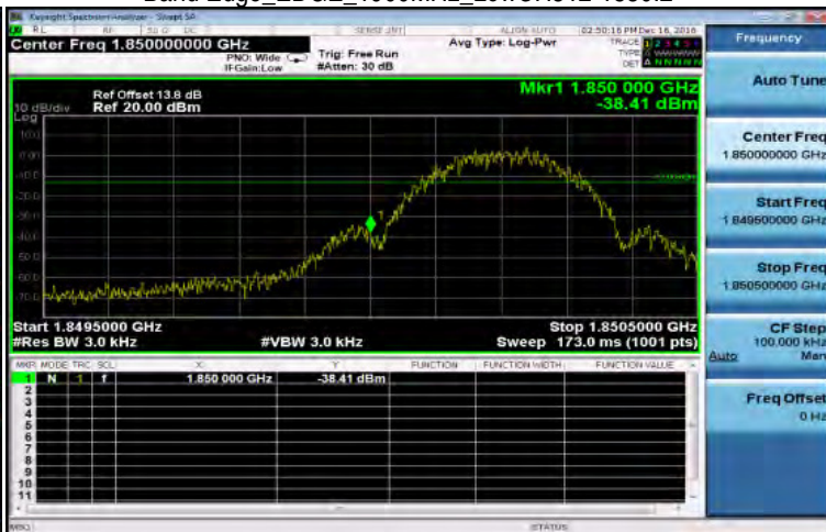
Band Edge_EDGE_1900MHz_LowCH512-1850.2
