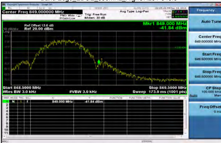
Band Edge_EDGE_850MHz_HighCH251-848.8
