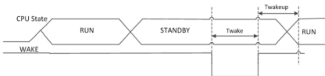
Figure 8-3 Wake Timing
