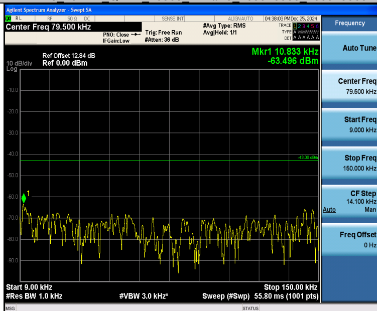
Band25 10MHz 16QAM 26365 1RB#49 0.009~0.15 0.009~0.15
