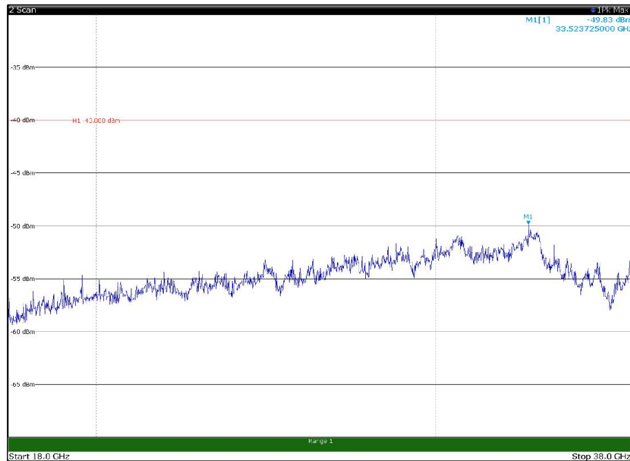
Channel: BOTTOM, Modulation: 16QAM, BW=5MHz, Range: 18GHz - 38GHz, Polarization: Vertical
