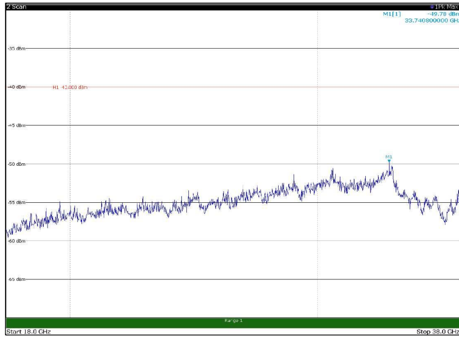
Channel: BOTTOM, Modulation: 16QAM, BW=5MHz, Range: 18GHz - 38GHz, Polarization: Horizontal
