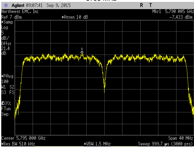
Chain A, 802.11(ac) MCS9 (256-QAM), 40 MHz, High Channel 5795 MHz
