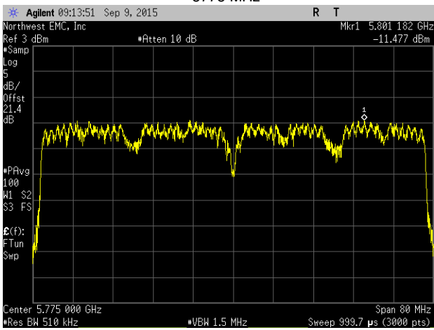
Chain A, 802.11(ac) MCS9 (256-QAM), 80 MHz, Low Channel 5775 MHz
