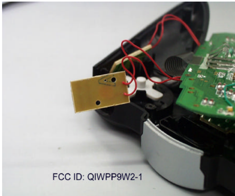
Switch PCB Photo 4
