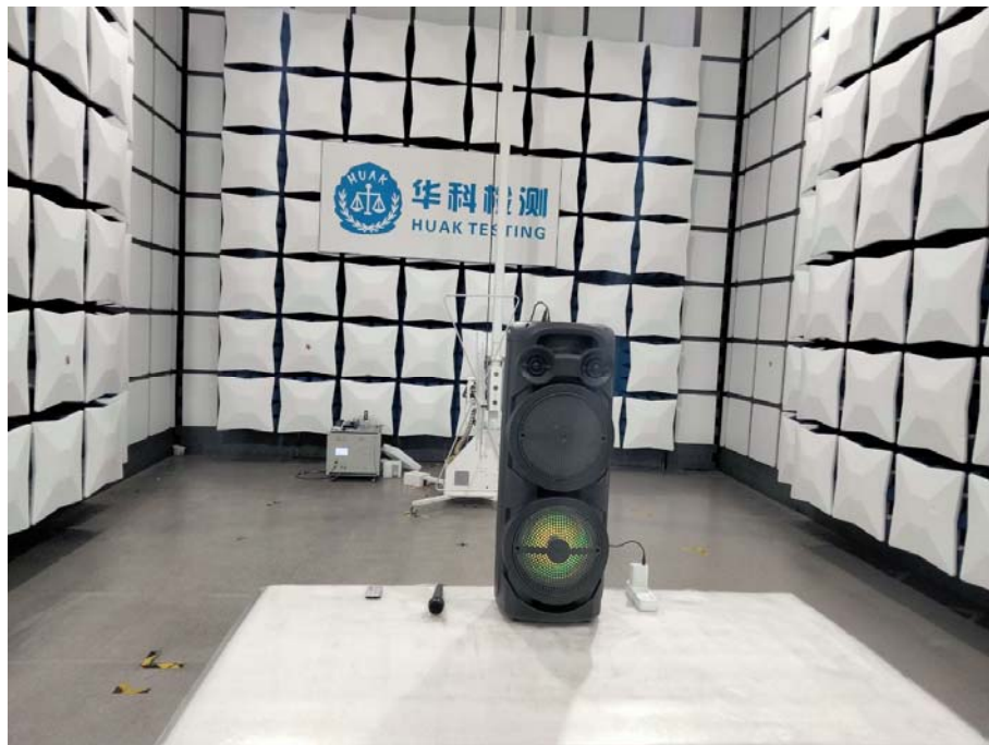
Model: YS-BS0466 Radiated Emissions
