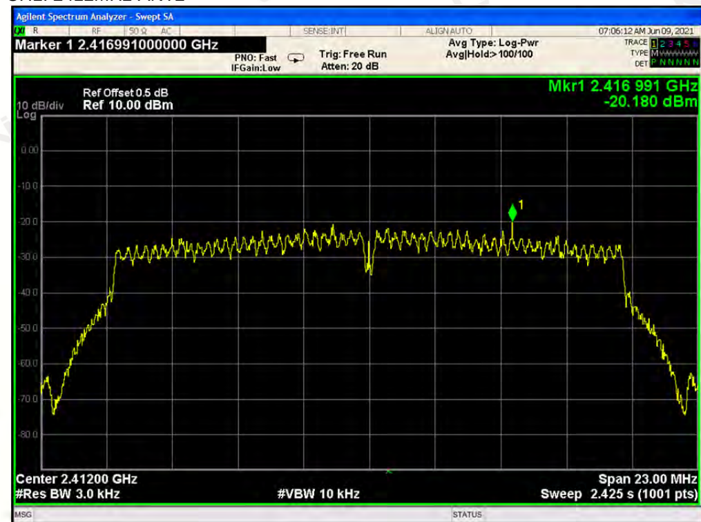
CH11: 2412MHz-ANT2
