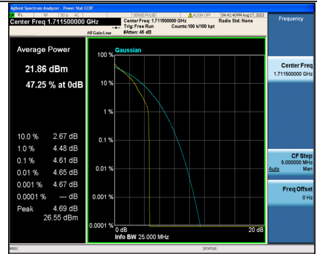
Band4-3MHz-QPSK-19965-1RB#0-PASS
