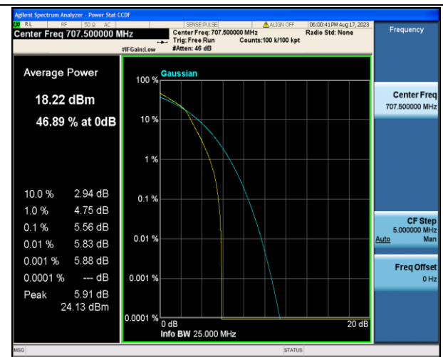
Band12-1.4MHz-16QAM-23095-6RB#0-PASS
