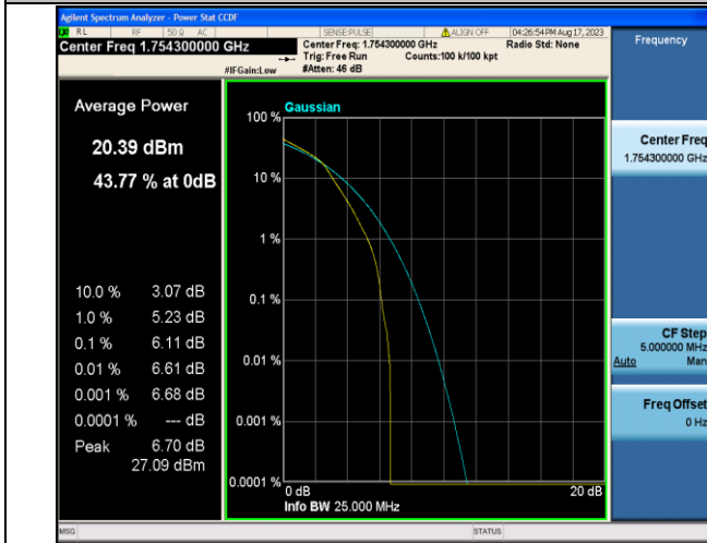
Band4-1.4MHz-16QAM-20393-6RB#0-PASS
