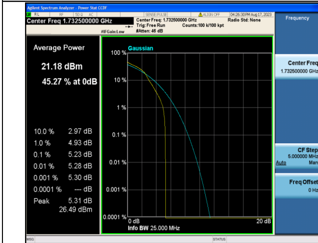
Band4-1.4MHz-16QAM-20175-1RB#0-PASS
