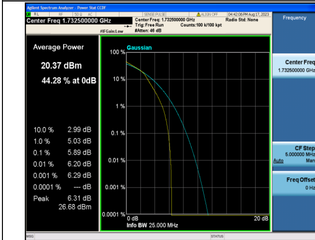
Band4-3MHz-16QAM-20175-15RB#0-PASS
