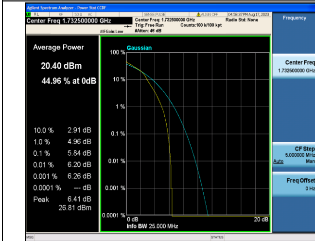
Band4-5MHz-16QAM-20175-25RB#0-PASS
