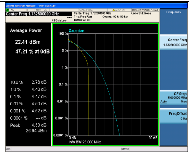
Band4-5MHz-QPSK-20175-1RB#0-PASS
