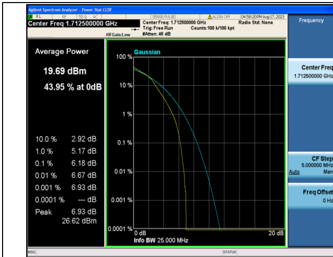
Band4-5MHz-16QAM-19975-25RB#0-PASS
