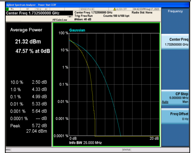
Band4-3MHz-QPSK-20175-15RB#0-PASS
