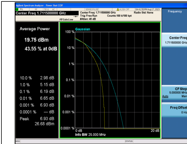
Band4-3MHz-16QAM-19965-15RB#0-PASS
