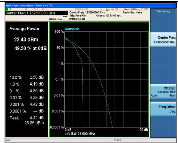
Band4-3MHz-QPSK-20175-1RB#0-PASS
