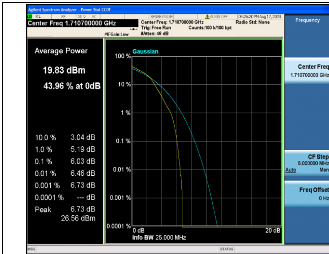
Band4-1.4MHz-16QAM-19957-6RB#0-PASS
