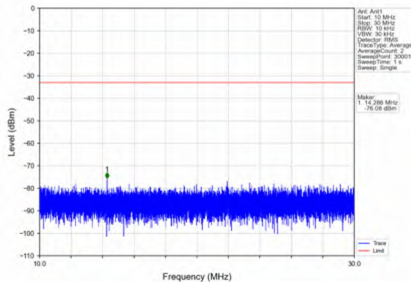
n7_15kHz_SISO_NTNV_15MHz_DFT-s-OFDM QPSK_2507.5MHz_Outer_Full
