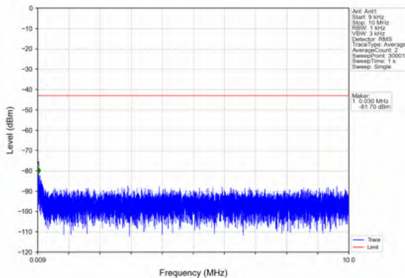
n7_15kHz_SISO_NTNV_10MHz_CP-OFDM QPSK_2505MHz_Edge_1RB_Left
