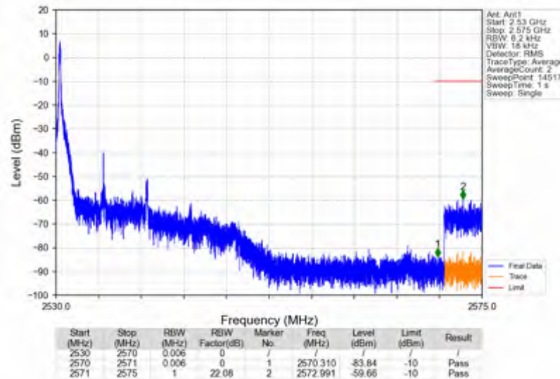
n7_15kHz_SISO_NTNV_10MHz_DFT-s-OFDM QPSK_2535MHz_Edge_1RB_Left
