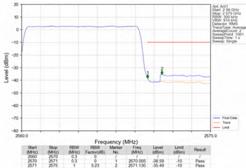
n7_15kHz_SISO_NTNV_10MHz_DFT-s-OFDM_QPSK_2565MHz_Outer_Full
