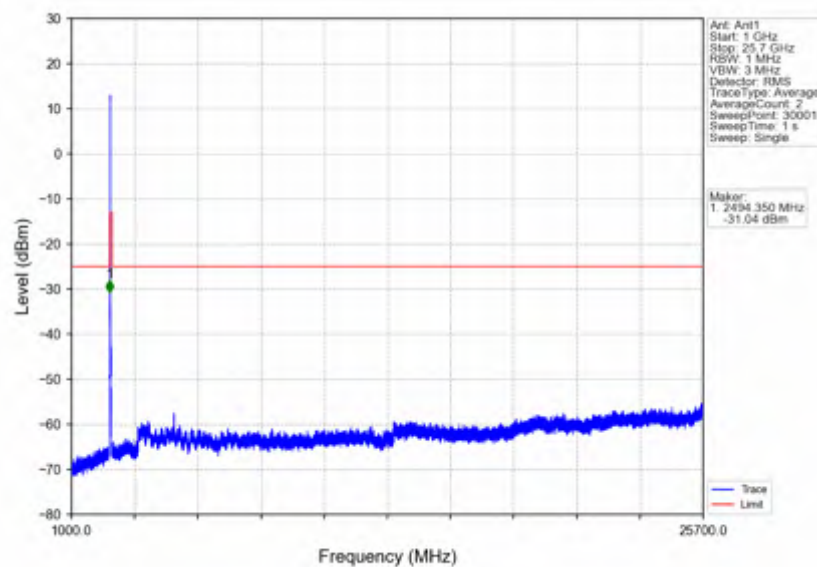
n7 15kHz SISO NTNV 15MHz DFT-s-OFDM PI/2 BPSK 2507.5MHz Outer Full
