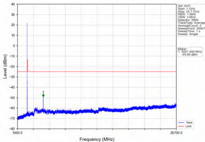
n7_15kHz_SISO_NTNV_10MHz_DFT-s-OFDM_PI/2_BPSK_2535MHz_Edge_1RB_Left
