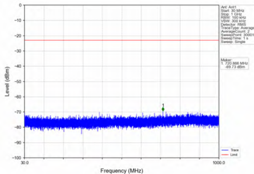
n7 15kHz SISO NTV 10MHz CP-OFDM QPSK 2565MHz Outer Full
