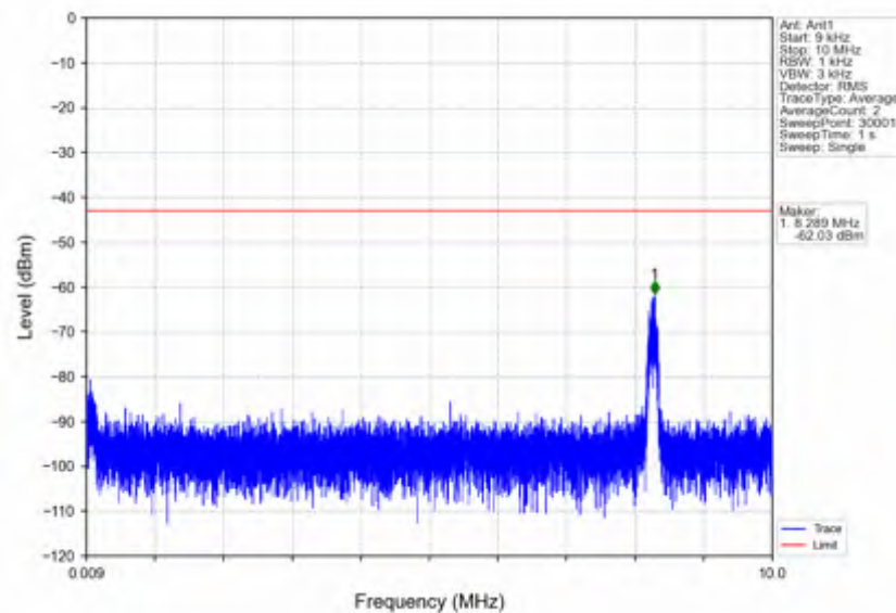
n7_15kHz_SISO_NTV_15MHz_DFT-s-OFDM QPSK_2562.5MHz_Edge_1RB_Right
