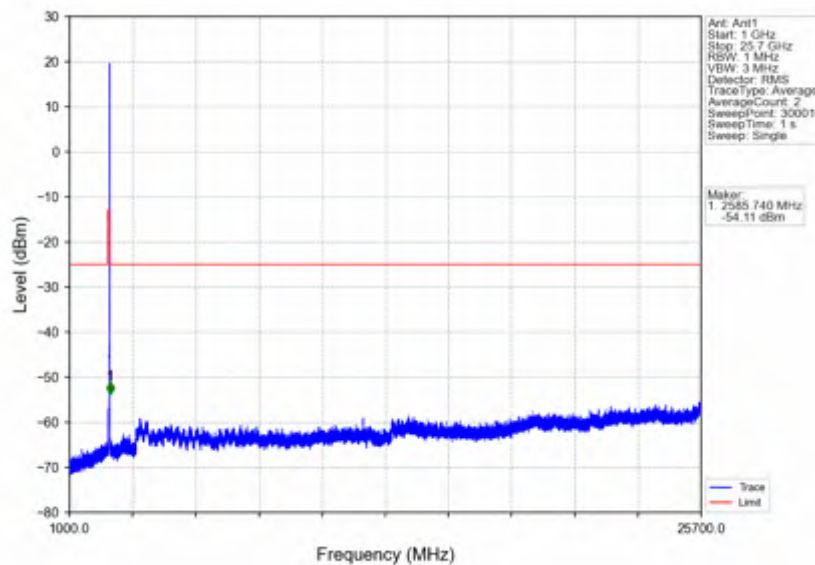
n7_15kHz_SISO_NTNV_15MHz_CP-OFDM QPSK_2562.5MHz_Outer_Full
