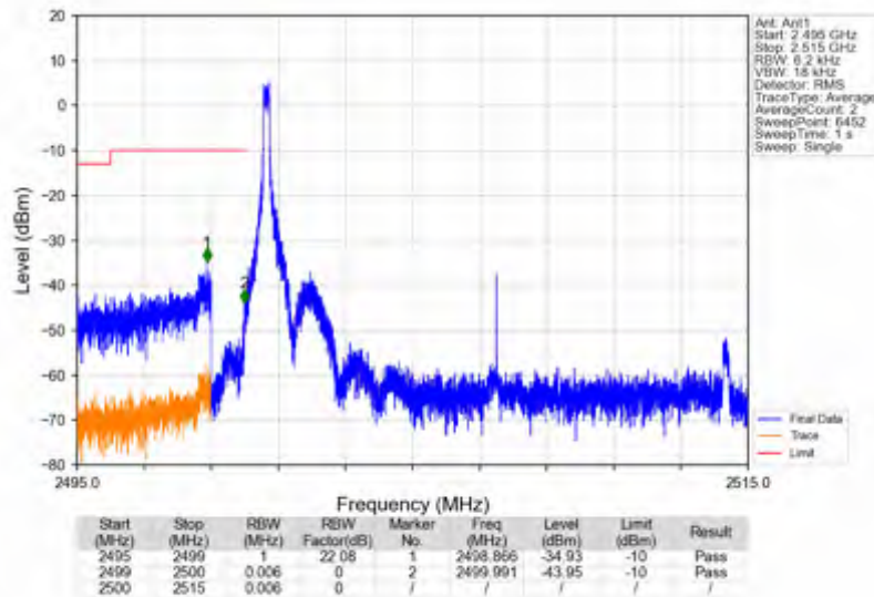
n7_15kHz_SISO_NTNV_15MHz_CP-OFDM_QPSK_2507.5MHz_Inner_1RB_Left
