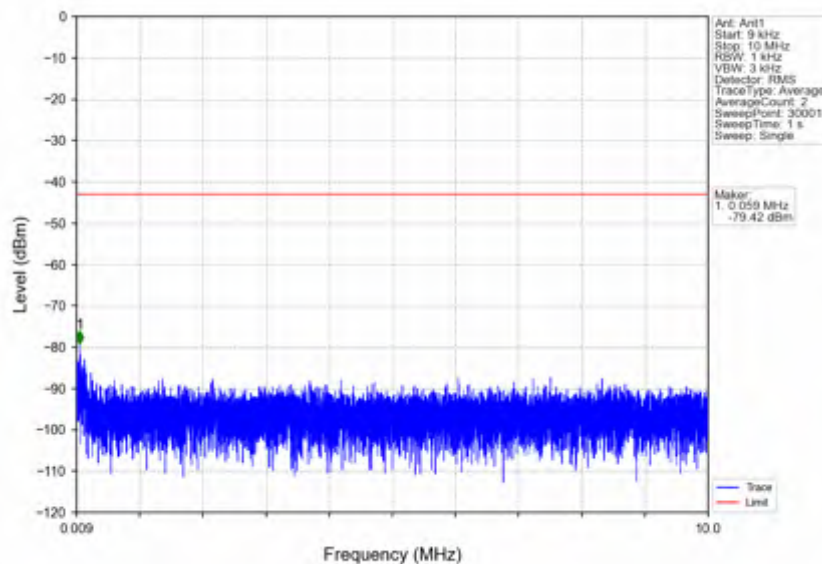
n7_15kHz_SISO_NTNV_15MHz_DFT-s-OFDM_PI/2_BPSK_2507.5MHz_Edge_1RB_Left
