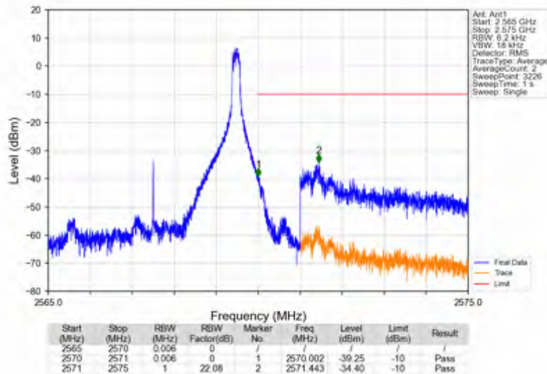
n7_15kHz_SISO_NTNV_5MHz_DFT-s-OFDM QPSK_2567.5MHz_Inner_1RB_Right
