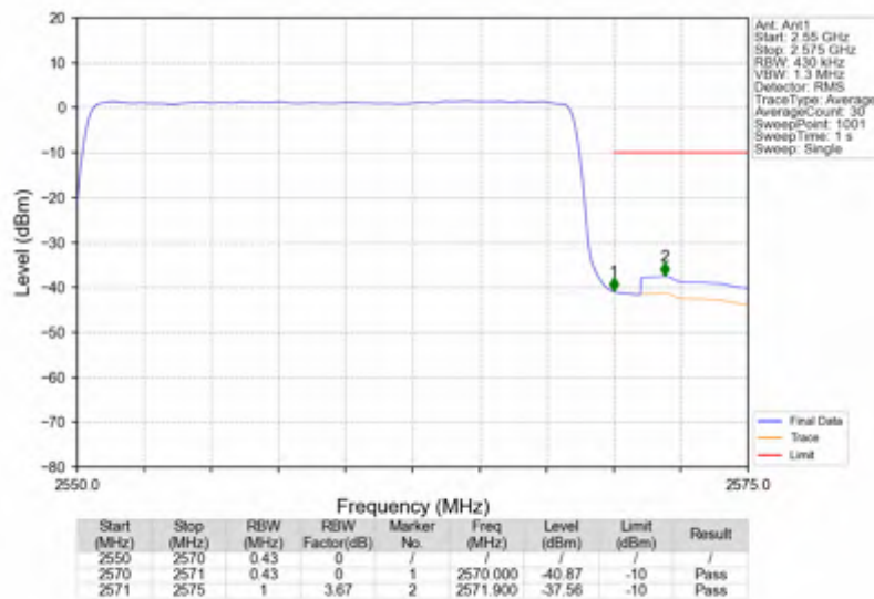
n7_15kHz_SISO_NTNV_20MHz_DFT-s-OFDM_QPSK_2560MHz_Outer_Full
