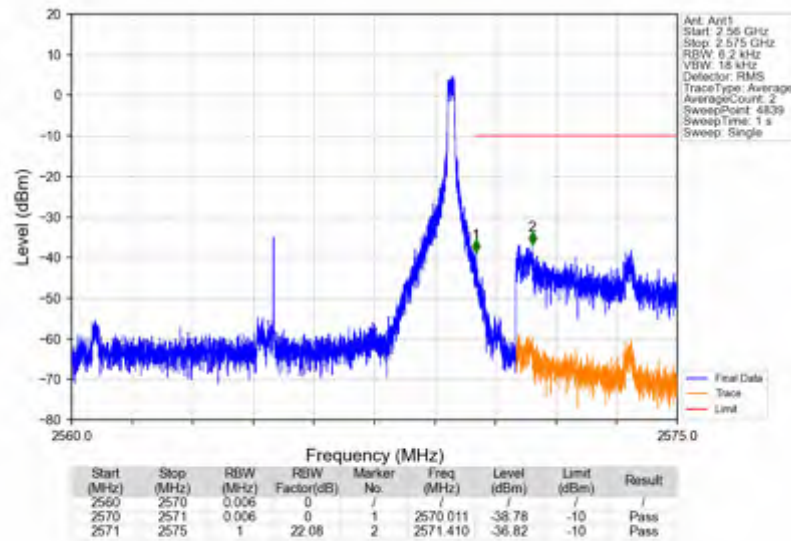
n7_15kHz_SISO_NTNV_10MHz_CP-OFDM_QPSK_2565MHz_Inner_1RB_Right
