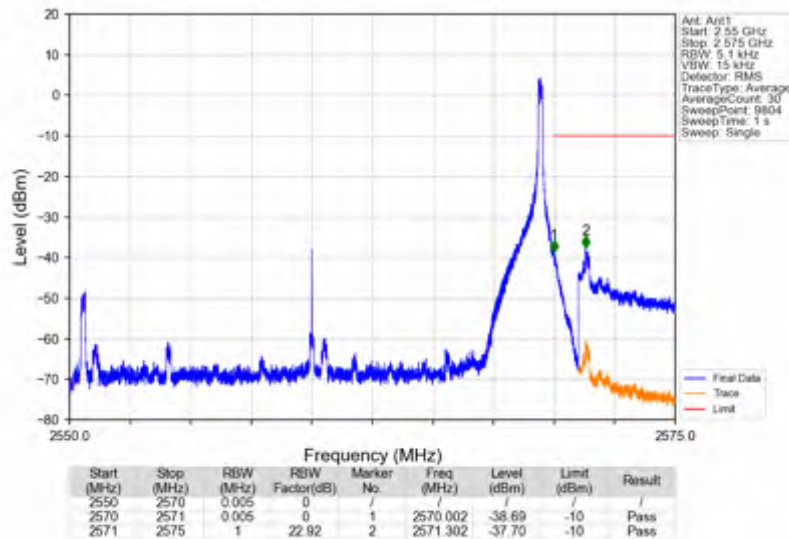
n7_15kHz_SISO_NTNV_20MHz_DFT-s-OFDM QPSK_2560MHz_Edge_1RB_Right
