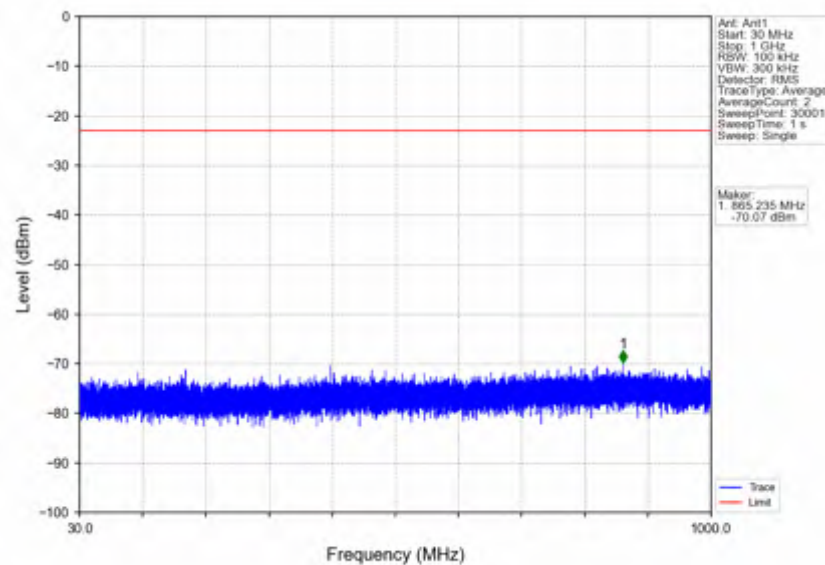
n7_15kHz_SISO_NTNV_20MHz_CP-OFDM_QPSK_2510MHz_Outer_Full
