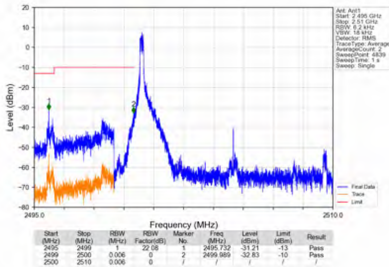
n7_15kHz_SISO_NTNV_10MHz_DFT-s-OFDM_PI/2_BPSK_2505MHz_Edge_1RB_Left
