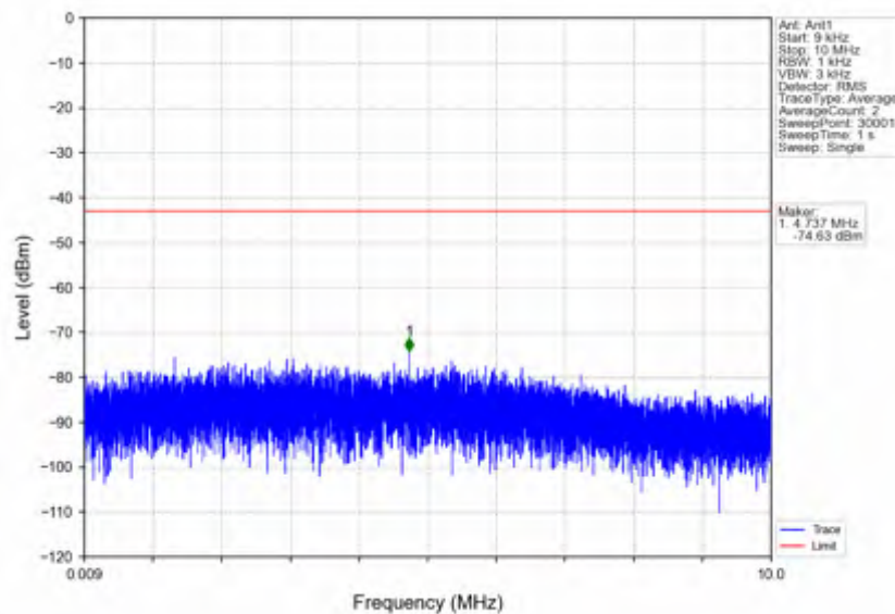
n7_15kHz_SISO_NTNV_10MHz_DFT-s-OFDM_QPSK_2565MHz_Outer_Full
