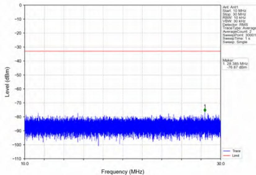
n7_15kHz_SISO_NTNV_10MHz_DFT-s-OFDM_QPSK_2565MHz_Inner_1RB_Right
