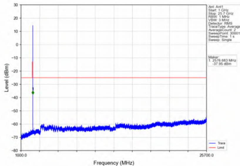
n7_15kHz_SISO_NTNV_5MHz_CP-OFDM_QPSK_2567.5MHz_Outer_Full
