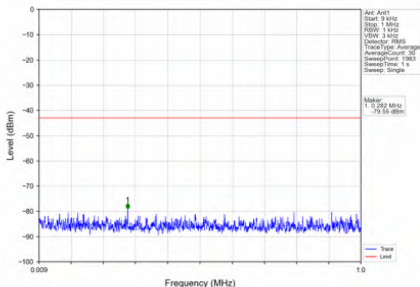
n7_15kHz_SISO_NTNV_20MHz_DFT-s-OFDM_QPSK_2560MHz_Outer_Full
