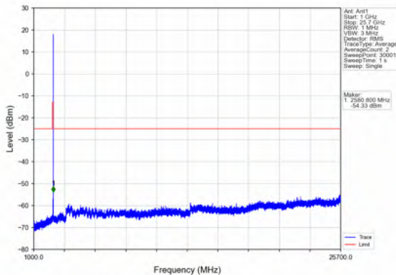
n7_15kHz_SISO_NTNV_10MHz_CP-OFDM QPSK_2565MHz_Outer_Full
