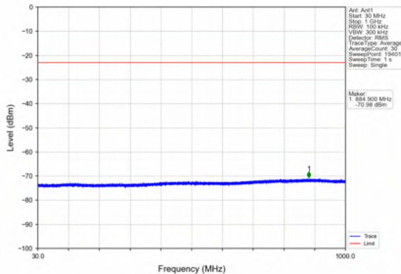
n7_15kHz_SISO_NTNV_20MHz_DFT-s-OFDM_QPSK_2560MHz_Inner_1RB_Right
