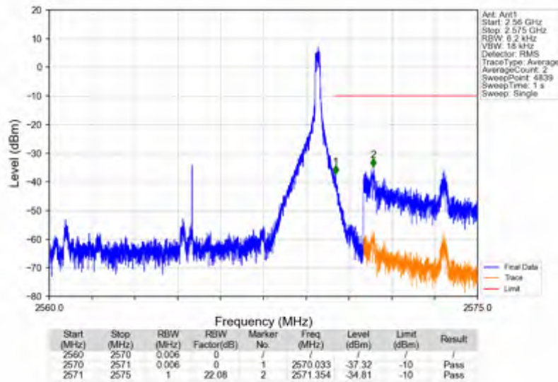
n7_15kHz_SISO_NTNV_10MHz_DFT-s-OFDM QPSK_2565MHz_Inner_1RB_Right
