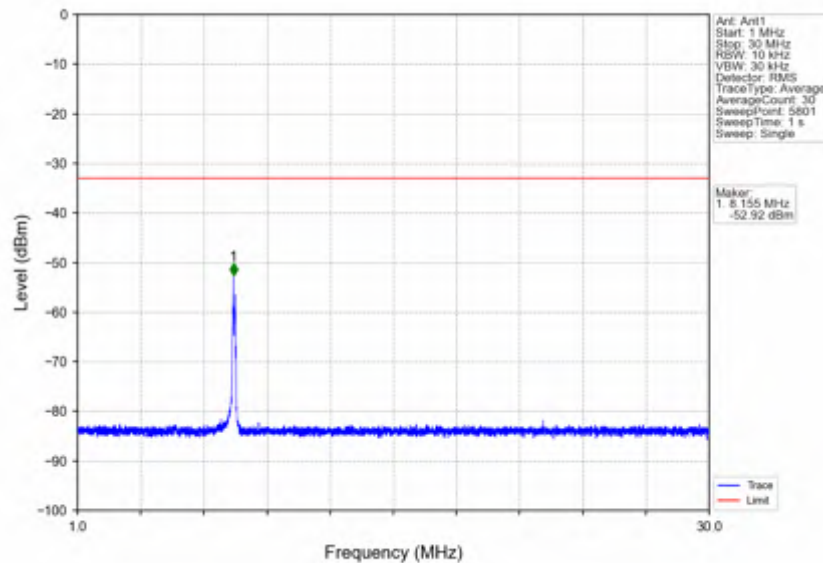
n7_15kHz_SISO_NTNV_20MHz_DFT-s-OFDM PI/2 BPSK_2560MHz_Edge_1RB_Right
