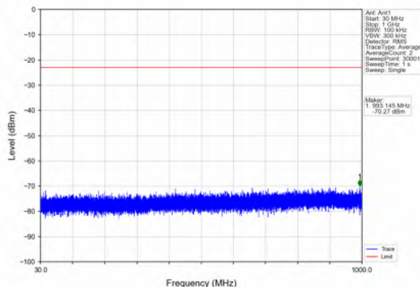
n7_15kHz_SISO_NTNV_15MHz_DFT-s-OFDM QPSK_2535MHz_Edge_1RB_Left
