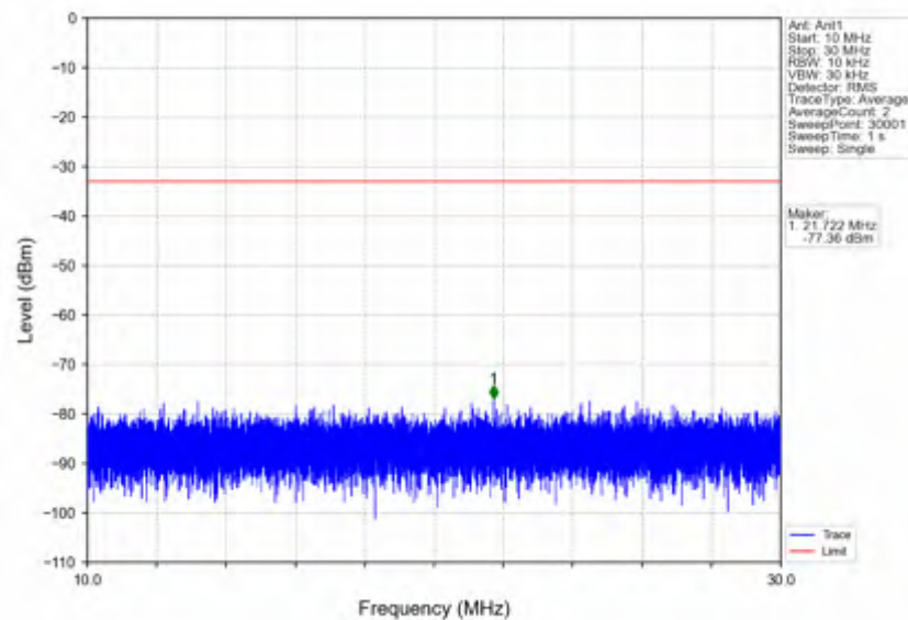
n7_15kHz_SISO_NTNV_5MHz_CP-OFDM_QPSK_2567.5MHz_Outer_Full
