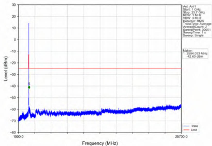
n7 15kHz SISO NTNV 10MHz DFT-s-OFDM PI/2 BPSK 2565MHz Outer Full
