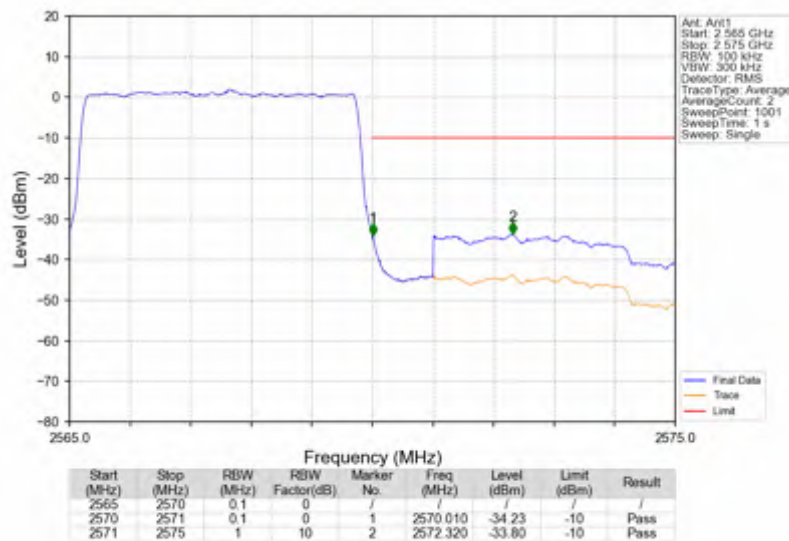
n7_15kHz_SISO_NTNV_5MHz_DFT-s-OFDM_QPSK_2567.5MHz_Outer_Full
