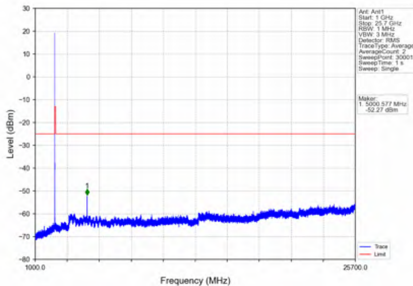
n7_15kHz_SISO_NTNV_5MHz_CP-OFDM QPSK_2502.5MHz_Outer_Full
