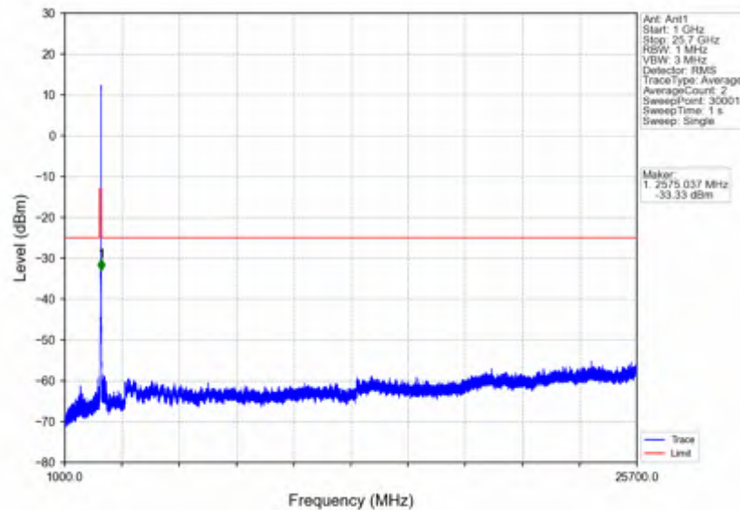
n7_15kHz_SISO_NTNV_15MHz_DFT-s-OFDM_PI/2_BPSK_2562.5MHz_Outer_Full
