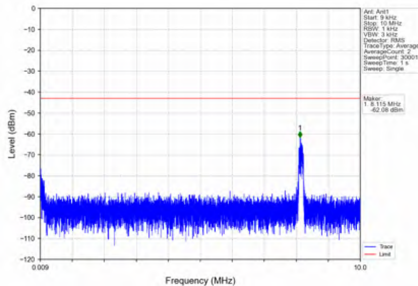
n7_15kHz_SISO_NTNV_10MHz_CP-OFDM_QPSK_2565MHz_Inner_1RB_Right
