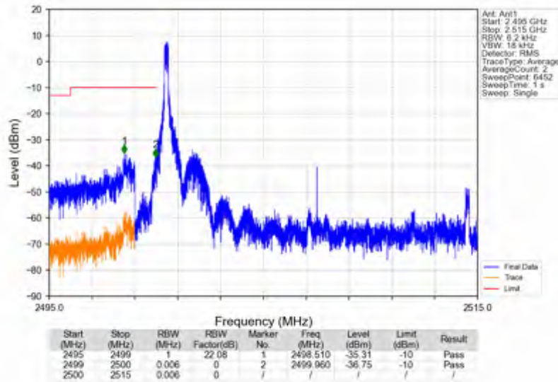
n7_15kHz_SISO_NTNV_15MHz_DFT-s-OFDM_PI/2_BPSK_2507.5MHz_Edge_1RB_Left
