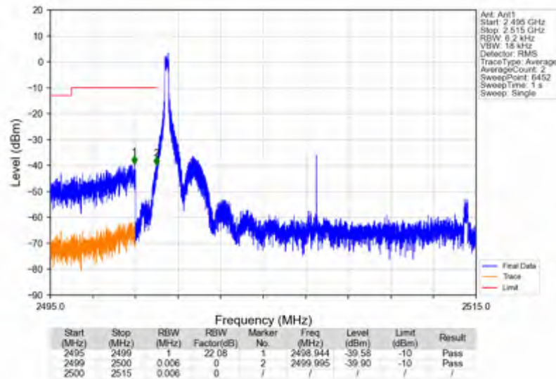
n7_15kHz_SISO_NTNV_15MHz_CP-OFDM_QPSK_2507.5MHz_Edge_1RB_Left
