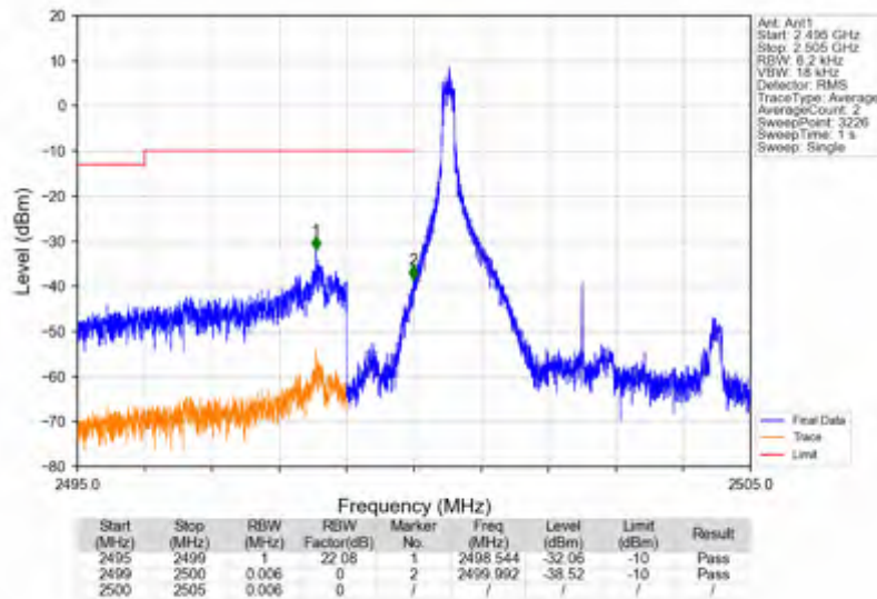
n7_15kHz_SISO_NTNV_5MHz_DFT-s-OFDM QPSK_2502.5MHz_Inner_1RB_Left
