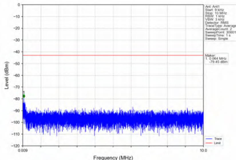
n7_15kHz_SISO_NTNV_10MHz_DFT-s-OFDM QPSK_2535MHz_Edge_1RB_Left
