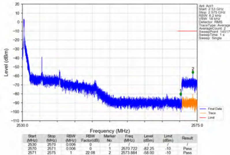
n7_15kHz_SISO_NTNV_10MHz_CP-OFDM QPSK_2535MHz_Edge_1RB_Left
