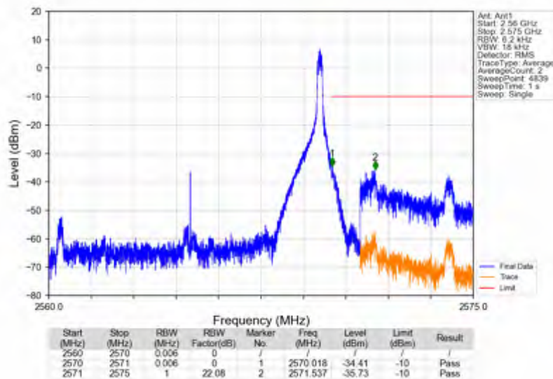
n7_15kHz_SISO_NTNV_10MHz_DFT-s-OFDM QPSK_2565MHz_Edge_1RB_Right
