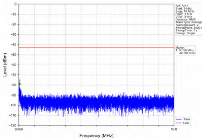
n7_15kHz_SISO_NTNV_10MHz_DFT-s-OFDM_PI/2_BPSK_2505MHz_Edge_1RB_Left
