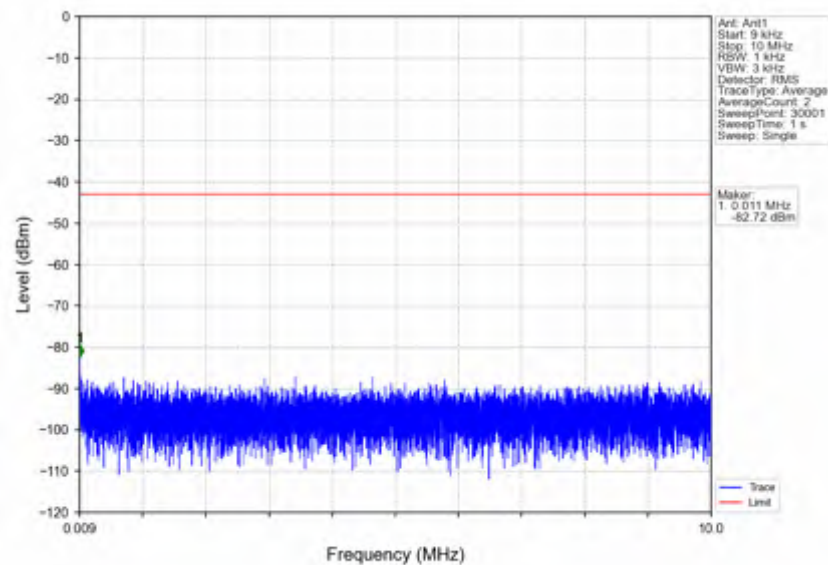
n7_15kHz_SISO_NTNV_15MHz_DFT-s-OFDM_PI/2_BPSK_2507.5MHz_Outer_Full
