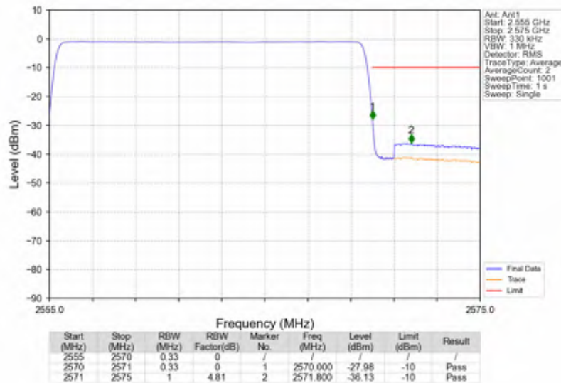
n7_15kHz_SISO_NTNV_15MHz_CP-OFDM QPSK_2562.5MHz_Outer_Full
