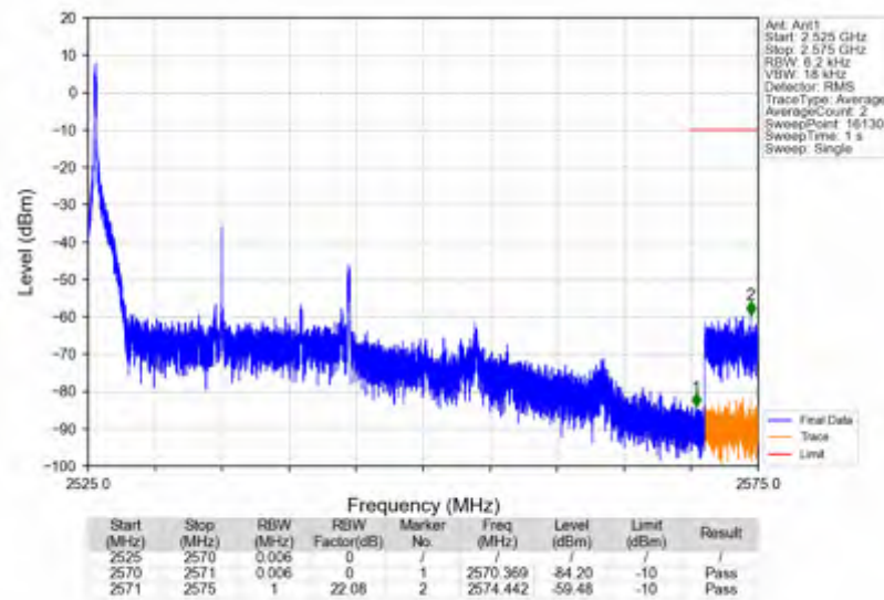
n7_15kHz_SISO_NTNV_20MHz_DFT-s-OFDM_QPSK_2535MHz_Edge_1RB_Left
