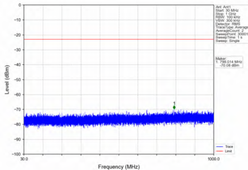
n7_15kHz_SISO_NTNV_5MHz_CP-OFDM_QPSK_2567.5MHz_Outer_Full
