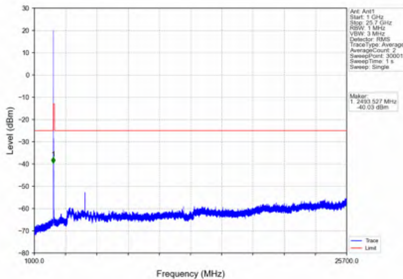
n7_15kHz_SISO_NTNV_15MHz_CP-OFDM QPSK_2535MHz_Edge_1RB_Left
