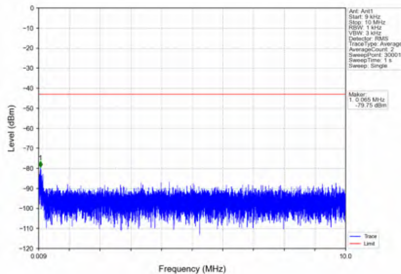
n7_15kHz_SISO_NTNV_5MHz_DFT-s-OFDM_QPSK_2535MHz_Edge_1RB_Left
