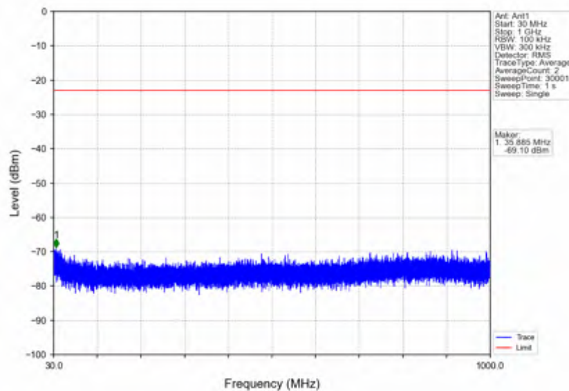
n7_15kHz_SISO_NTNV_15MHz_CP-OFDM QPSK_2562.5MHz_Outer_Full
