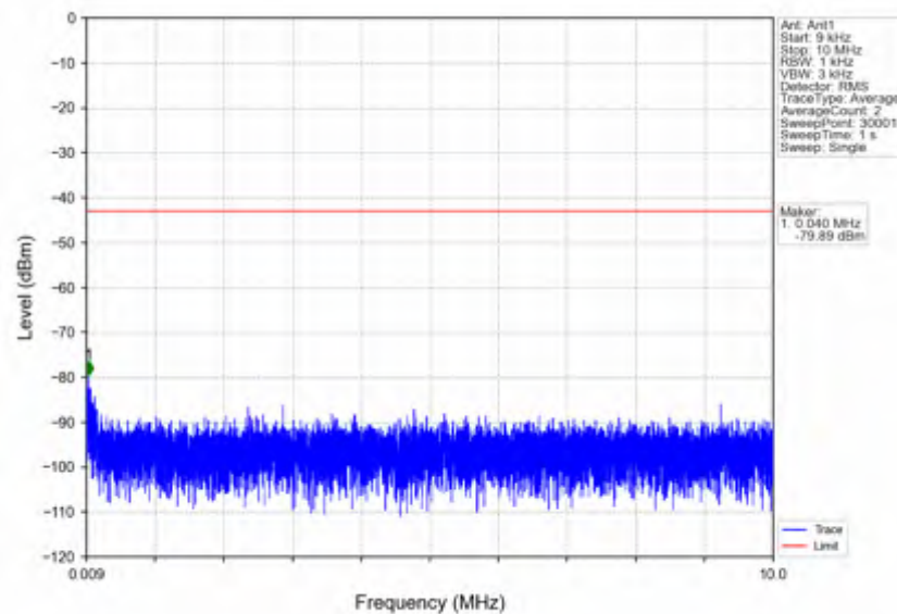
n7_15kHz_SISO_NTNV_15MHz_CP-OFDM QPSK_2535MHz_Edge_1RB_Left
