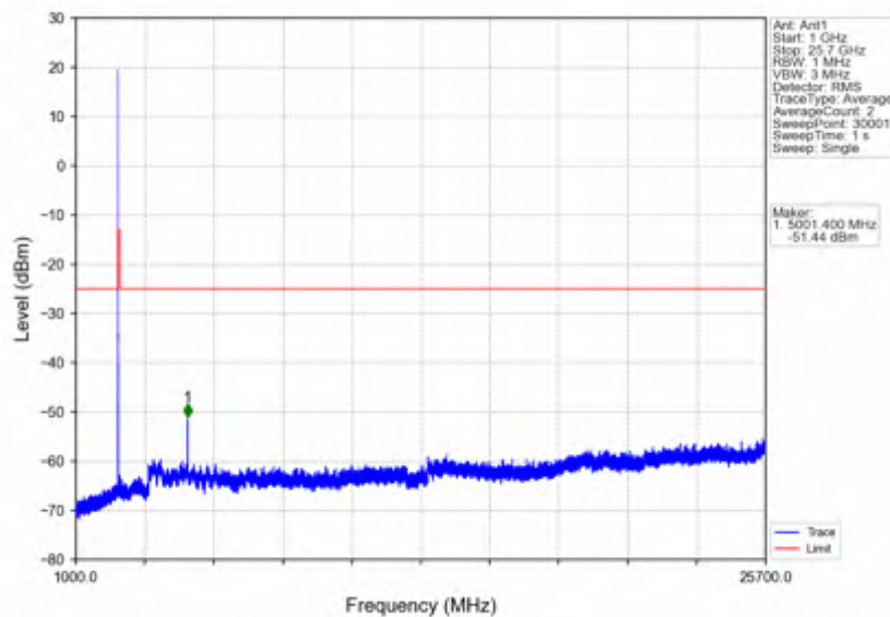
n7_15kHz_SISO_NTNV_10MHz_CP-OFDM QPSK_2535MHz_Edge_1RB_Left
