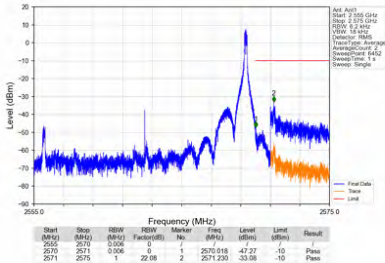
n7_15kHz_SISO_NTNV_15MHz_DFT-s-OFDM_PI/2_BPSK_2562.5MHz_Inner_1RB_Right
