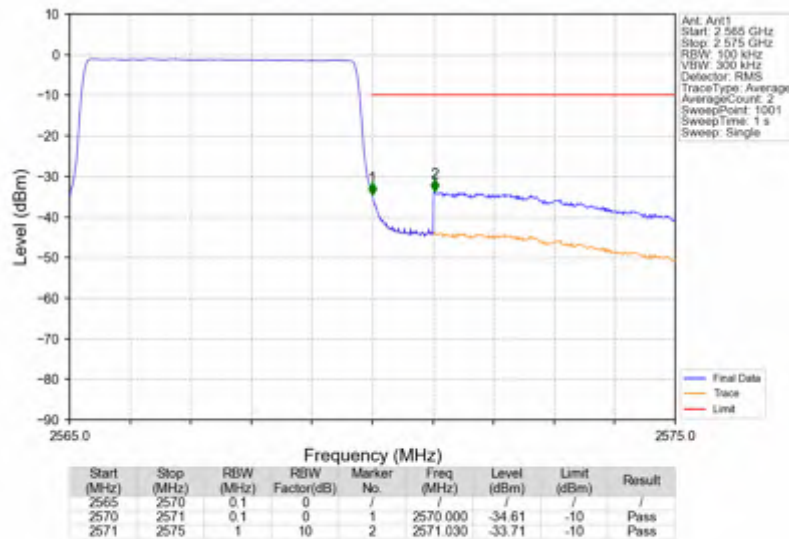
n7_15kHz_SISO_NTNV_5MHz_CP-OFDM_QPSK_2567.5MHz_Outer_Full
