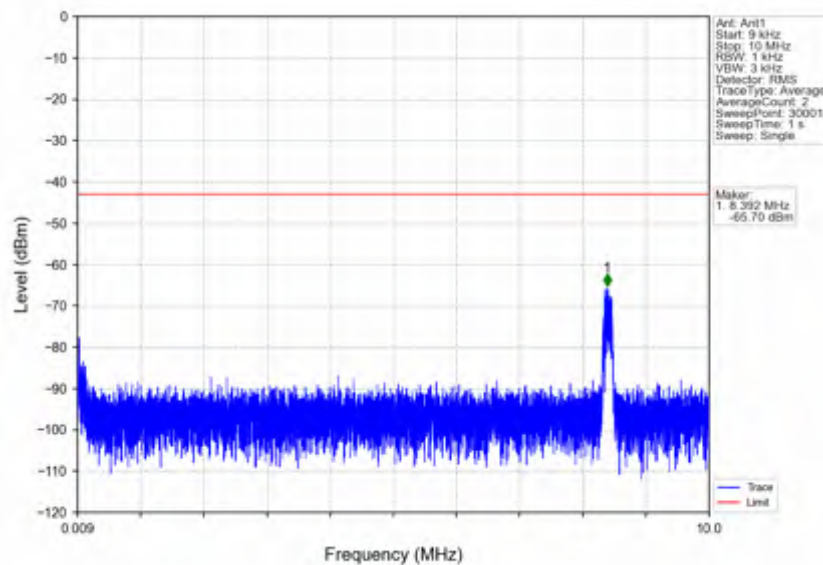
n7_15kHz_SISO_NTNV_5MHz_CP-OFDM_QPSK_2567.5MHz_Edge_1RB_Right
