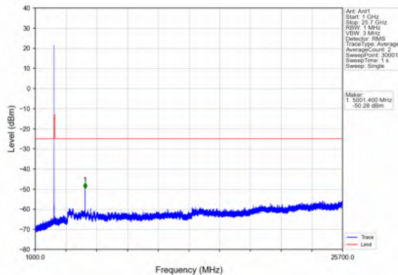
n7_15kHz_SISO_NTNV_5MHz_DFT-s-OFDM_QPSK_2502.5MHz_Inner_1RB_Left
