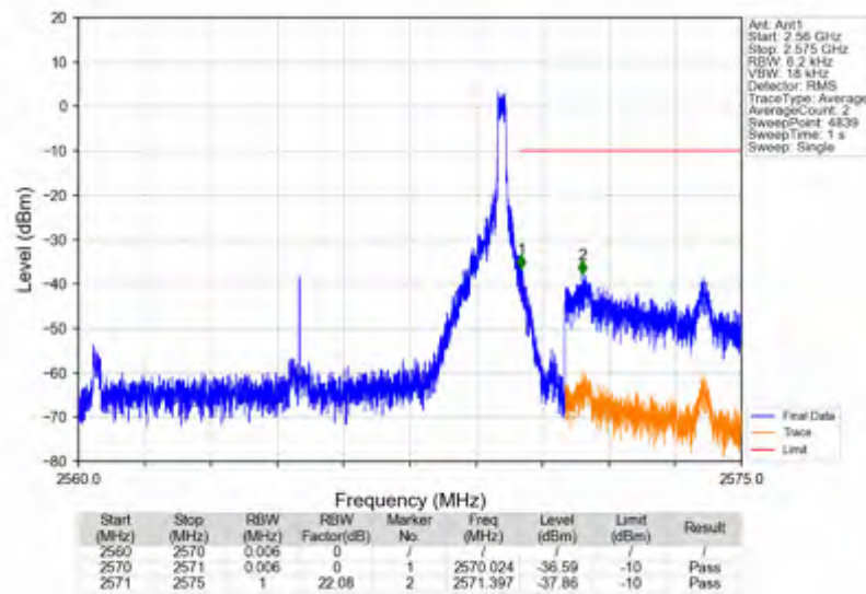
n7_15kHz_SISO_NTNV_10MHz_CP-OFDM_QPSK_2565MHz_Edge_1RB_Right
