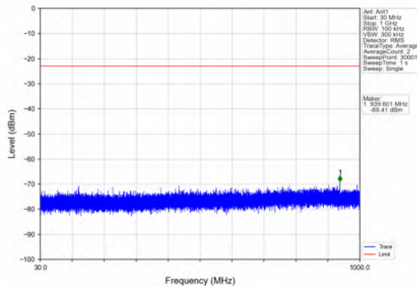
n7_15kHz_SISO_NTNV_5MHz_CP-OFDM QPSK_2502.5MHz_Edge_1RB_Left
