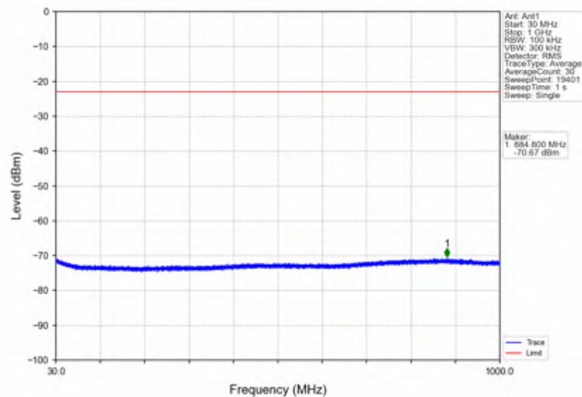
n7 15kHz SISO NTNV 20MHz DFT-s-OFDM PI/2 BPSK 2560MHz Outer Full
