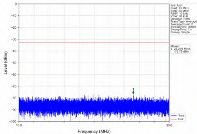
n7_15kHz_SISO_NTNV_10MHz_DFT-s-OFDM_QPSK_2565MHz_Edge_1RB_Right
