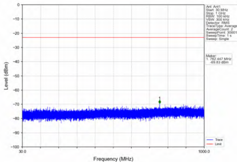
n7_15kHz_SISO_NTNV_10MHz_DFT-s-OFDM PI/2 BPSK_2505MHz_Edge_1RB_Left
