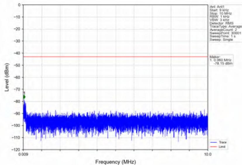
n7_15kHz_SISO_NTNV_5MHz_DFT-s-OFDM QPSK_2502.5MHz_Inner_1RB_Left
