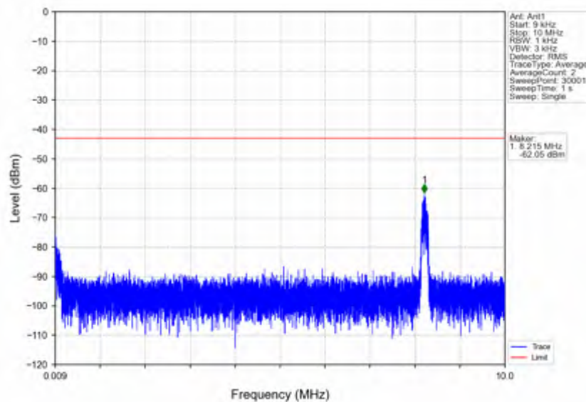
n7_15kHz_SISO_NTNV_5MHz_CP-OFDM_QPSK_2567.5MHz_Inner_1RB_Right
