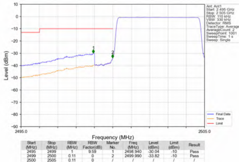
n7_15kHz_SISO_NTNV_5MHz_CP-OFDM QPSK_2502.5MHz_Outer_Full
