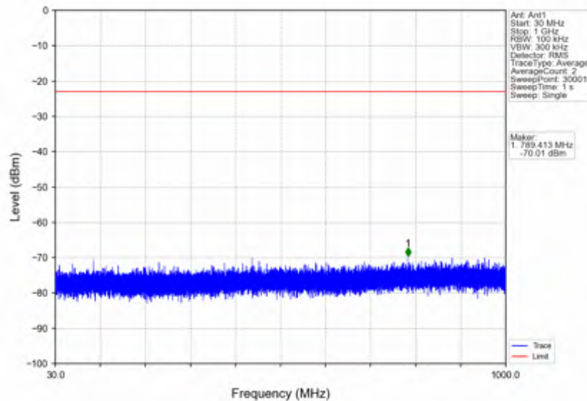
n7_15kHz_SISO_NTNV_15MHz_DFT-s-OFDM PI/2 BPSK_2535MHz_Edge_1RB_Left
