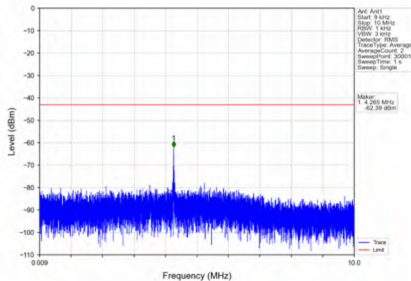
n7_15kHz_SISO_NTNV_15MHz_DFT-s-OFDM_PI/2_BPSK_2562.5MHz_Outer_Full
