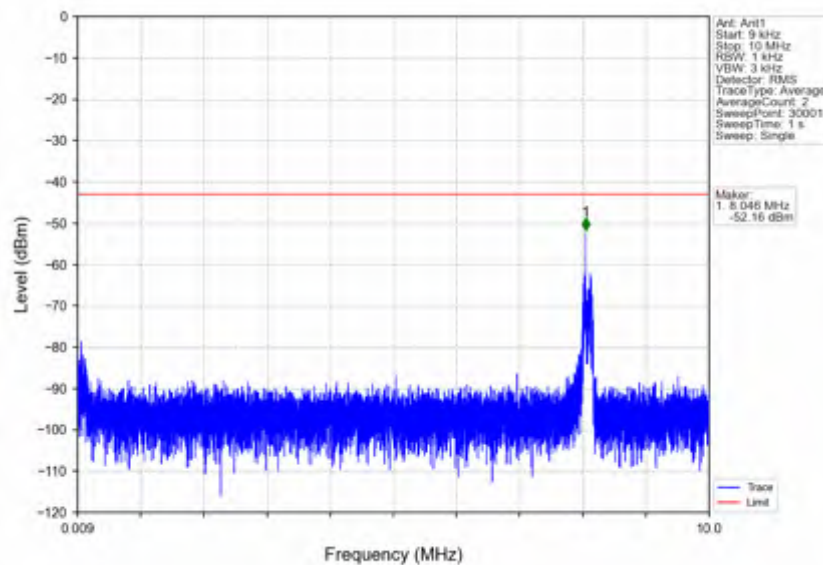
n7_15kHz_SISO_NTNV_15MHz_DFT-s-OFDM_PI/2_BPSK_2562.5MHz_Inner_1RB_Right
