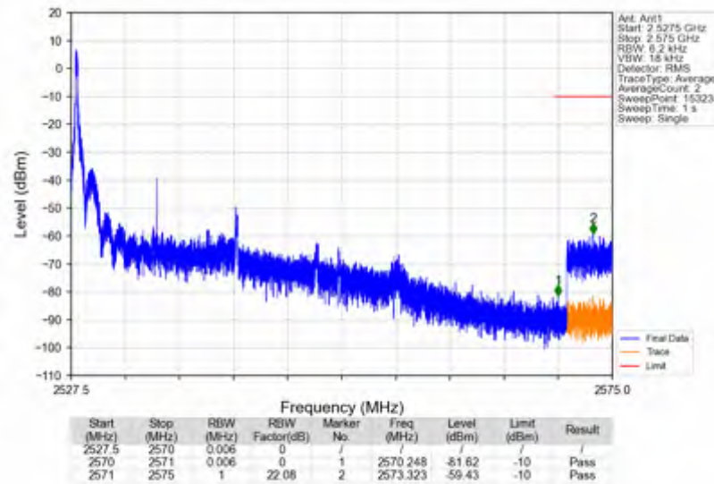
n7_15kHz_SISO_NTNV_15MHz_DFT-s-OFDM_QPSK_2535MHz_Edge_1RB_Left
