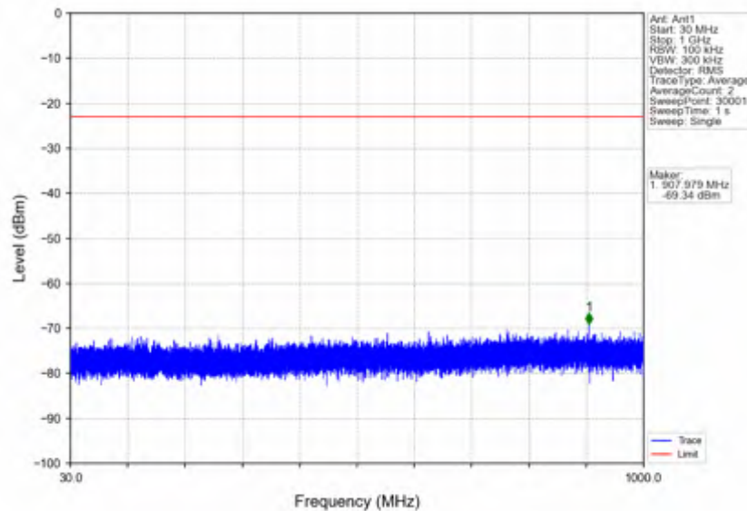
n7_15kHz_SISO_NTNV_15MHz_DFT-s-OFDM QPSK_2562.5MHz_Edge_1RB_Right
