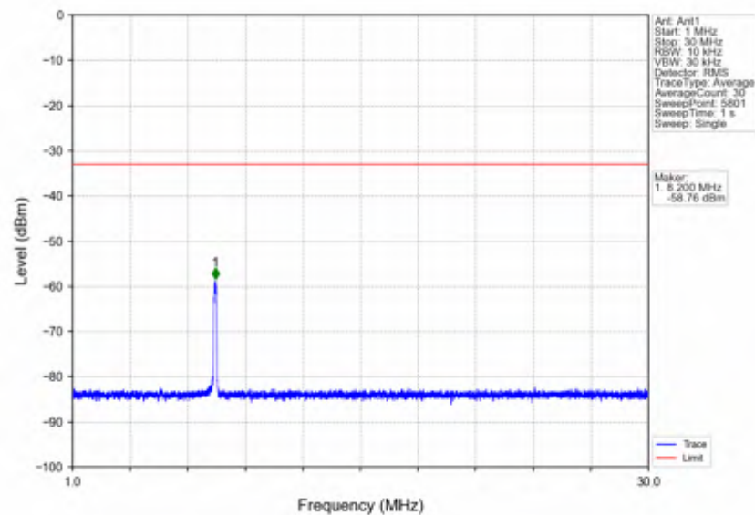
n7_15kHz_SISO_NTNV_20MHz_DFT-s-OFDM QPSK_2560MHz_Edge_1RB_Right
