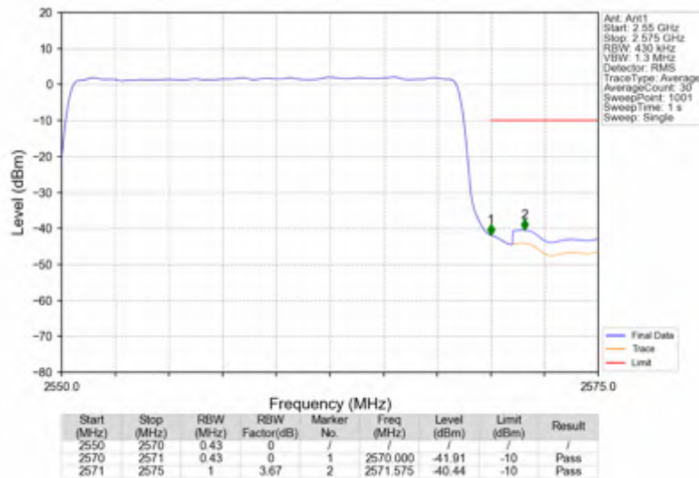
n7_15kHz_SISO_NTNV_20MHz_DFT-s-OFDM PI/2 BPSK_2560MHz_Outer_Full
