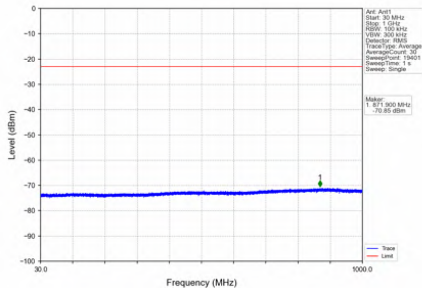
n7_15kHz_SISO_NTNV_20MHz_CP-OFDM_QPSK_2560MHz_Edge_1RB_Right
