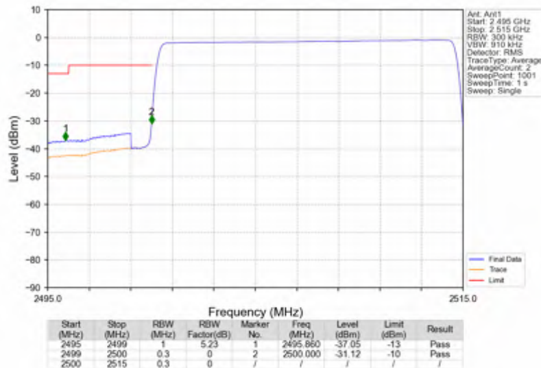
n7_15kHz_SISO_NTNV_15MHz_CP-OFDM QPSK_2507.5MHz_Outer_Full
