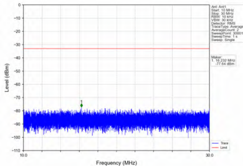
n7_15kHz_SISO_NTNV_15MHz_DFT-s-OFDM_QPSK_2507.5MHz_Inner_1RB_Left
