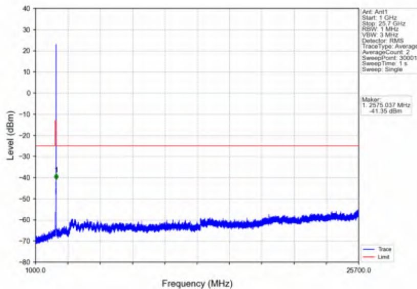
n7_15kHz_SISO_NTNV_15MHz_DFT-s-OFDM QPSK_2562.5MHz_Inner_1RB_Right
