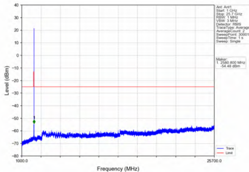
n7_15kHz_SISO_NTNV_10MHz_DFT-s-OFDM QPSK_2565MHz_Edge_1RB_Right
