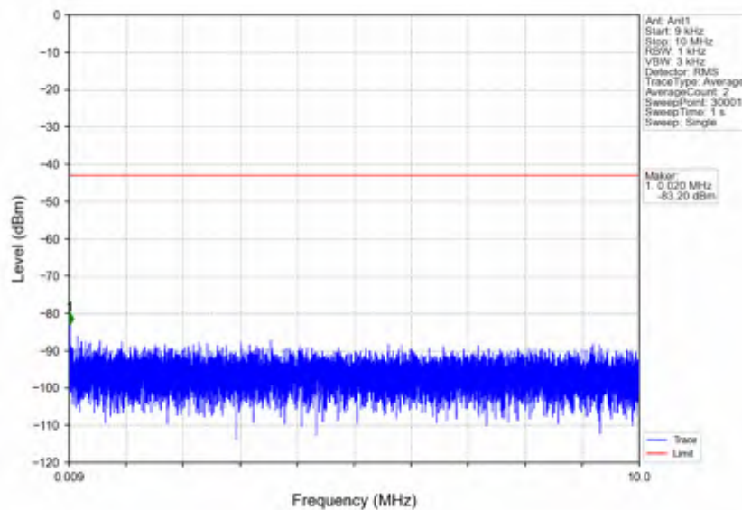
n7_15kHz_SISO_NTNV_5MHz_DFT-s-OFDM QPSK_2502.5MHz_Outer_Full
