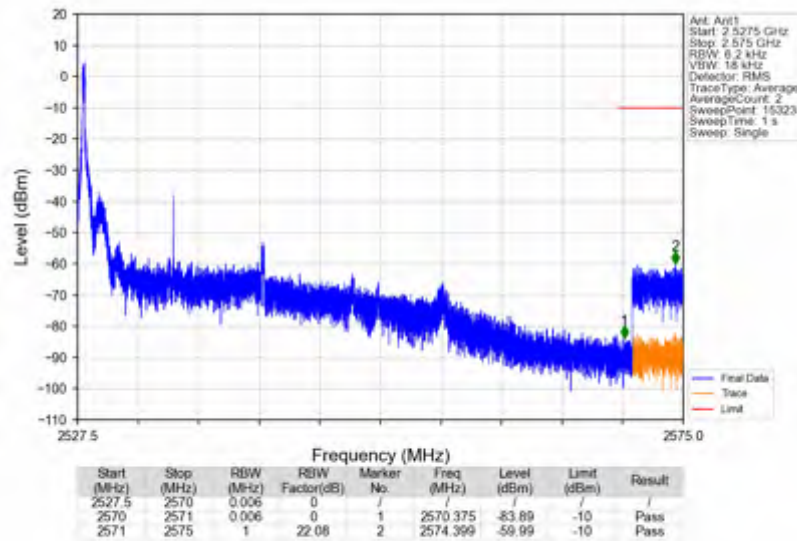
n7_15kHz_SISO_NTNV_15MHz_CP-OFDM QPSK_2535MHz_Edge_1RB_Left
