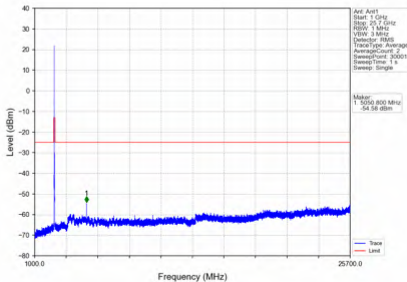
n7_15kHz_SISO_NTNV_20MHz_DFT-s-OFDM QPSK_2560MHz_Edge_1RB_Right
