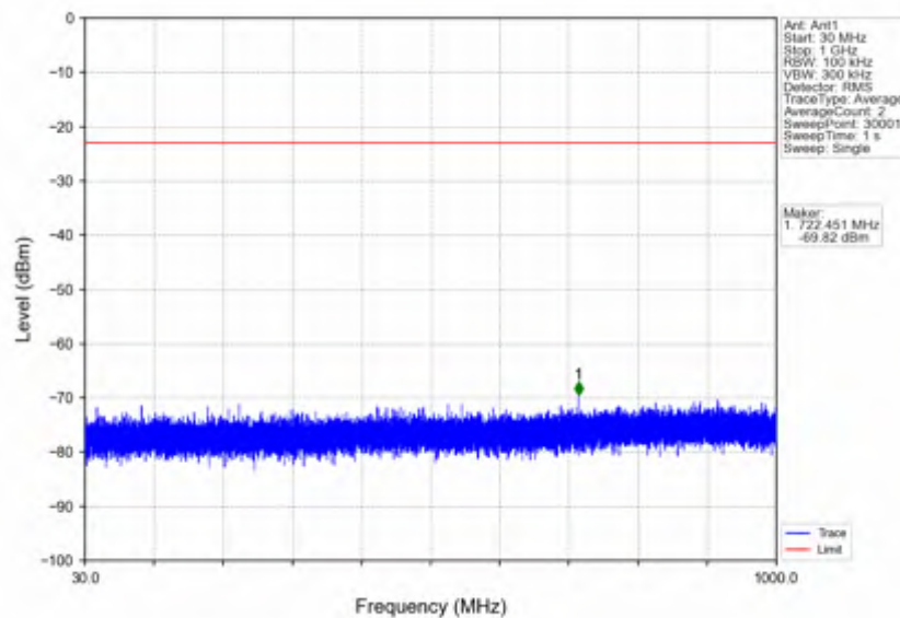
n7_15kHz_SISO_NTNV_10MHz_CP-OFDM_QPSK_2505MHz_Outer_Full
