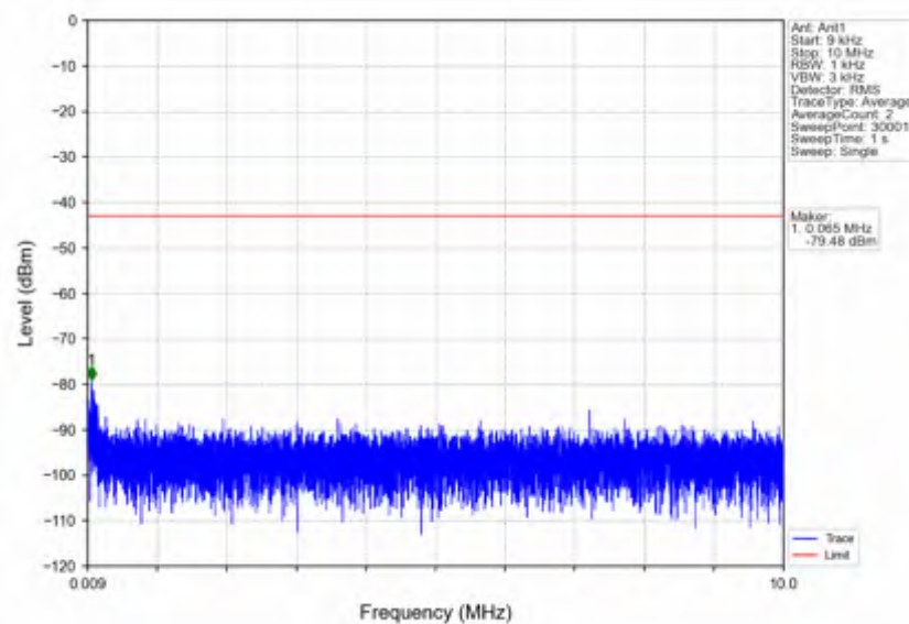
n7_15kHz_SISO_NTNV_20MHz_DFT-s-OFDM_QPSK_2535MHz_Edge_1RB_Left
