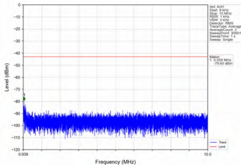
n7_15kHz_SISO_NTNV_10MHz_DFT-s-OFDM PI/2 BPSK_2535MHz_Edge_1RB_Left
