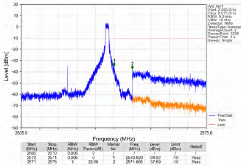
n7_15kHz_SISO_NTNV_5MHz_CP-OFDM_QPSK_2567.5MHz_Edge_1RB_Right
