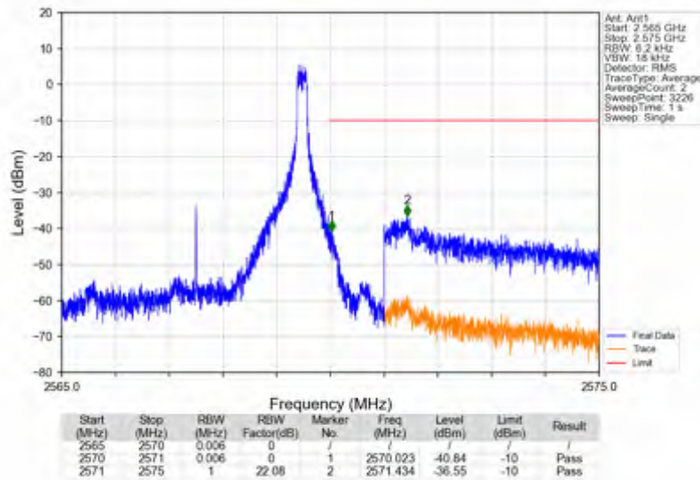
n7_15kHz_SISO_NTNV_5MHz_CP-OFDM_QPSK_2567.5MHz_Inner_1RB_Right
