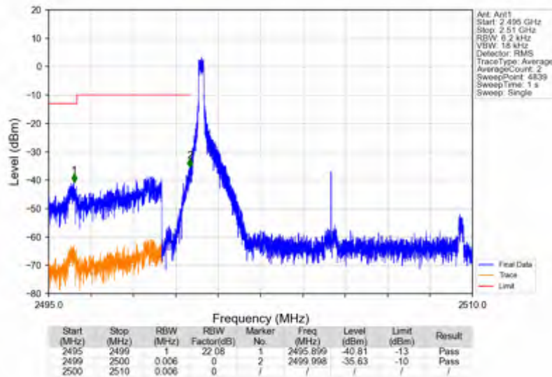
n7_15kHz_SISO_NTNV_10MHz_CP-OFDM QPSK_2505MHz_Edge_1RB_Left
