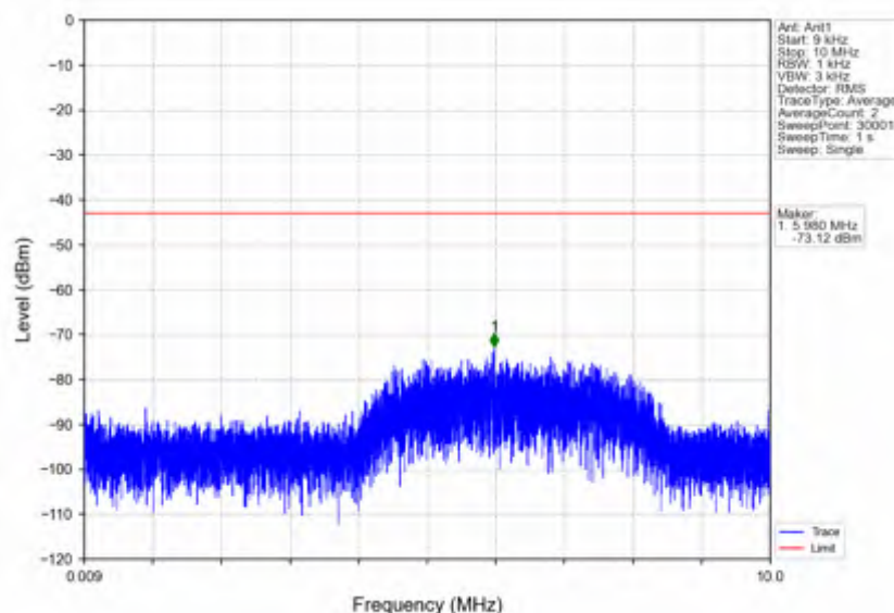
n7_15kHz_SISO_NTNV_5MHz_DFT-s-OFDM_QPSK_2567.5MHz_Outer_Full
