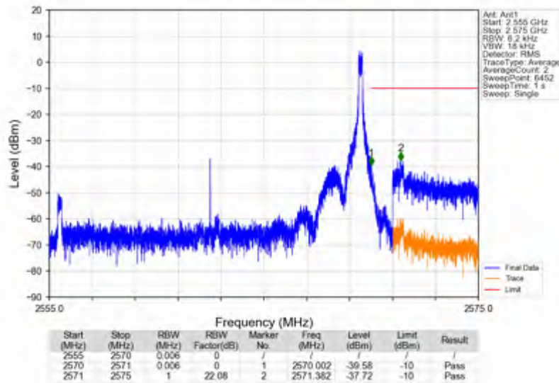
n7_15kHz_SISO_NTV_15MHz_CP-OFDM_QPSK_2562.5MHz_Edge_1RB_Right
