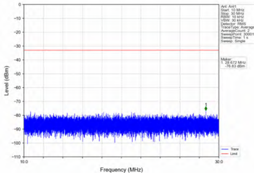
n7_15kHz_SISO_NTNV_15MHz_CP-OFDM_QPSK_2562.5MHz_Edge_1RB_Right
