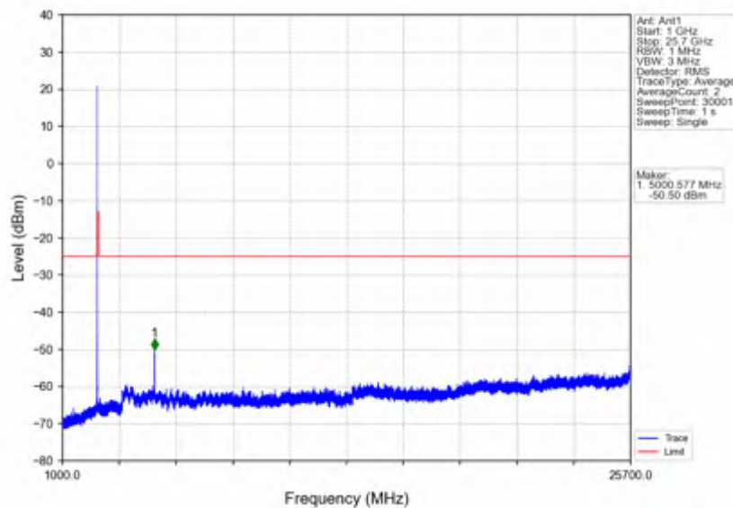
n7_15kHz_SISO_NTNV_5MHz_CP-OFDM QPSK_2535MHz_Edge_1RB_Left
