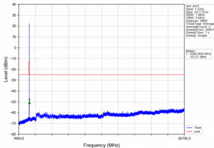
n7_15kHz_SISO_NTNV_10MHz_DFT-s-OFDM_QPSK_2565MHz_Inner_1RB_Right
