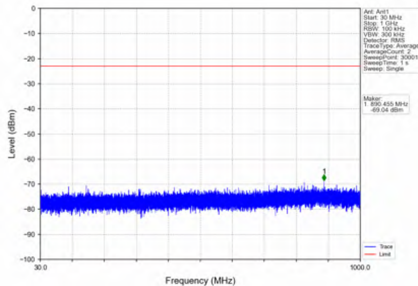
n7_15kHz_SISO_NTNV_10MHz_DFT-s-OFDM QPSK_2565MHz_Edge_1RB_Right
