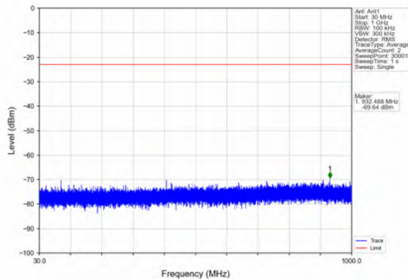
n7_15kHz_SISO_NTNV_5MHz_DFT-s-OFDM_QPSK_2567.5MHz_Inner_1RB_Right
