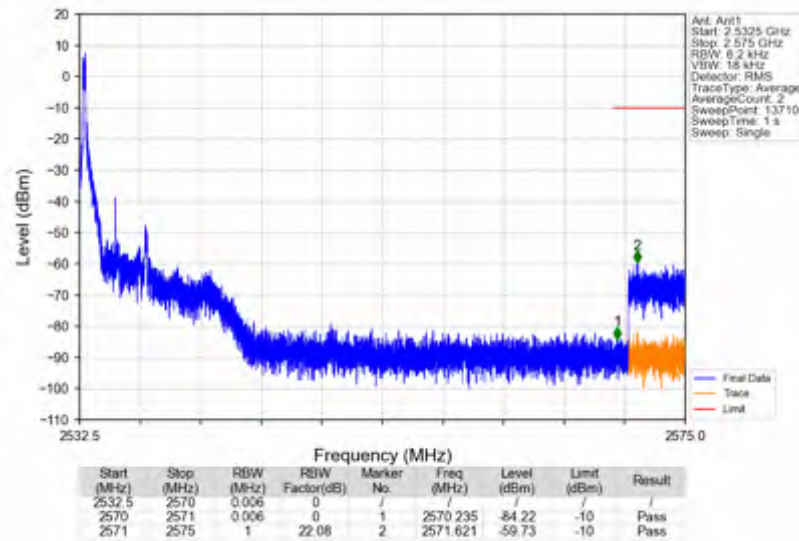
n7_15kHz_SISO_NTNV_5MHz_DFT-s-OFDM_QPSK_2535MHz_Edge_1RB_Left
