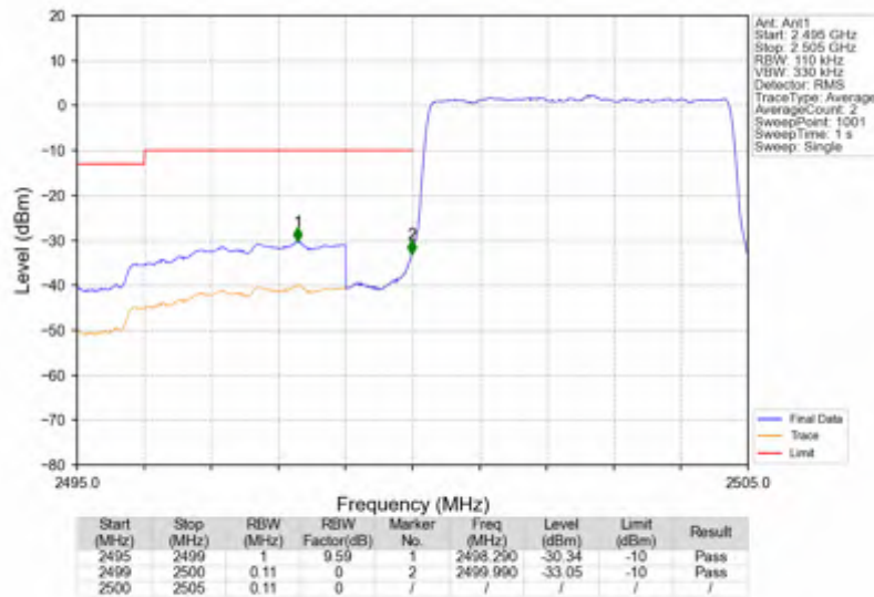
n7_15kHz_SISO_NTNV_5MHz_DFT-s-OFDM QPSK_2502.5MHz_Outer_Full
