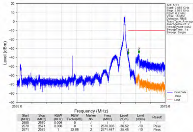
n7_15kHz_SISO_NTNV_15MHz_DFT-s-OFDM QPSK_2562.5MHz_Edge_1RB_Right
