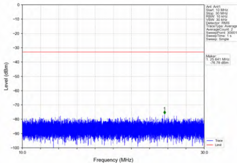
n7_15kHz_SISO_NTNV_15MHz_CP-OFDM QPSK_2562.5MHz_Inner_1RB_Right
