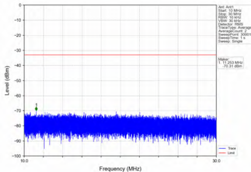
n7_15kHz_SISO_NTNV_15MHz_DFT-s-OFDM QPSK_2562.5MHz_Outer_Full
