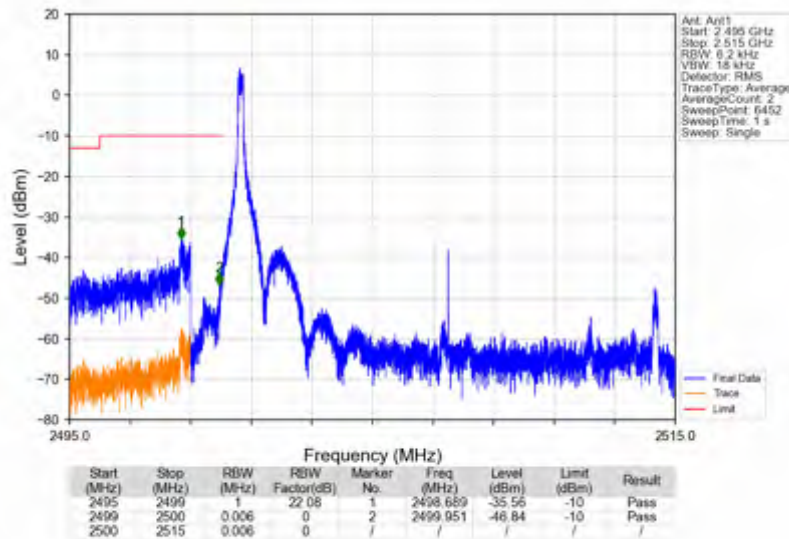
n7_15kHz_SISO_NTNV_15MHz_DFT-s-OFDM QPSK_2507.5MHz_Inner_1RB_Left
