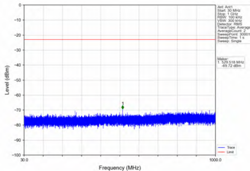
n7_15kHz_SISO_NTNV_10MHz_DFT-s-OFDM_QPSK_2505MHz_Outer_Full
