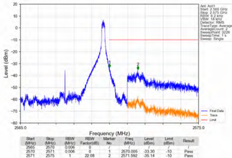
n7_15kHz_SISO_NTNV_5MHz_DFT-s-OFDM QPSK_2567.5MHz_Edge_1RB_Right
