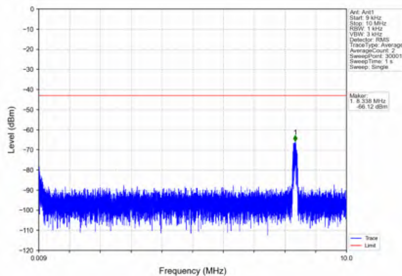
n7_15kHz_SISO_NTNV_10MHz_CP-OFDM_QPSK_2565MHz_Edge_1RB_Right
