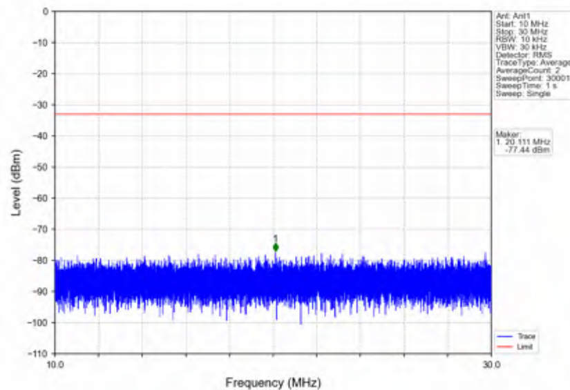
n7_15kHz_SISO_NTNV_5MHz_DFT-s-OFDM QPSK_2567.5MHz_Edge_1RB_Right
