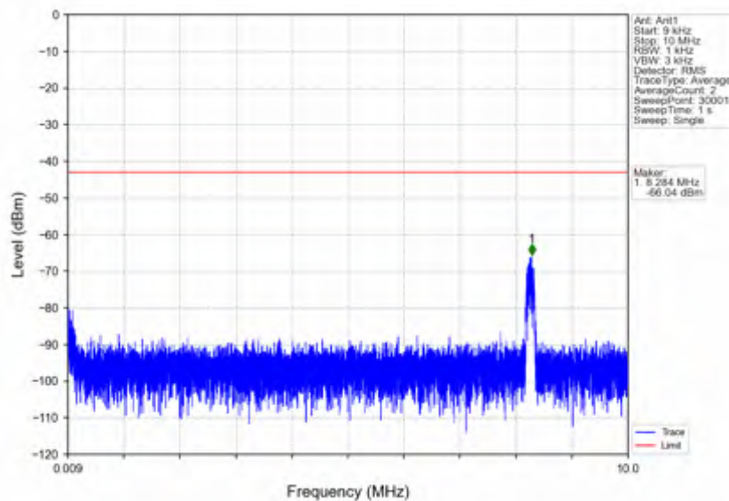
n7_15kHz_SISO_NTV_15MHz_CP-OFDM_QPSK_2562.5MHz_Edge_1RB_Right
