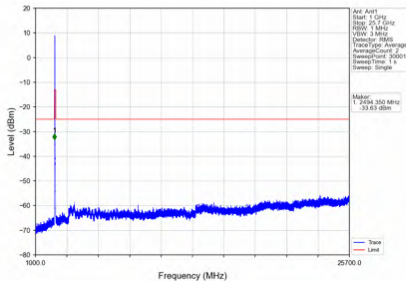
n7_15kHz_SISO_NTNV_20MHz_CP-OFDM_QPSK_2510MHz_Outer_Full
