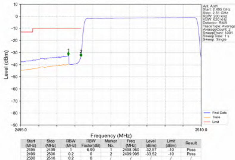
n7_15kHz_SISO_NTNV_10MHz_CP-OFDM QPSK_2505MHz_Outer_Full
