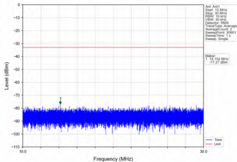
n7_15kHz_SISO_NTNV_10MHz_DFT-s-OFDM PI/2 BPSK_2505MHz_Outer_Full
