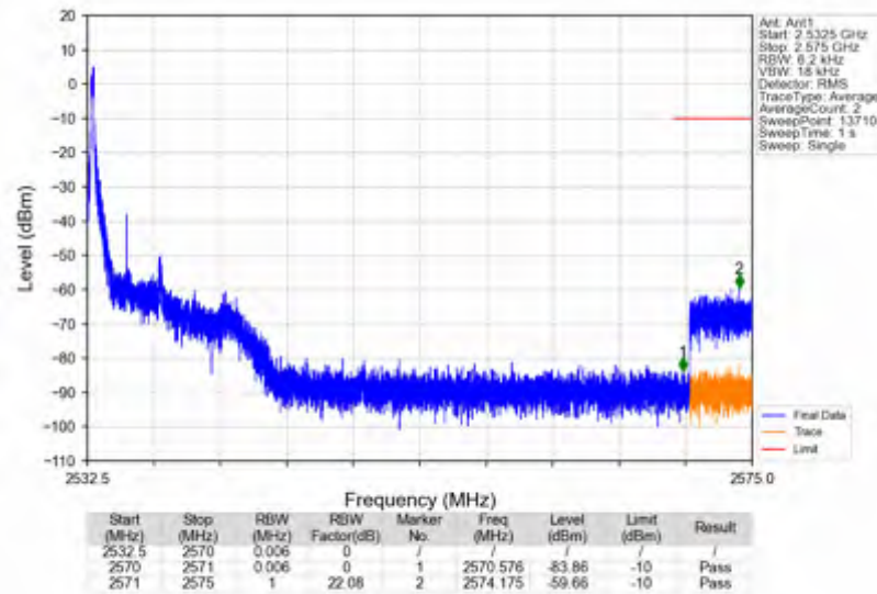
n7_15kHz_SISO_NTNV_5MHz_CP-OFDM QPSK_2535MHz_Edge_1RB_Left
