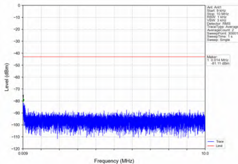
n7_15kHz_SISO_NTNV_15MHz_CP-OFDM_QPSK_2507.5MHz_Edge_1RB_Left
