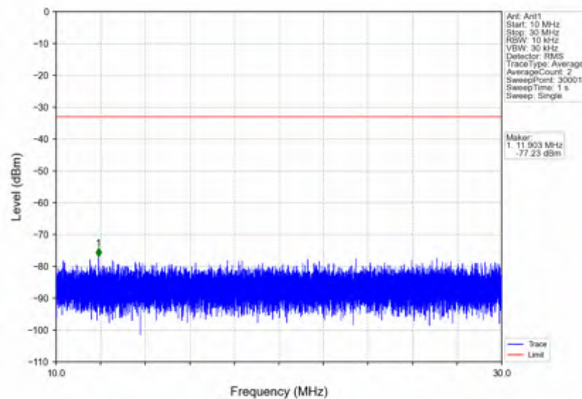
n7_15kHz_SISO_NTNV_15MHz_DFT-s-OFDM QPSK_2507.5MHz_Edge_1RB_Left
