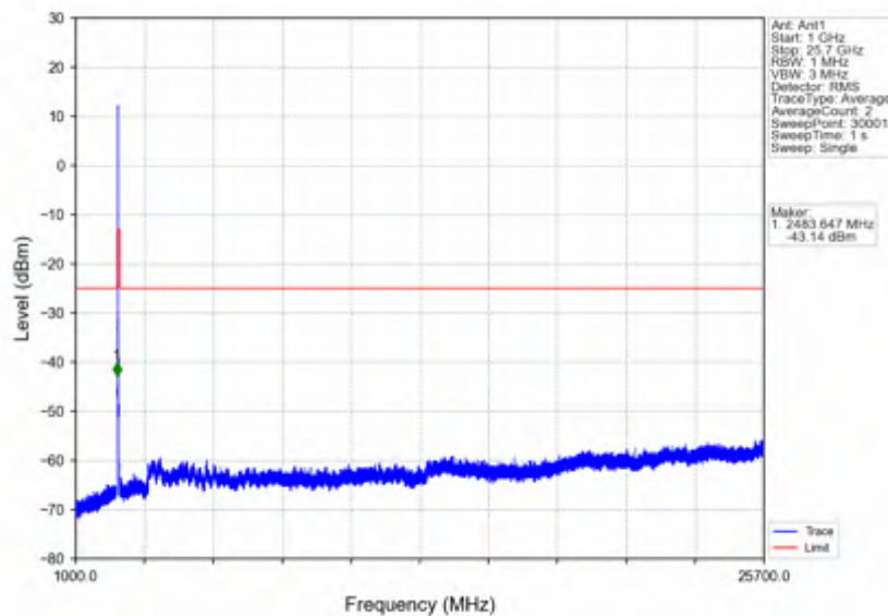
n7_15kHz_SISO_NTNV_15MHz_DFT-s-OFDM QPSK_2507.5MHz_Inner_1RB_Left
