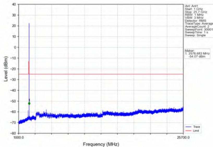
n7_15kHz_SISO_NTNV_5MHz_DFT-s-OFDM_QPSK_2567.5MHz_Inner_1RB_Right
