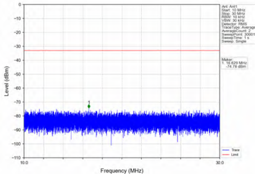
n7_15kHz_SISO_NTNV_10MHz_CP-OFDM_QPSK_2565MHz_Outer_Full
