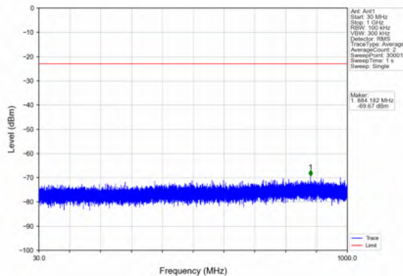
n7_15kHz_SISO_NTNV_5MHz_DFT-s-OFDM_QPSK_2502.5MHz_Inner_1RB_Left
