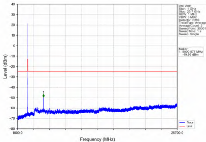
n7_15kHz_SISO_NTNV_10MHz_DFT-s-OFDM PI/2 BPSK_2505MHz_Outer_Full
