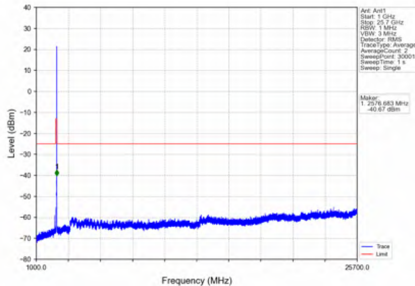
n7_15kHz_SISO_NTNV_15MHz_DFT-s-OFDM QPSK_2562.5MHz_Edge_1RB_Right
