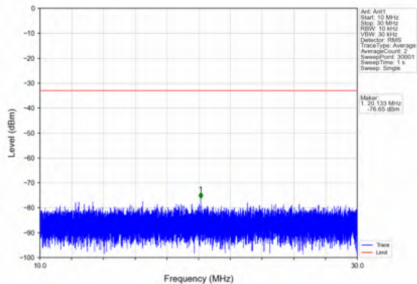
n7_15kHz_SISO_NTNV_5MHz_CP-OFDM QPSK_2535MHz_Edge_1RB_Left
