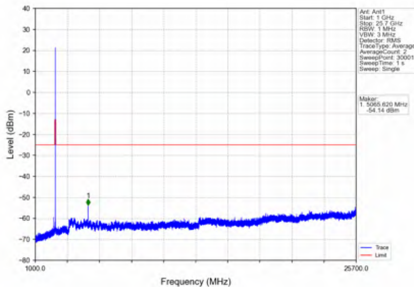
n7_15kHz_SISO_NTNV_5MHz_DFT-s-OFDM QPSK_2567.5MHz_Edge_1RB_Right
