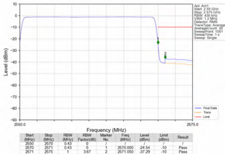
n7_15kHz_SISO_NTNV_20MHz_CP-OFDM QPSK_2560MHz_Outer_Full
