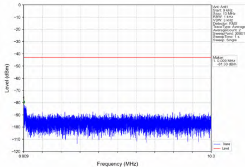
n7_15kHz_SISO_NTNV_10MHz_DFT-s-OFDM QPSK_2505MHz_Edge_1RB_Left
