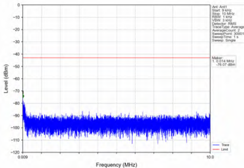
n7_15kHz_SISO_NTNV_15MHz_CP-OFDM_QPSK_2507.5MHz_Inner_1RB_Left
