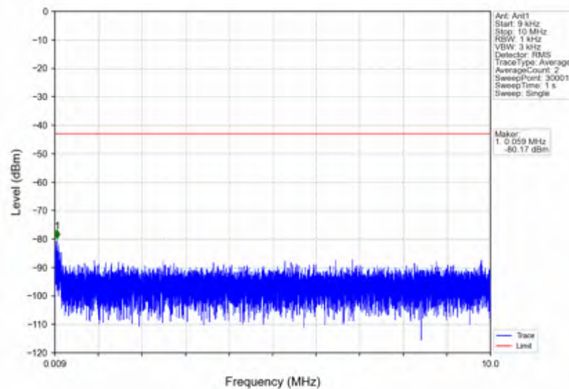
n7_15kHz_SISO_NTNV_10MHz_CP-OFDM QPSK_2535MHz_Edge_1RB_Left
