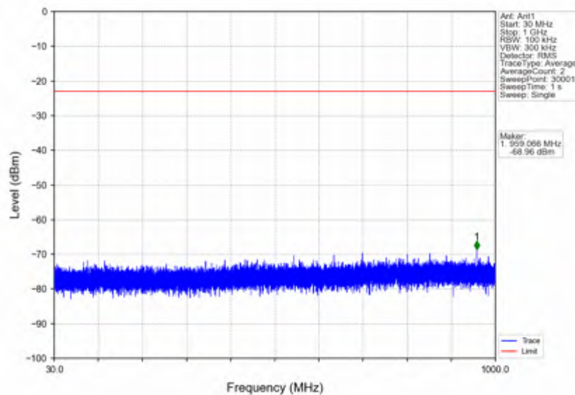
n7_15kHz_SISO_NTNV_15MHz_CP-OFDM QPSK_2507.5MHz_Outer_Full
