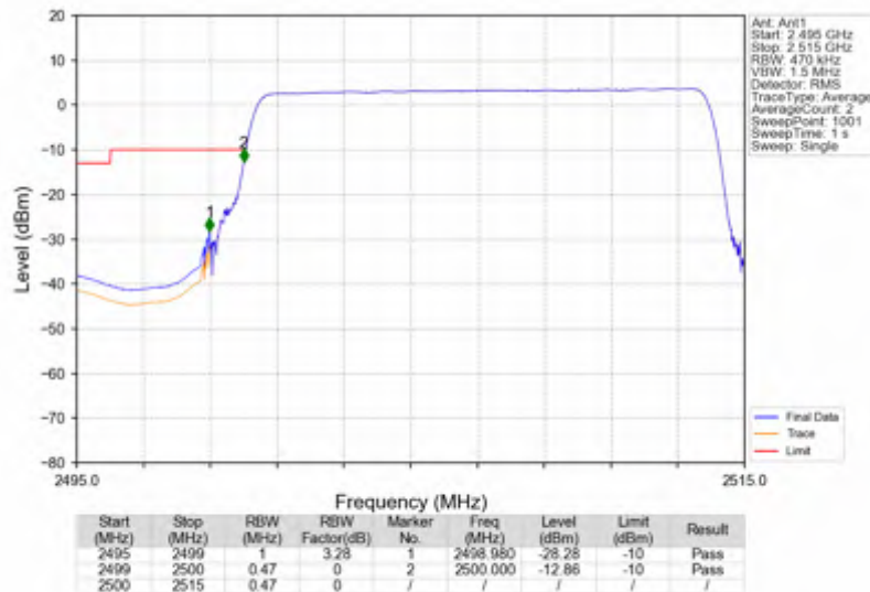
n7_15kHz_SISO_NTNV_15MHz_DFT-s-OFDM PI/2 BPSK_2507.5MHz_Outer_Full
