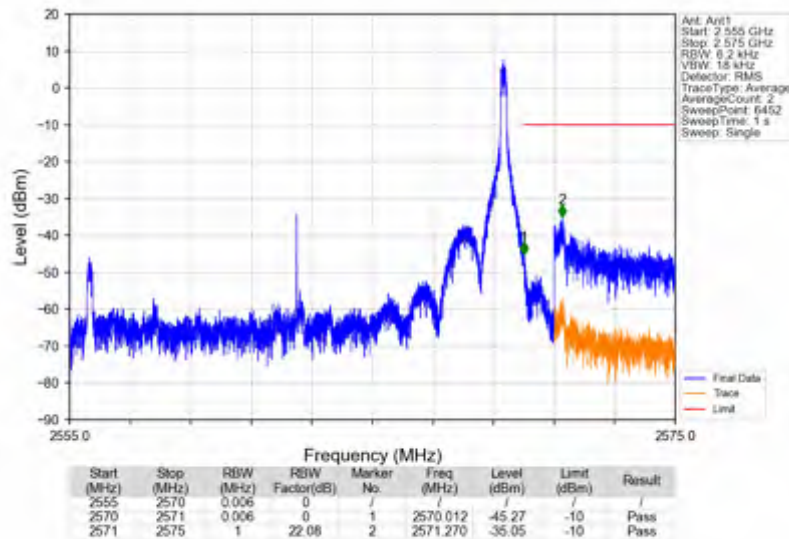
n7_15kHz_SISO_NTNV_15MHz_DFT-s-OFDM QPSK_2562.5MHz_Inner_1RB_Right
