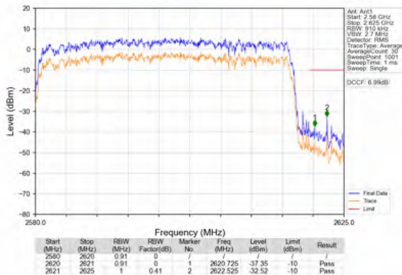
n38_30kHz_SISO_NTNV_40MHz_DFT-s-OFDM_PI/2_BPSK_2600MHz_Outer_Full
