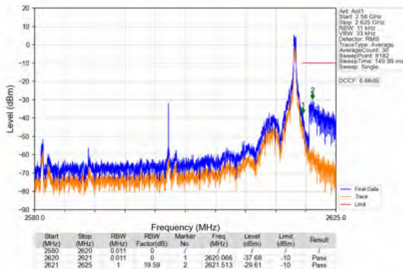
n38_30kHz_SISO_NTNV_40MHz_DFT-s-OFDM_PI/2_BPSK_2600MHz_Edge_1RB_Right
