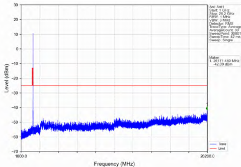
n38_30kHz_SISO_NTNV_20MHz_DFT-s-OFDM QPSK_2610MHz_Edge_1RB_Right
