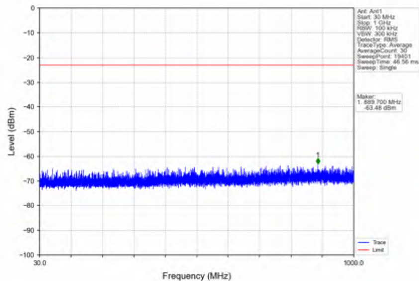
n38_30kHz_SISO_NTNV_40MHz_DFT-s-OFDM PI/2 BPSK_2600MHz_Edge_1RB_Right
