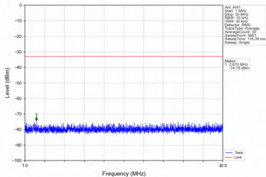
n38_30kHz_SISO_NTNV_20MHz_CP-OFDM QPSK_2610MHz_Edge_1RB_Right
