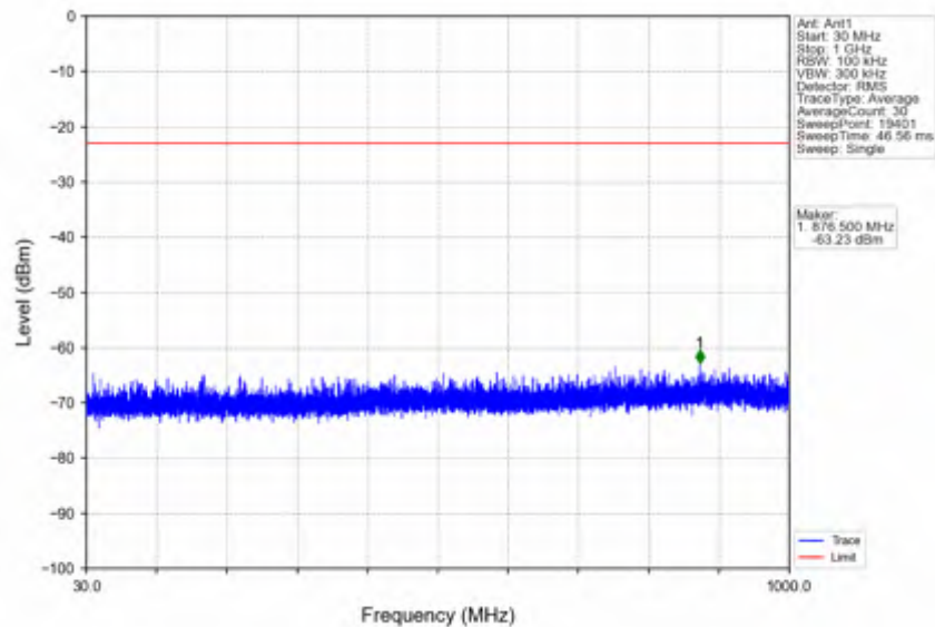
n38_30kHz_SISO_NTNV_25MHz_DFT-s-OFDM PI/2 BPSK_2595MHz_Edge_1RB_Left
