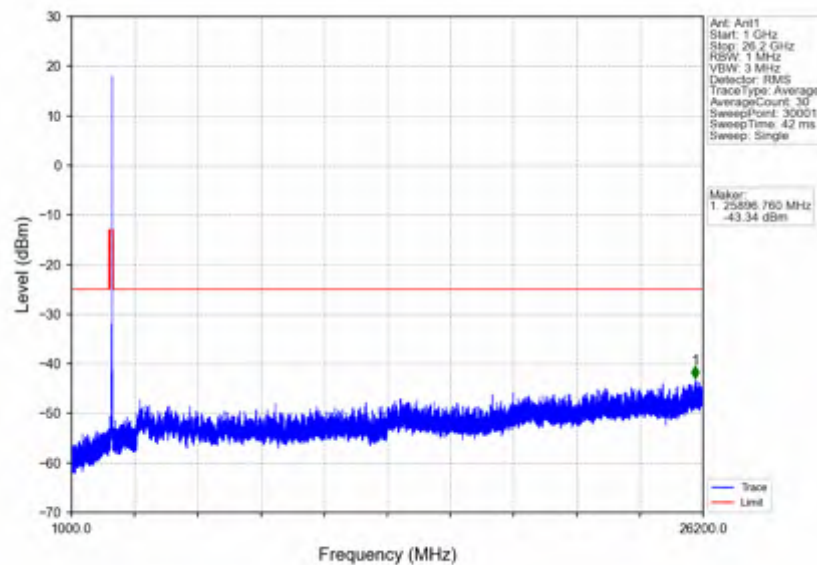
n38_30kHz_SISO_NTNV_40MHz_DFT-s-OFDM PI/2 BPSK_2600MHz_Edge_1RB_Right
