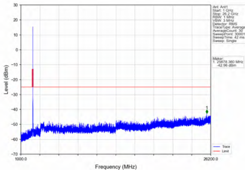
n38_30kHz_SISO_NTNV_30MHz_DFT-s-OFDM PI/2 BPSK_2605MHz_Edge_1RB_Right
