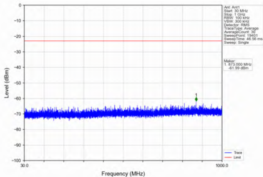
n38_30kHz_SISO_NTNV_15MHz_DFT-s-OFDM PI/2 BPSK_2595MHz_Edge_1RB_Left
