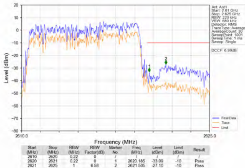
n38_30kHz_SISO_NTNV_10MHz_DFT-s-OFDM QPSK_2615MHz_Outer_Full
