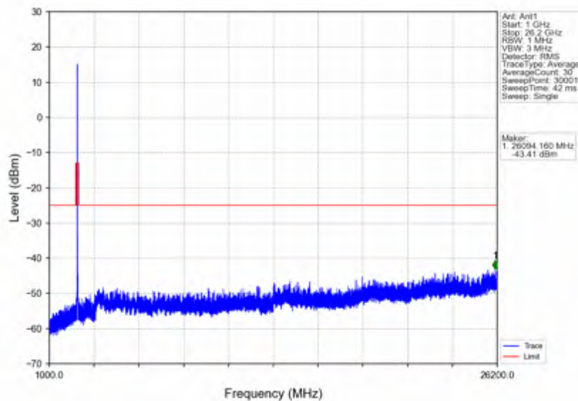
n38_30kHz_SISO_NTNV_40MHz_CP-OFDM QPSK_2590MHz_Outer_Full
