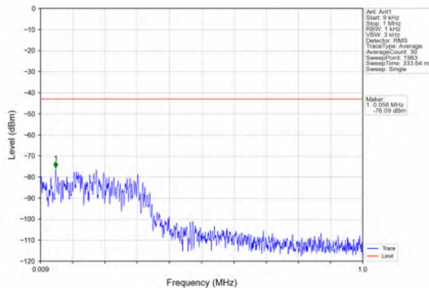
n38_30kHz_SISO_NTNV_20MHz_DFT-s-OFDM_QPSK_2610MHz_Edge_1RB_Right
