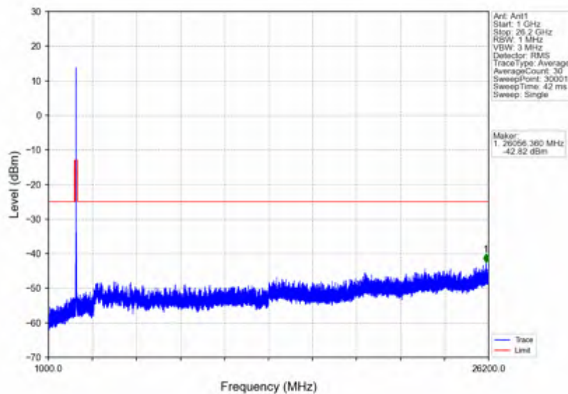
n38_30kHz_SISO_NTNV_40MHz_DFT-s-OFDM_PI/2_BPSK_2600MHz_Edge_1RB_Right
