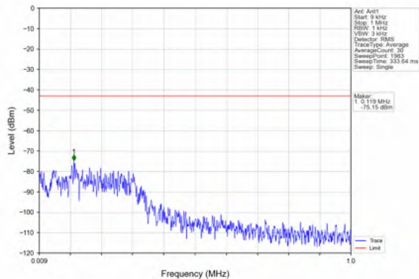
n38_30kHz_SISO_NTNV_25MHz_DFT-s-OFDM QPSK 2607.5MHz_Edge_1RB_Right
