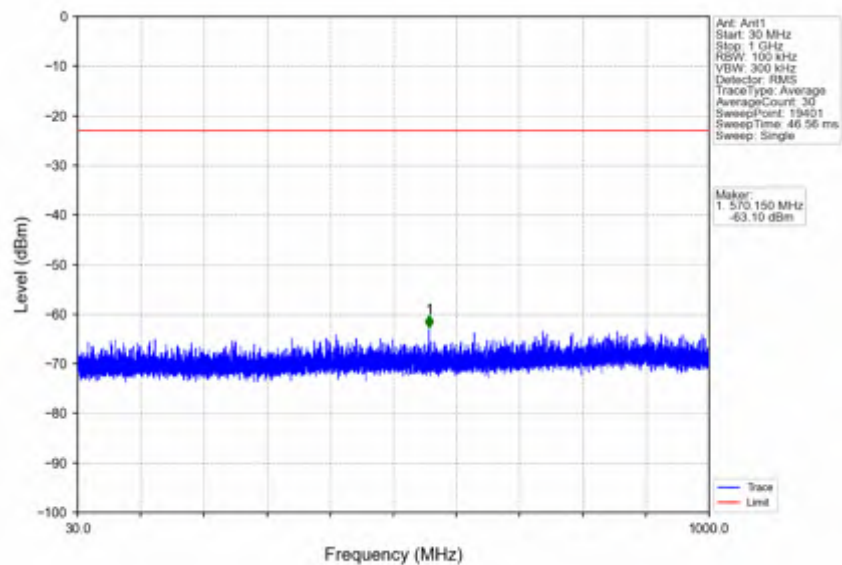
n38_30kHz_SISO_NTNV_25MHz_CP-OFDM_QPSK_2595MHz_Edge_1RB_Left
