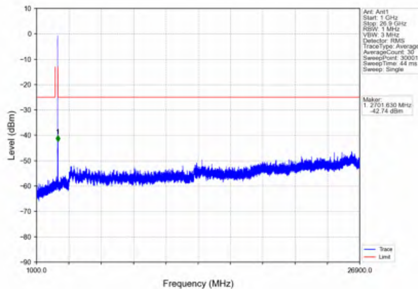
n41_15kHz_SISO_NTNV_10MHz_DFT-s-OFDM PI/2 BPSK_2685MHz_Outer_Full
