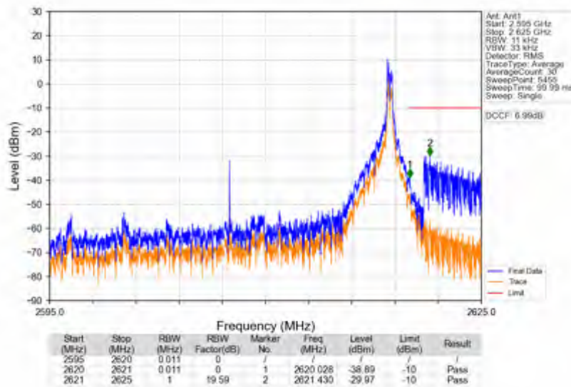
n38_30kHz_SISO_NTNV_25MHz_DFT-s-OFDM PI/2 BPSK_2607.5MHz_Inner_1RB_Right
