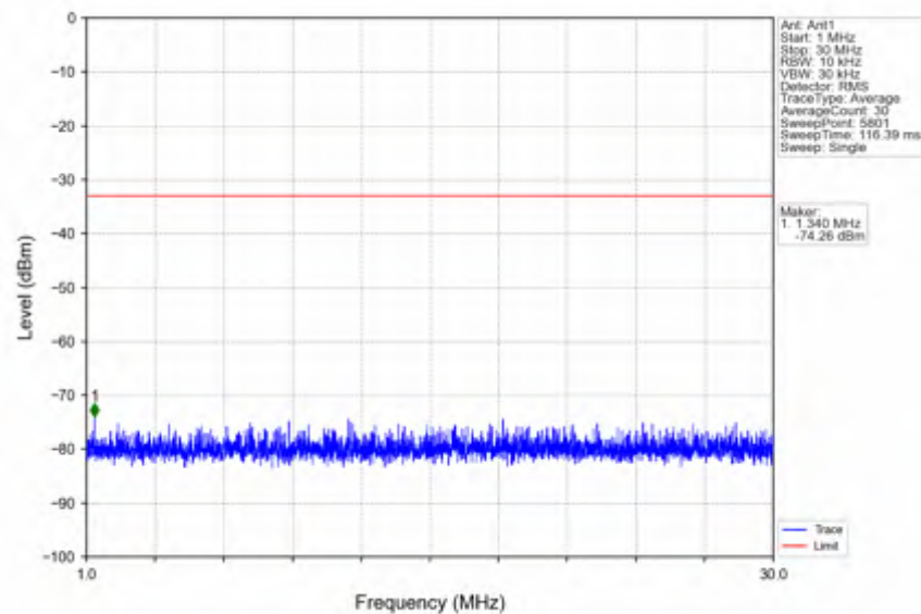
n38_30kHz_SISO_NTNV_25MHz_CP-OFDM QPSK_2607.5MHz_Edge_1RB_Right
