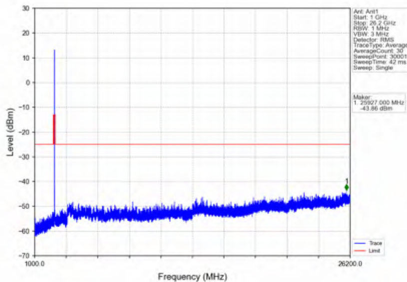
n38_30kHz_SISO_NTNV_20MHz_DFT-s-OFDM QPSK_2580MHz_Outer_Full
