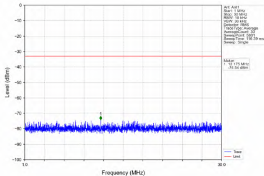
n38_30kHz_SISO_NTNV_30MHz_DFT-s-OFDM PI/2 BPSK_2605MHz_Edge_1RB_Right
