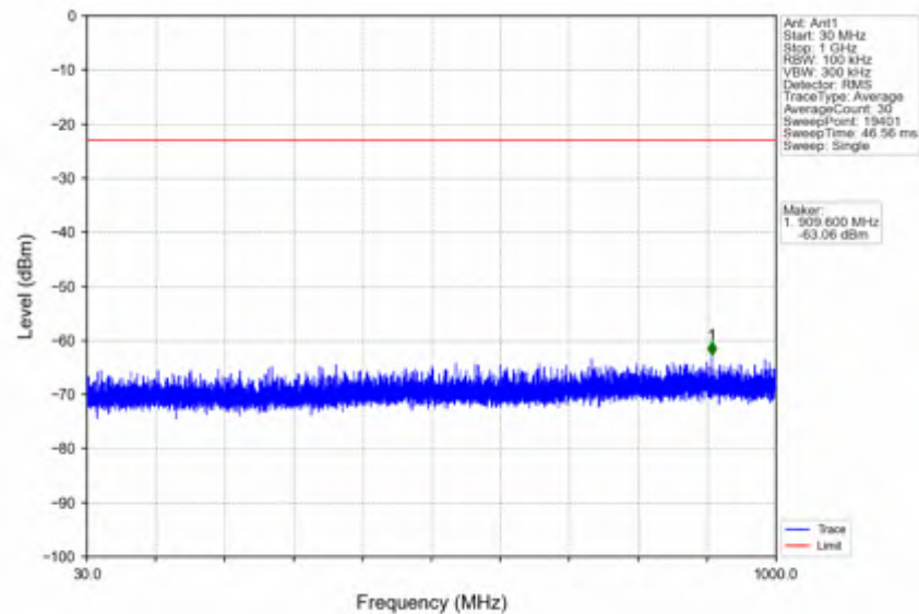
n38_30kHz_SISO_NTNV_40MHz_CP-OFDM QPSK_2600MHz_Edge_1RB_Right
