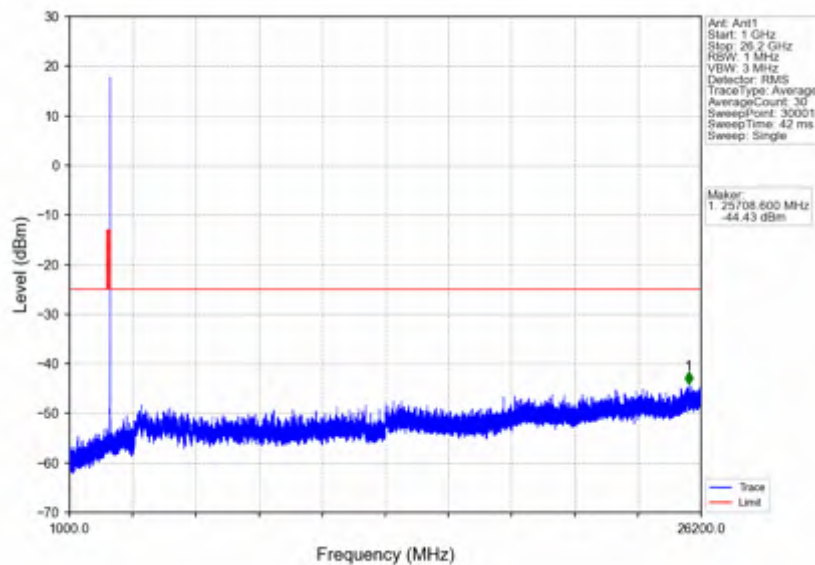
n38_30kHz_SISO_NTNV_10MHz_DFT-s-OFDM QPSK_2615MHz_Outer_Full
