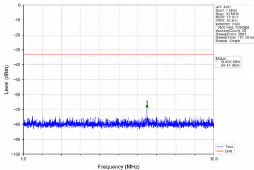
n38_30kHz_SISO_NTNV_30MHz_DFT-s-OFDM PI/2 BPSK_2595MHz_Edge_1RB_Left
