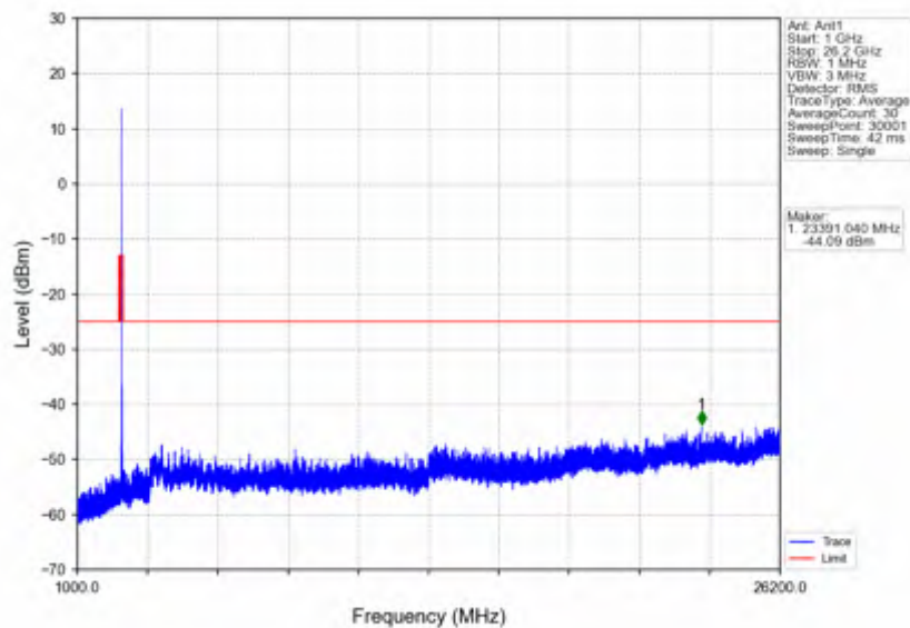
n38_30kHz_SISO_NTNV_20MHz_DFT-s-OFDM QPSK_2610MHz_Edge_1RB_Right
