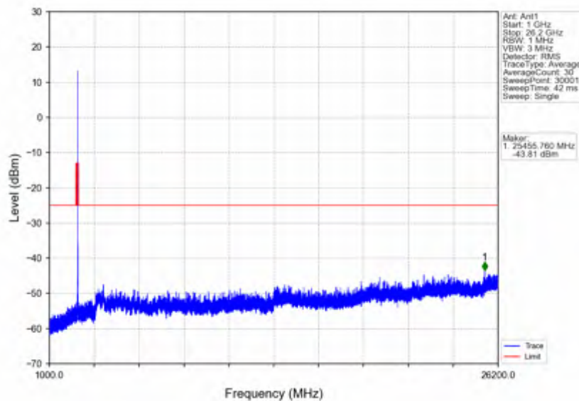
n38_30kHz_SISO_NTNV_15MHz_DFT-s-OFDM QPSK_2612.5MHz_Edge_1RB_Right
