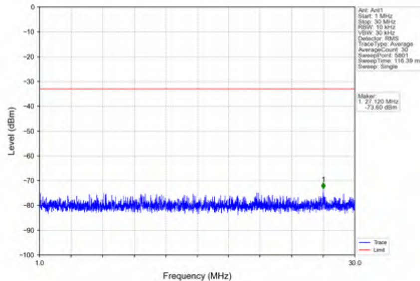
n38_30kHz_SISO_NTNV_15MHz_DFT-s-OFDM QPSK_2595MHz_Edge_1RB_Left
