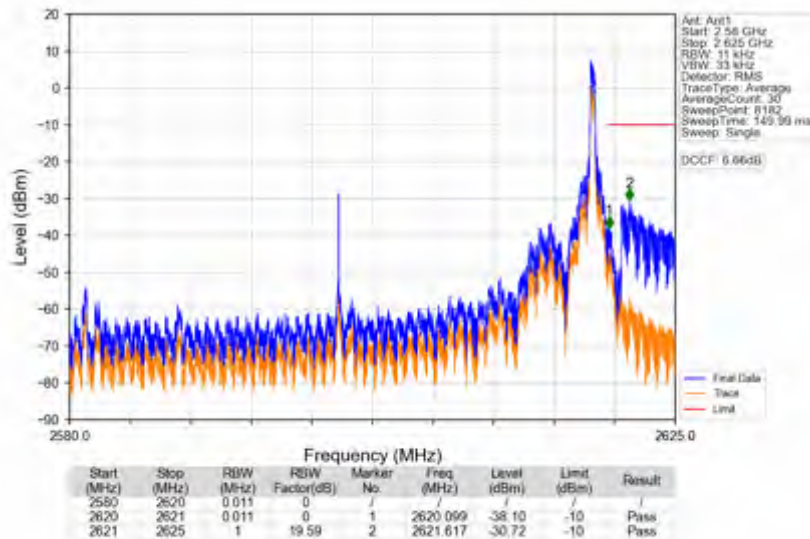
n38_30kHz_SISO_NTNV_40MHz_DFT-s-OFDM_QPSK_2600MHz_Edge_1RB_Right
