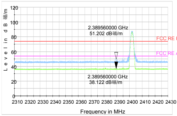
Bluetooth LE Channel 0 Peak+ Average
