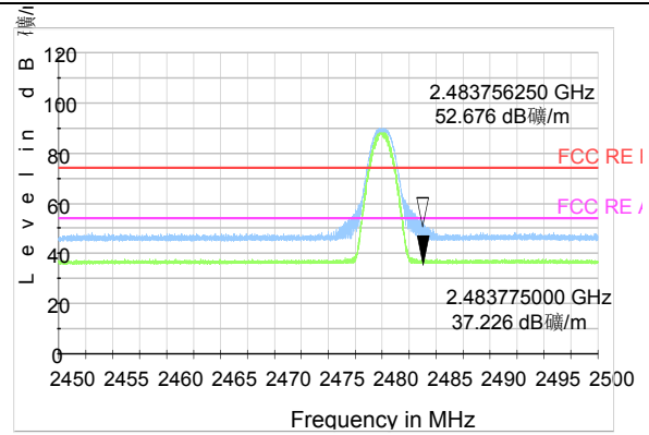
Bluetooth LE Channel 39 Peak+ Average
