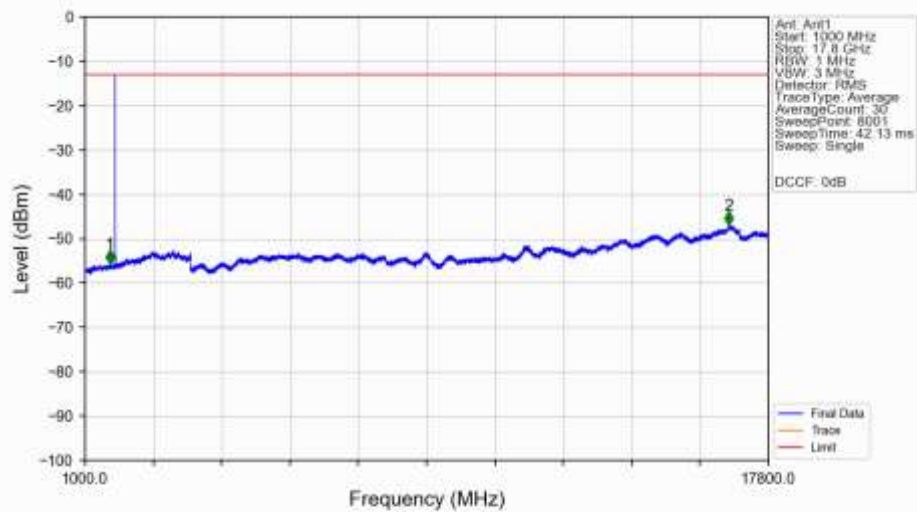
n66_30kHz_SISO_NTNV_10MHz_CP-OFDM_QPSK_1745MHz_Edge_1RB_Left_Ant1
