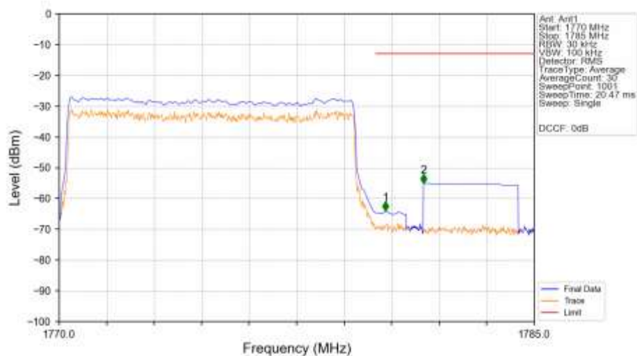
n66_15kHz_SISO_NTNV_10MHz_DFT-s-OFDM_QPSK_1775MHz_Outer_Full_Ant1
