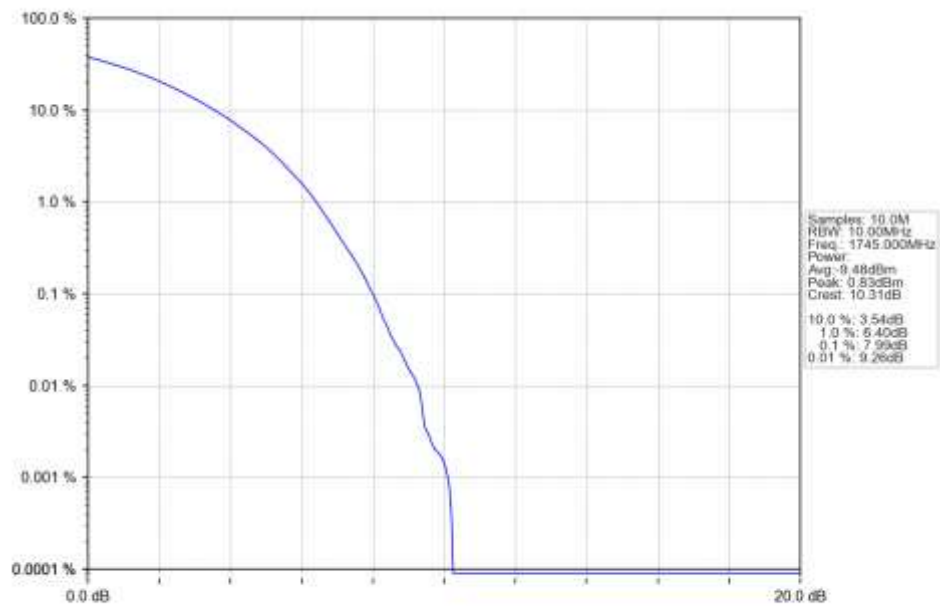
n66_30kHz_SISO_NTNV_10MHz_CP-OFDM_64_QAM_1745MHz_Outer_Full_Ant1
