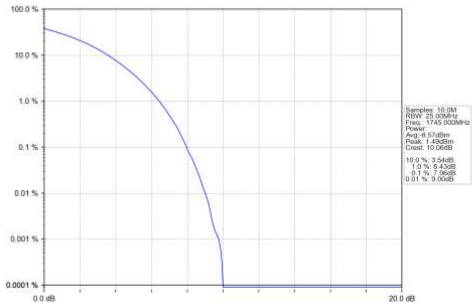
n66_30kHz_SISO_NTNV_20MHz_CP-OFDM_64_QAM_1745MHz_Outer_Full_Ant1
