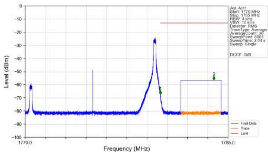
n66_15kHz_SISO_NTNV_10MHz_CP-OFDM_QPSK_1775MHz_Edge_1RB_Right_Ant1
