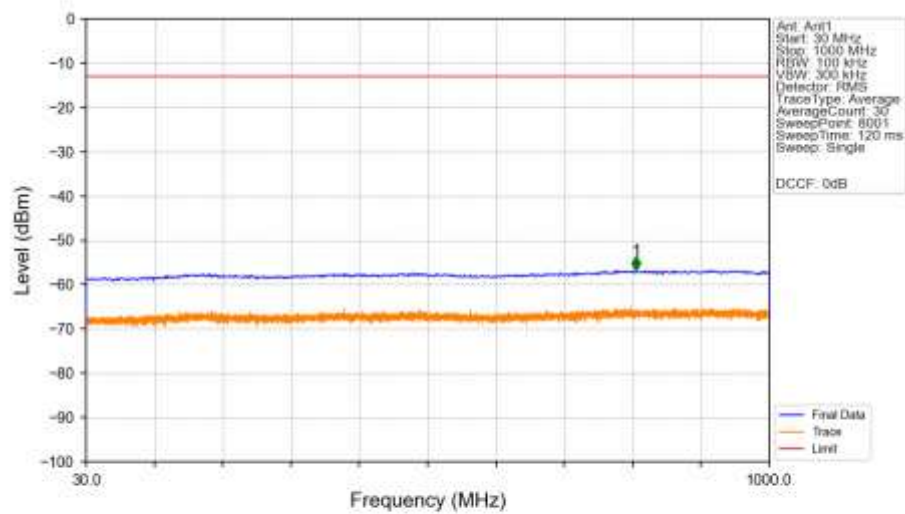
n66_15kHz_SISO_NTNV_10MHz_DFT-s-OFDM_QPSK_1715MHz_Edge_1RB_Left_Ant1
