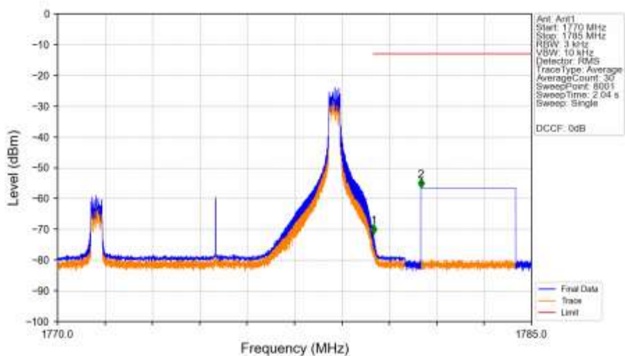
n66_30kHz_SISO_NTNV_10MHz_DFT-s-OFDM_QPSK_1775MHz_Inner_1RB_Right_Ant1
