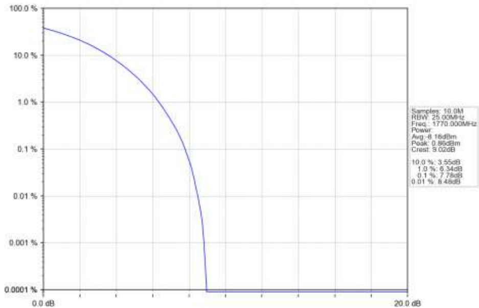
n66_30kHz_SISO_NTNV_20MHz_CP-OFDM_64_QAM_1770MHz_Outer_Full_Ant1
