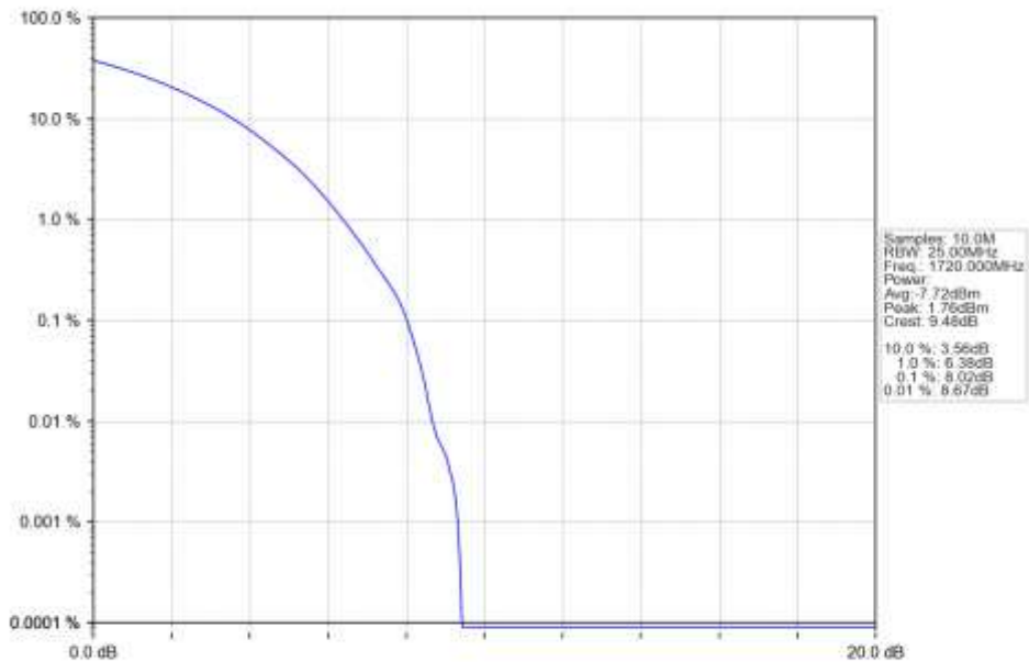
n66_30kHz_SISO_NTNV_20MHz_CP-OFDM_256_QAM_1720MHz_Outer_Full_Ant1
