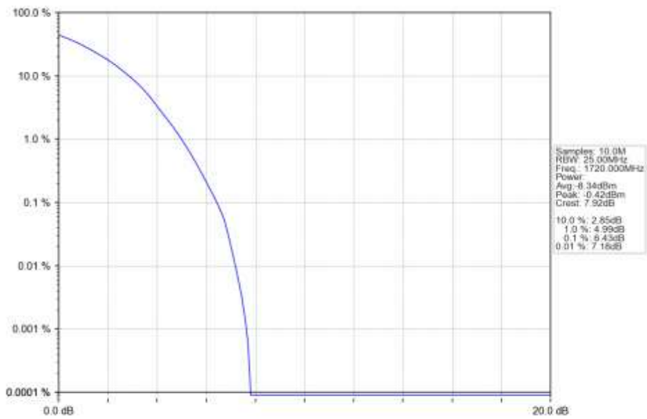
n66_15kHz_SISO_NTNV_20MHz_DFT-s-OFDM_64_QAM_1720MHz_Outer_Full_Ant1
