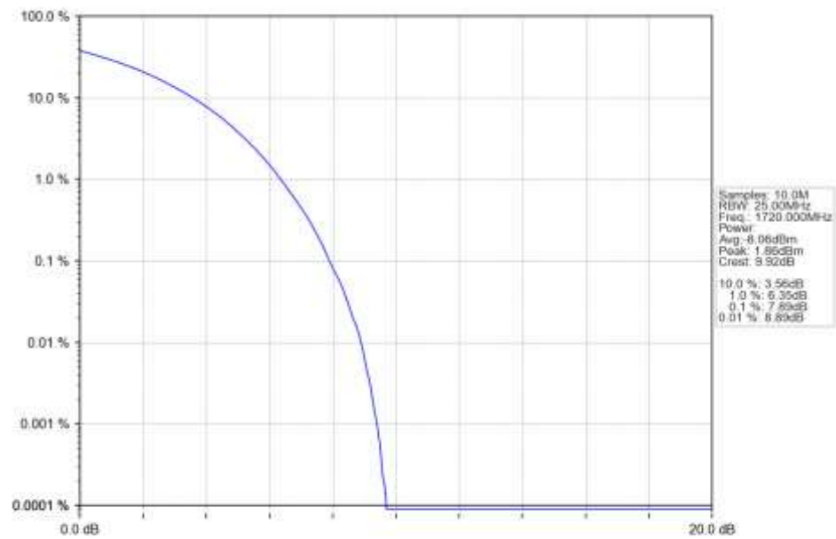
n66_15kHz_SISO_NTNV_20MHz_CP-OFDM_256_QAM_1720MHz_Outer_Full_Ant1
