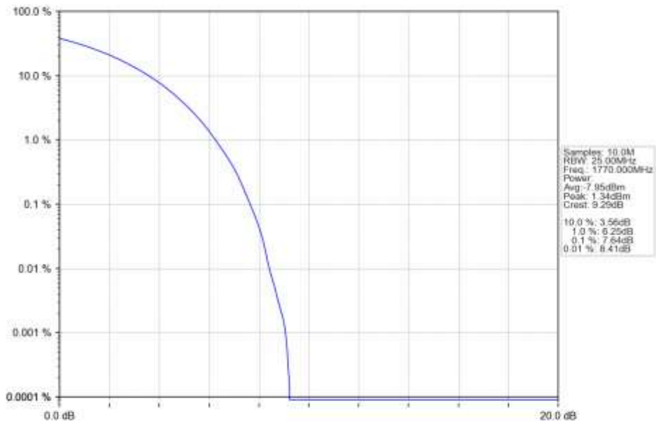
n66_15kHz_SISO_NTNV_20MHz_CP-OFDM_256_QAM_1770MHz_Outer_Full_Ant1
