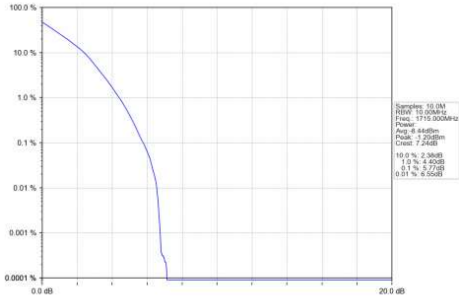
n66_30kHz_SISO_NTNV_10MHz_DFT-s-OFDM QPSK_1715MHz_Outer_Full_Ant1
