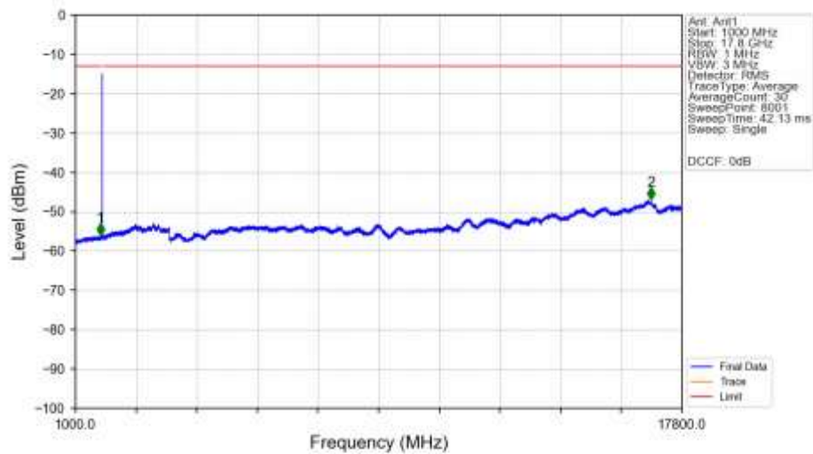
n66_15kHz_SISO_NTNV_10MHz_CP-OFDM_QPSK_1745MHz_Edge_1RB_Left_Ant1
