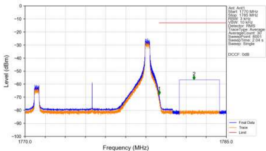
n66_30kHz_SISO_NTNV_10MHz_CP-OFDM_QPSK_1775MHz_Edge_1RB_Right_Ant1
