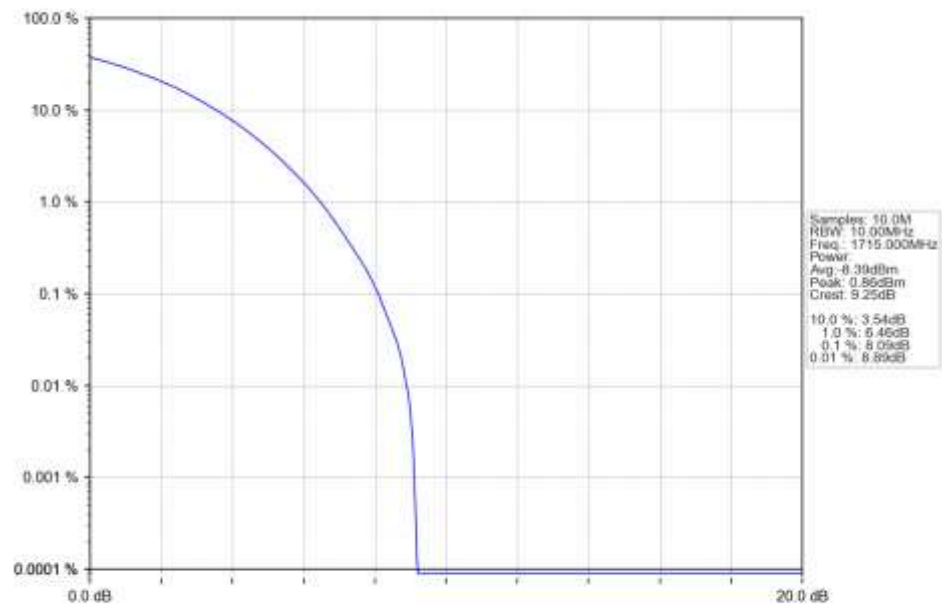
n66_30kHz_SISO_NTNV_10MHz_CP-OFDM_QPSK_1715MHz_Outer_Full_Ant1
