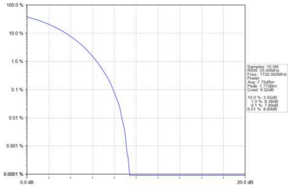
n66_30kHz_SISO_NTNV_20MHz_CP-OFDM_64_QAM_1720MHz_Outer_Full_Ant1
