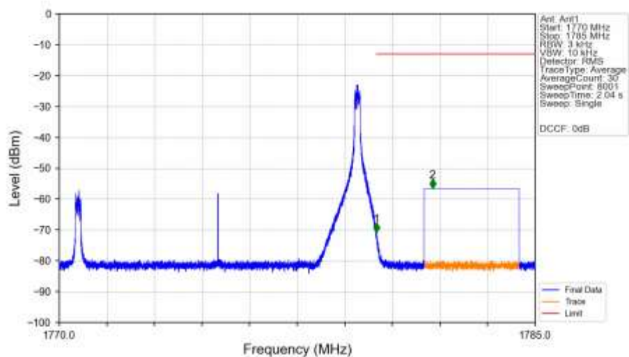
n66_15kHz_SISO_NTNV_10MHz_DFT-s-OFDM_QPSK_1775MHz_Inner_1RB_Right_Ant1
