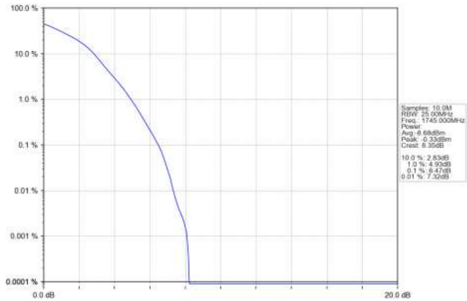
n66_30kHz_SISO_NTNV_20MHz_DFT-s-OFDM_16_QAM_1745MHz_Outer_Full_Ant1
