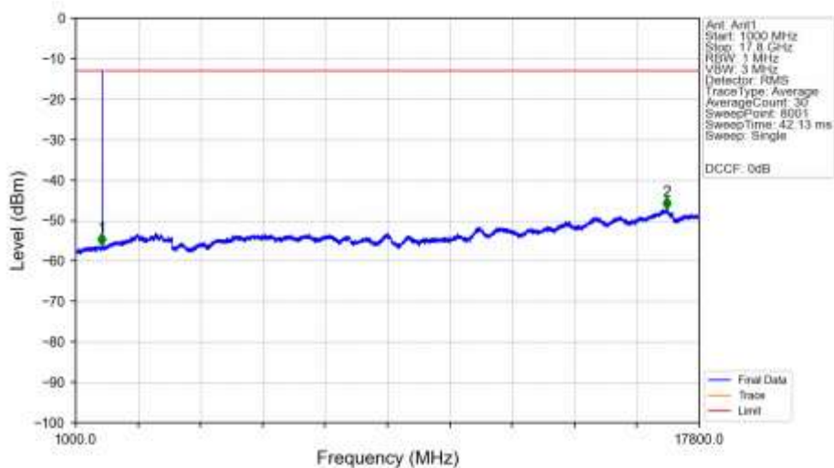
n66_15kHz_SISO_NTNV_5MHz_DFT-s-OFDM_QPSK_1712.5MHz_Edge_1RB_Left_Ant1
