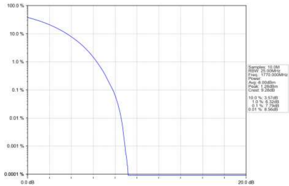
n66_15kHz_SISO_NTNV_20MHz_CP-OFDM_64_QAM_1770MHz_Outer_Full_Ant1
