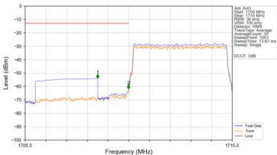
n66_15kHz_SISO_NTNV_5MHz_DFT-s-OFDM_QPSK_1712.5MHz_Outer_Full_Ant1
