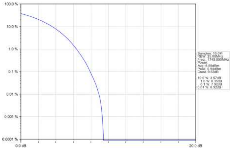
n66_15kHz_SISO_NTNV_20MHz_CP-OFDM_256_QAM_1745MHz_Outer_Full_Ant1
