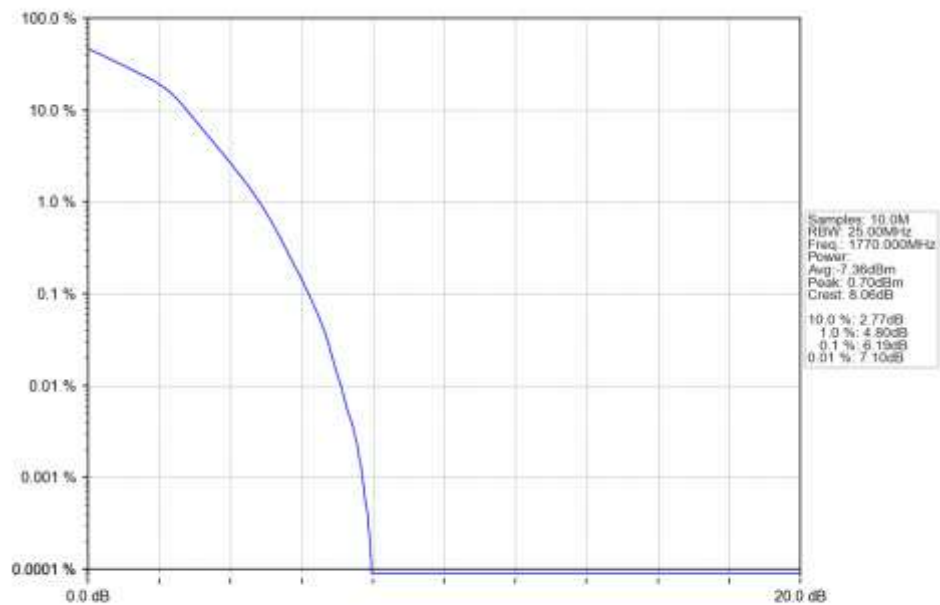
n66_30kHz_SISO_NTNV_20MHz_DFT-s-OFDM_16_QAM_1770MHz_Outer_Full_Ant1
