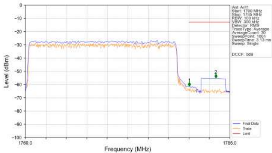
n66_15kHz_SISO_NTNV_20MHz_DFT-s-OFDM_QPSK_1770MHz_Outer_Full_Ant1
