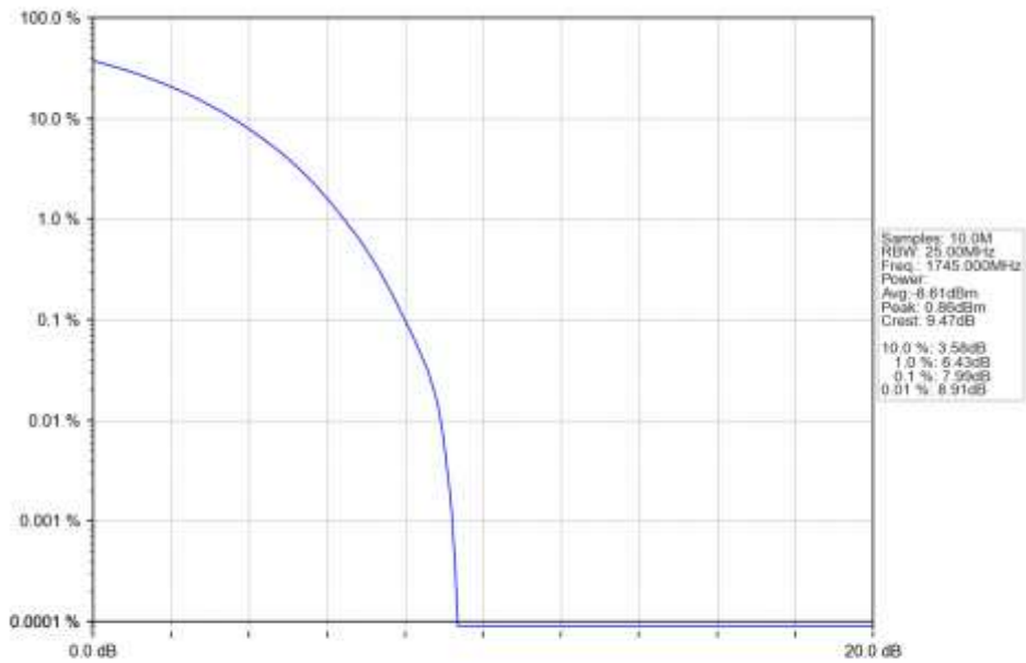
n66_15kHz_SISO_NTNV_20MHz_CP-OFDM_64_QAM_1745MHz_Outer_Full_Ant1
