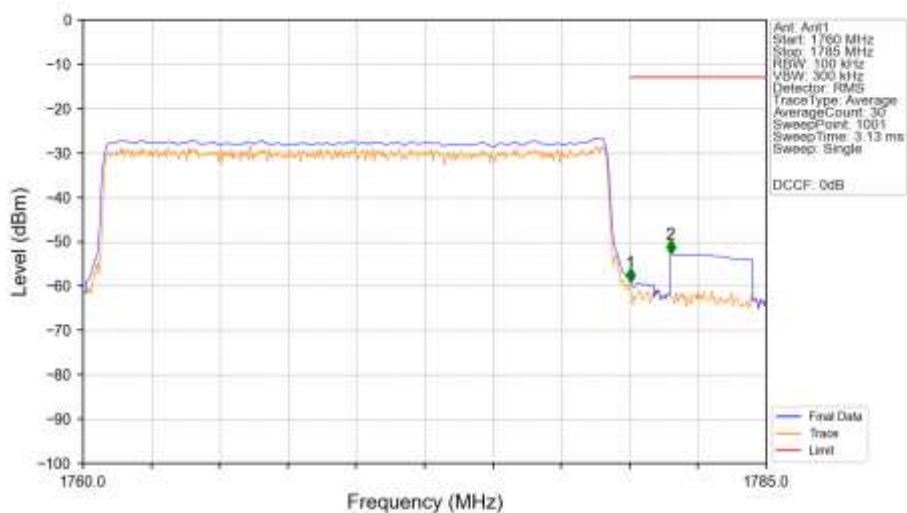
n66_30kHz_SISO_NTNV_20MHz_CP-OFDM_QPSK_1770MHz_Outer_Full_Ant1
