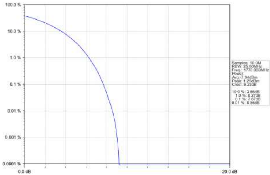
n66_15kHz_SISO_NTNV_20MHz_CP-OFDM_QPSK_1770MHz_Outer_Full_Ant1
