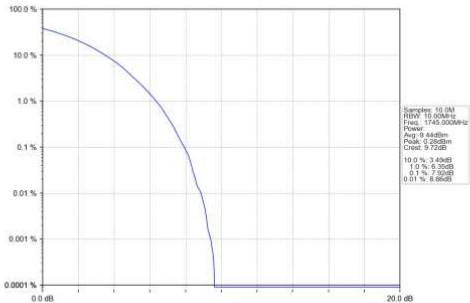
n66_30kHz_SISO_NTNV_10MHz_CP-OFDM_256_QAM_1745MHz_Outer_Full_Ant1
