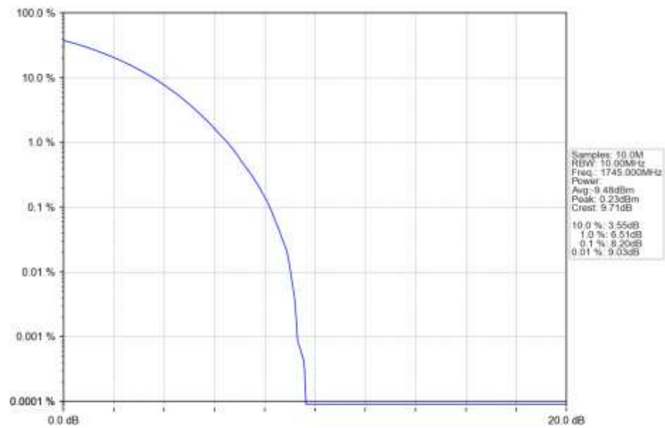
n66_30kHz_SISO_NTNV_10MHz_CP-OFDM_QPSK_1745MHz_Outer_Full_Ant1
