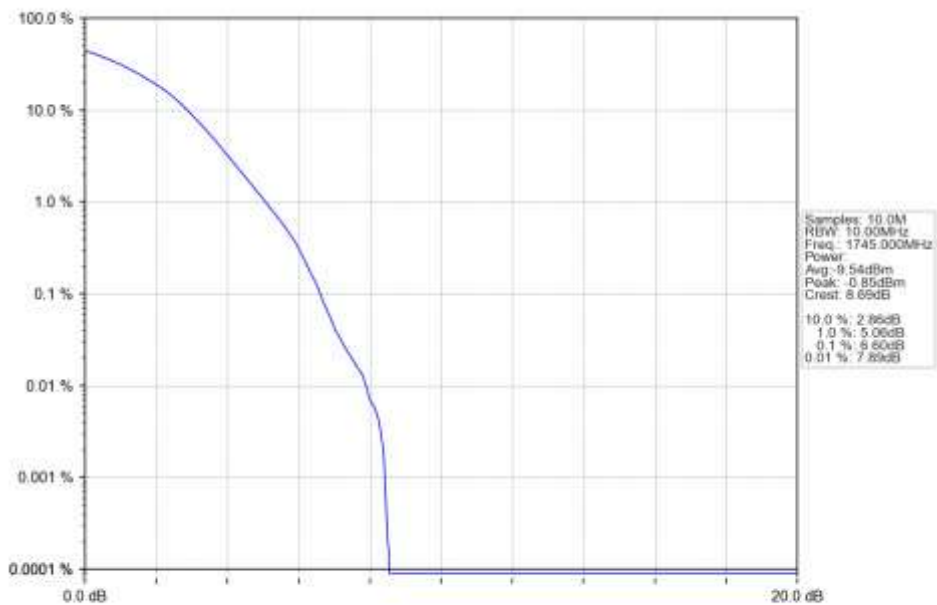
n66_30kHz_SISO_NTNV_10MHz_DFT-s-OFDM_256_QAM_1745MHz_Outer_Full_Ant1
