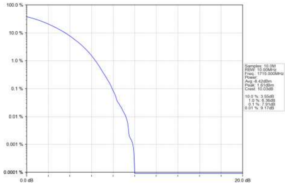
n66_30kHz_SISO_NTNV_10MHz_CP-OFDM_64_QAM_1715MHz_Outer_Full_Ant1
