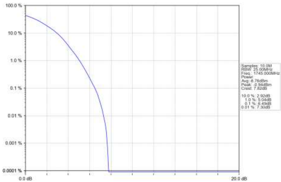
n66_15kHz_SISO_NTNV_20MHz_DFT-s-OFDM_64_QAM_1745MHz_Outer_Full_Ant1
