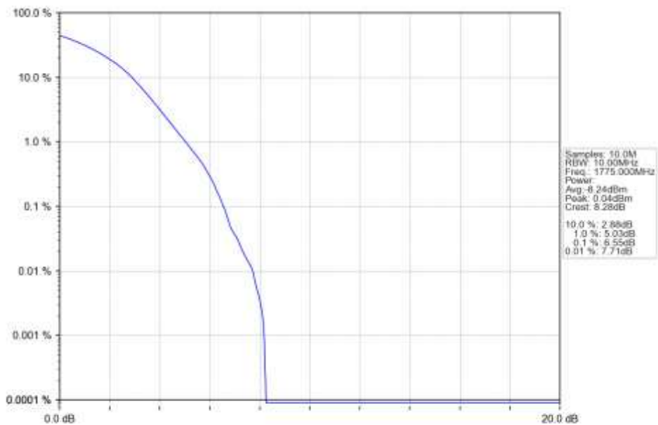
n66_30kHz_SISO_NTNV_10MHz_DFT-s-OFDM_256_QAM_1775MHz_Outer_Full_Ant1
