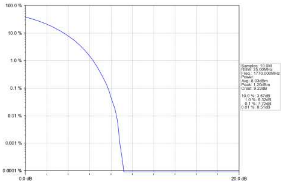
n66_15kHz_SISO_NTNV_20MHz_CP-OFDM_16_QAM_1770MHz_Outer_Full_Ant1
