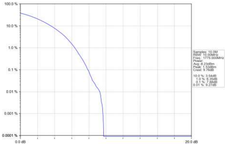
n66_30kHz_SISO_NTNV_10MHz_CP-OFDM_64_QAM_1775MHz_Outer_Full_Ant1
