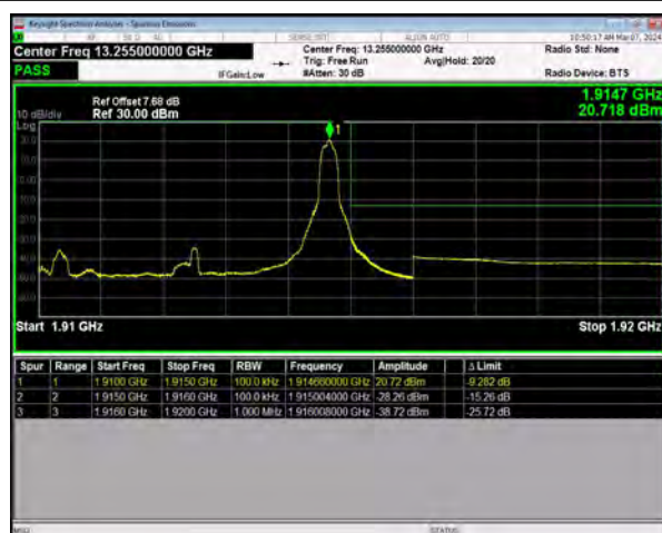
n25 SCS=15kHz DFT_BPSK BW=5MHz HighChannel=382500 RB=1@24
