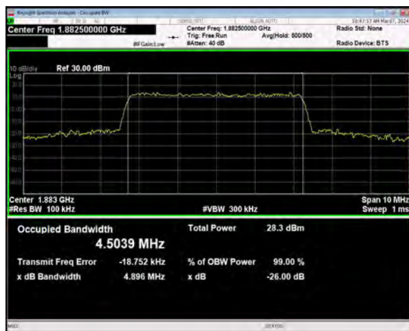
n25 SCS=15kHz CP_64QAM BW=5MHz Channel=376500 RB=25@0
