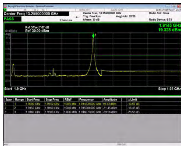
n25 SCS=15kHz DFT_QPSK BW=15MHz HighChannel=381500 RB=1@78
