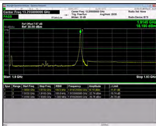
n25 SCS=15kHz DFT_16QAM BW=15MHz HighChannel=381500 RB=1@78
