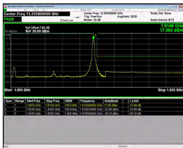
n25 SCS=15kHz DFT_64QAM BW=10MHz HighChannel=382000 RB=1@51
