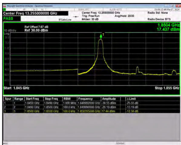
n25 SCS=15kHz DFT_16QAM BW=5MHz LowChannel=370500 RB=1@0
