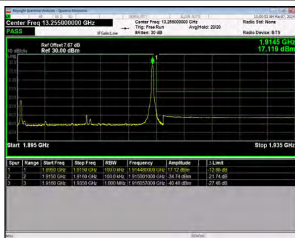
n25 SCS=15kHz DFT_64QAM BW=20MHz HighChannel=381000 RB=1@105
