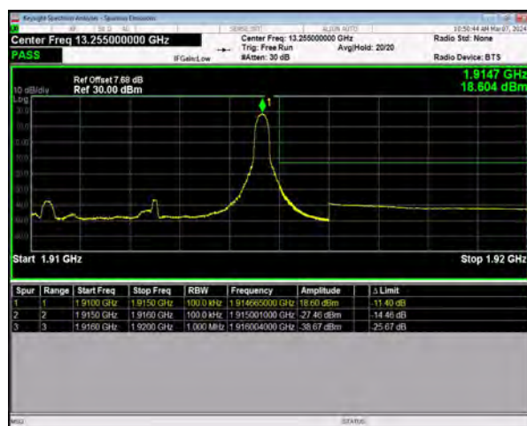
n25 SCS=15kHz DFT_16QAM BW=5MHz HighChannel=382500 RB=1@24
