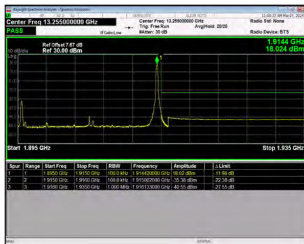
n25 SCS=15kHz DFT_16QAM BW=20MHz HighChannel=381000 RB=1@105
