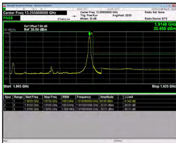
n25 SCS=15kHz DFT_BPSK BW=10MHz HighChannel=382000
