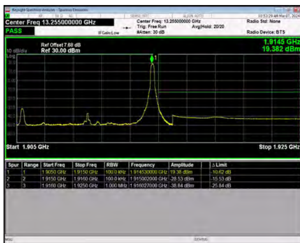
n25 SCS=15kHz DFT_QPSK BW=10MHz HighChannel=382000
