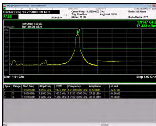
n25 SCS=15kHz DFT_64QAM BW=5MHz HighChannel=382500 RB=1@24
