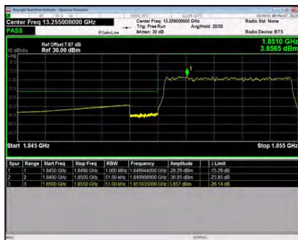
n25 SCS=15kHz DFT_64QAM BW=5MHz LowChannel=370500 RB=25@0
