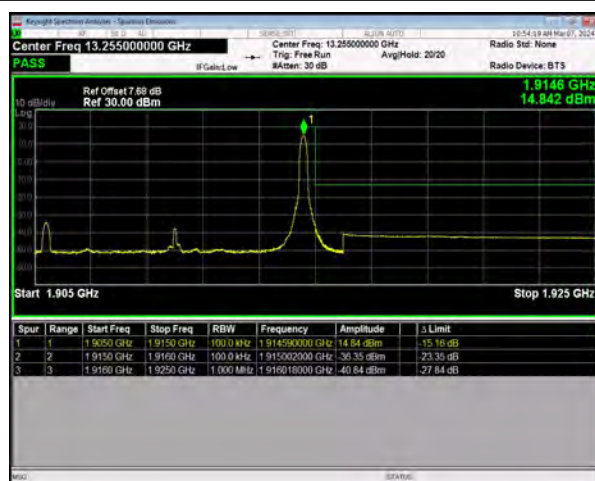
n25 SCS=15kHz DFT_256QAM BW=10MHz HighChannel=382000 RB=1@51
