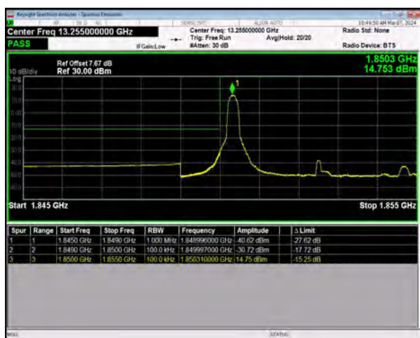
n25 SCS=15kHz DFT_256QAM BW=5MHz LowChannel=370500 RB=1@0
