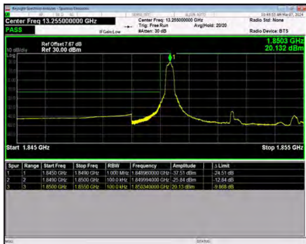
n25 SCS=15kHz DFT_BPSK BW=5MHz LowChannel=370500 RB=1@0
