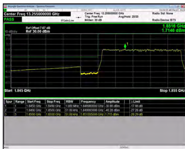
n25 SCS=15kHz DFT_256QAM BW=5MHz LowChannel=370500 RB=25@0
