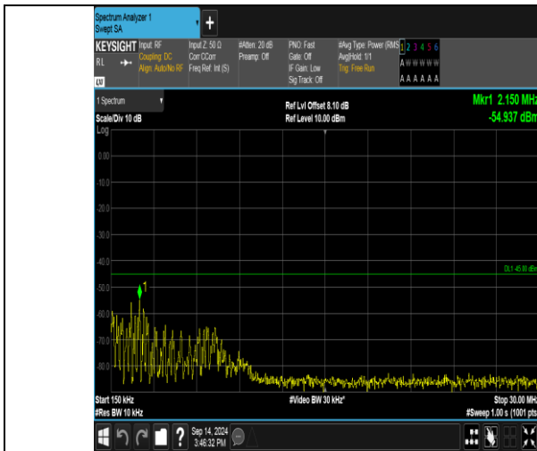
Band41_20MHz_16QAM_40140_100RB#0_0.15~30_0.15~30
