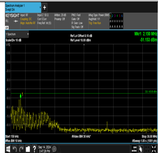
Band41_20MHz_QPSK_40590_1RB#0_0.15~30_0.15~30
