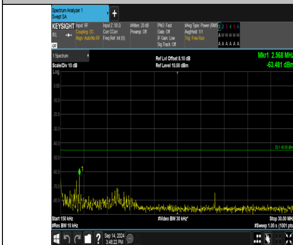
Band41_20MHz_16QAM_40590_1RB#0_0.15~30_0.15~30
