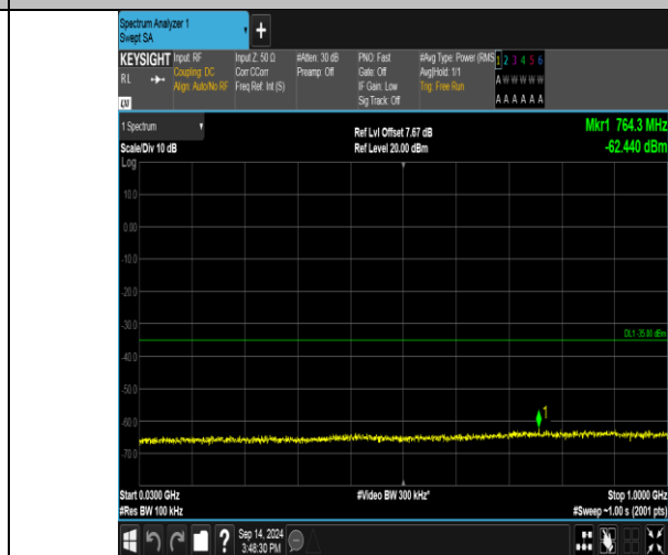
Band41_20MHz_16QAM_40590_1RB#0_30~1000_30~1000
