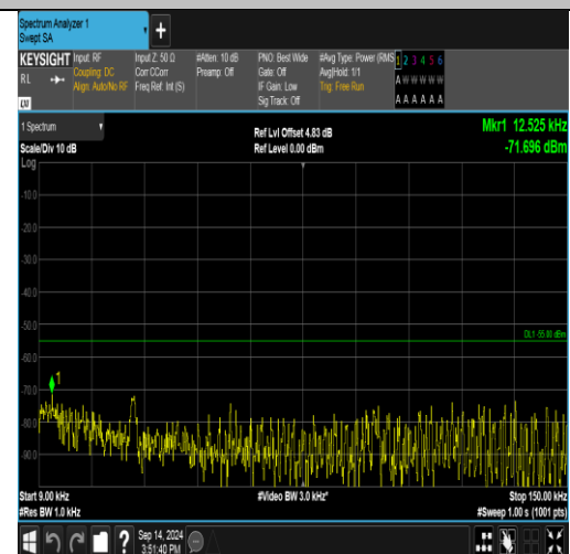
Band41_20MHz_16QAM_40590_100RB#0_0.009~0.15_0.009~0.15
