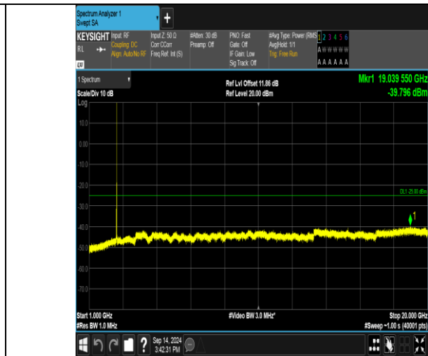
Band41_20MHz_QPSK_40140_1RB#0_1000~20000_1000~20000
