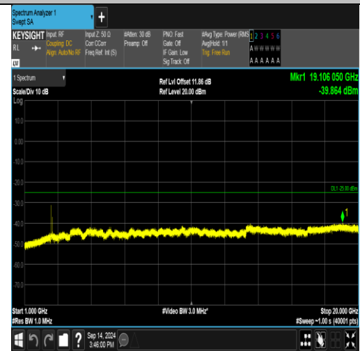
Band41_20MHz_QPSK_40140_100RB#0_1000-20000_1000-20000
