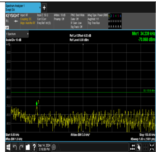
Band41_15MHz_16QAM_41165_1RB#74_0.009-0.15_0.009-0.15
