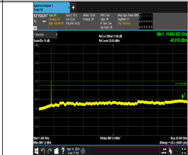
Band41_20MHz_QPSK_40140_1RB#99_1000~20000_1000~20000
