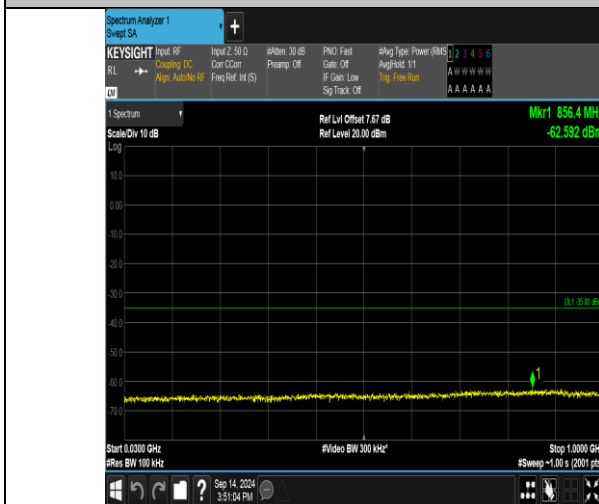
Band41_20MHz_QPSK_40590_100RB#0_30~1000_30~1000
