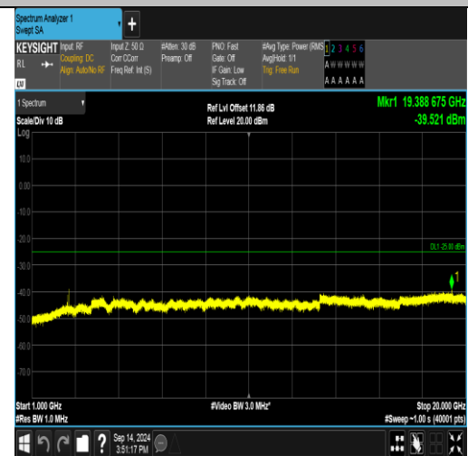
Band41_20MHz_QPSK_40590_100RB#0_1000~20000_1000~20000
