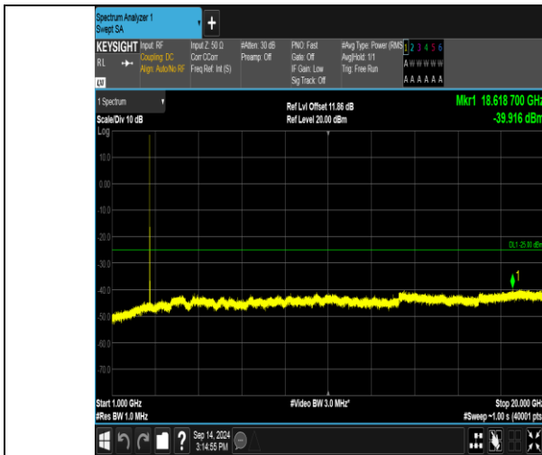
Band41_15MHz_16QAM_41165_1RB#0_1000-20000_1000-20000
