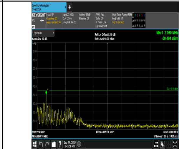
Band41_20MHz_QPSK_40140_1RB#99_0.15~30_0.15~30
