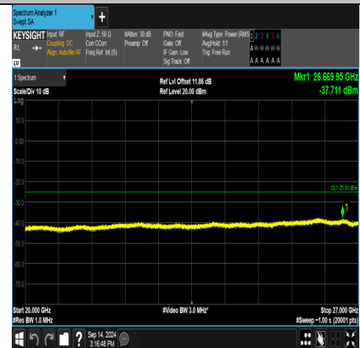
Band41_15MHz_16QAM_41165_1RB#74_20000-27000_20000-27000
