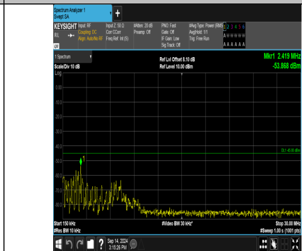
Band41_15MHz_QPSK_41165_1RB#74_0.15-30_0.15-30
