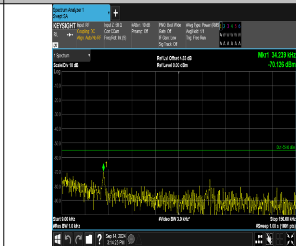
Band41_15MHz_16QAM_41165_1RB#0_0.009~0.15_0.009~0.15
