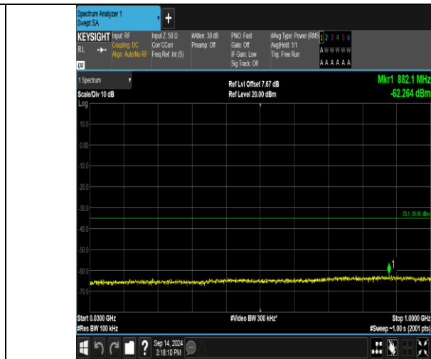
Band41_15MHz_16QAM_41165_75RB#0_30~1000_30~1000
