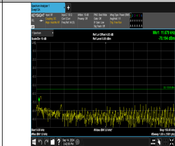
Band41_20MHz_16QAM_40140_1RB#0_0.009~0.15_0.009~0.15
