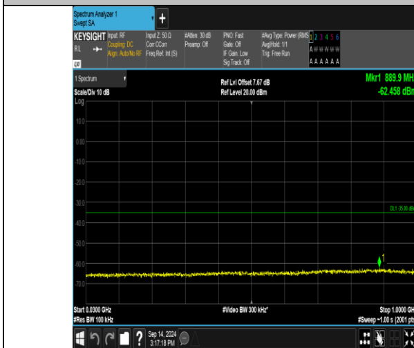
Band41_15MHz_QPSK_41165_75RB#0_30-1000_30-1000
