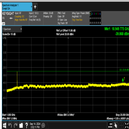
Band41_20MHz_16QAM_40590_100RB#0_1000~20000_1000~20000
