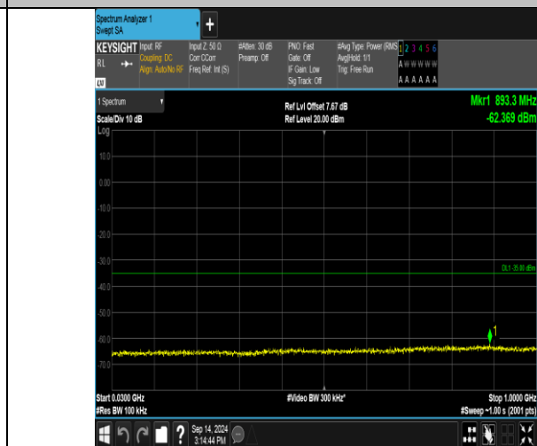
Band41_15MHz_16QAM_41165_1RB#0_30~1000_30~1000
