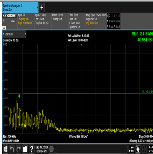
Band41_20MHz_16QAM_40590_1RB#99_0.15~30_0.15~30
