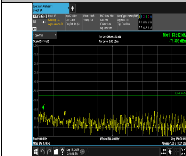
Band41_15MHz_QPSK_41165_1RB#74_0.009-0.15_0.009-0.15
