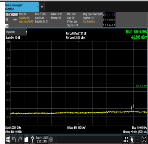
Band41_20MHz_16QAM_40590_1RB#99_30~1000_30~1000
