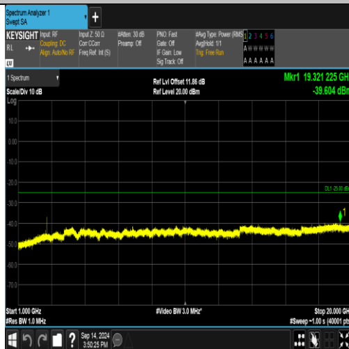
Band41_20MHz_16QAM_40590_1RB#99_1000~20000_1000~20000
