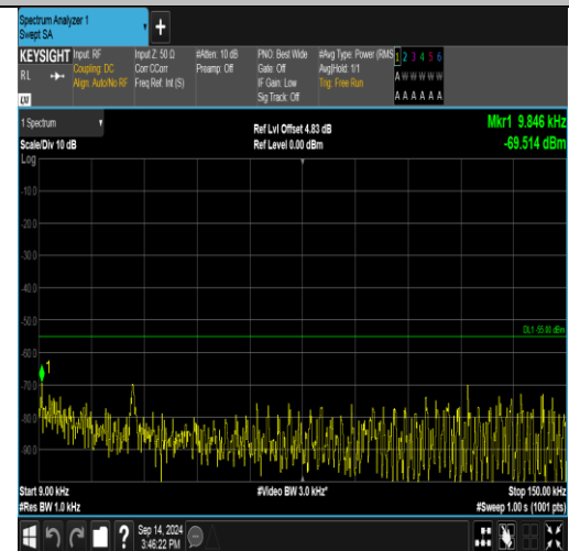
Band41_20MHz_16QAM_40140_100RB#0_0.009-0.15_0.009-0.15
