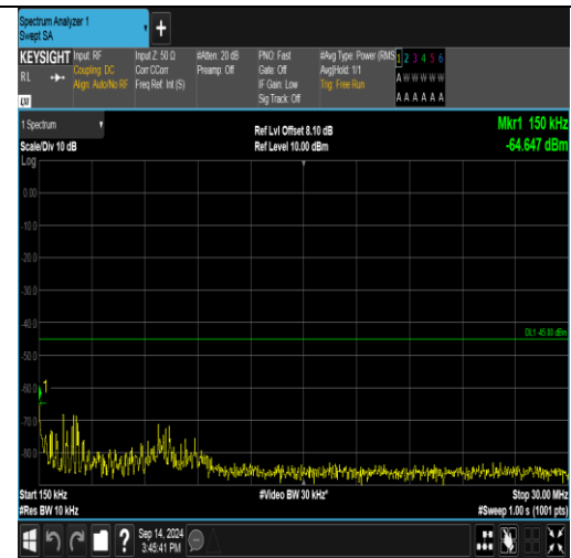
Band41_20MHz_QPSK_40140_100RB#0_0.15-30_0.15-30
