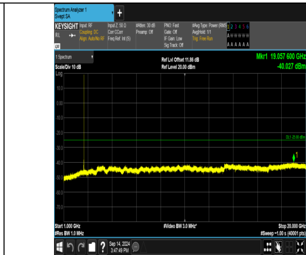
Band41_20MHz_QPSK_40590_1RB#0_1000~20000_1000~20000
