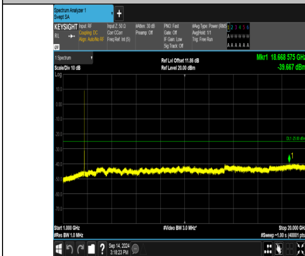
Band41_15MHz_16QAM_41165_75RB#0_1000~20000_1000~20000
