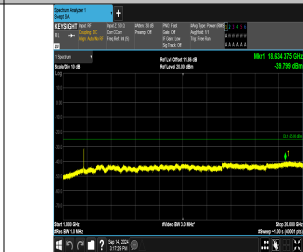
Band41_15MHz_QPSK_41165_75RB#0_1000-20000_1000-20000
