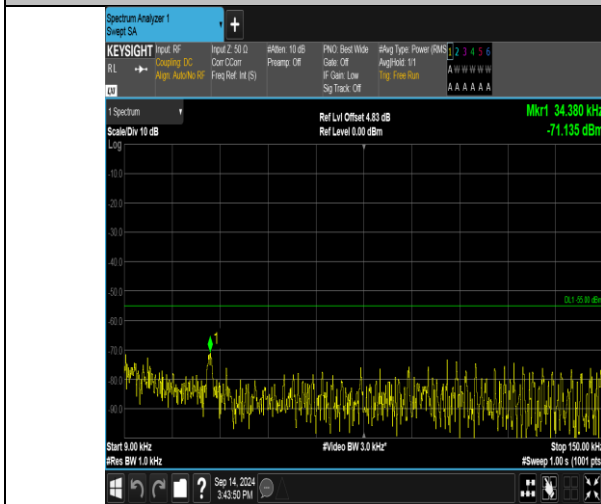
Band41_20MHz_QPSK_40140_1RB#99_0.009~0.15_0.009~0.15
