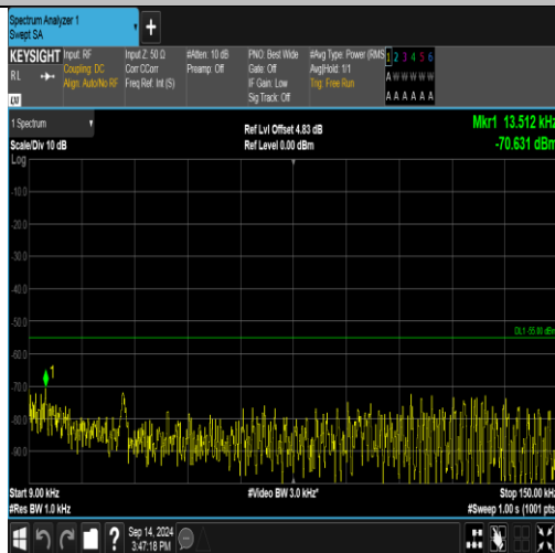
Band41_20MHz_QPSK_40590_1RB#0_0.009~0.15_0.009~0.15
