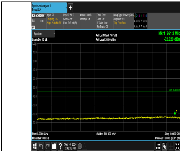
Band41_20MHz_QPSK_40140_1RB#0_30~1000_30~1000
