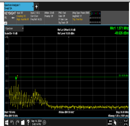
Band41_20MHz_QPSK_40590_1RB#99_0.15~30_0.15~30
