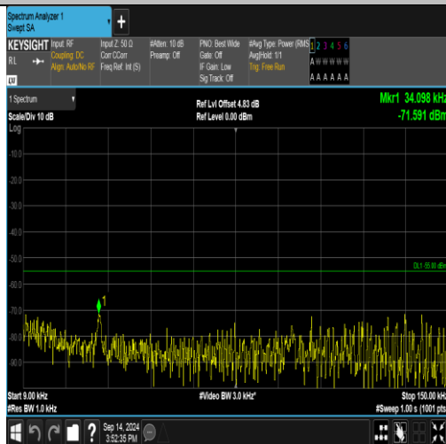
Band41_20MHz_QPSK_41140_1RB#0_0.009~0.15_0.009~0.15
