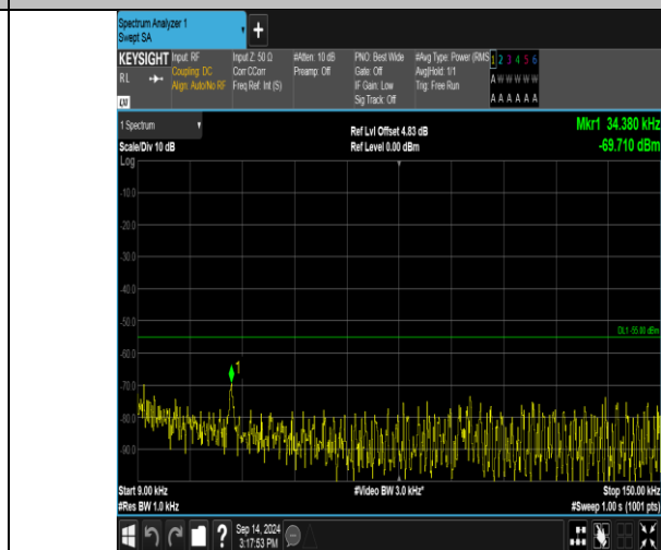
Band41_15MHz_16QAM_41165_75RB#0_0.009-0.15_0.009-0.15
