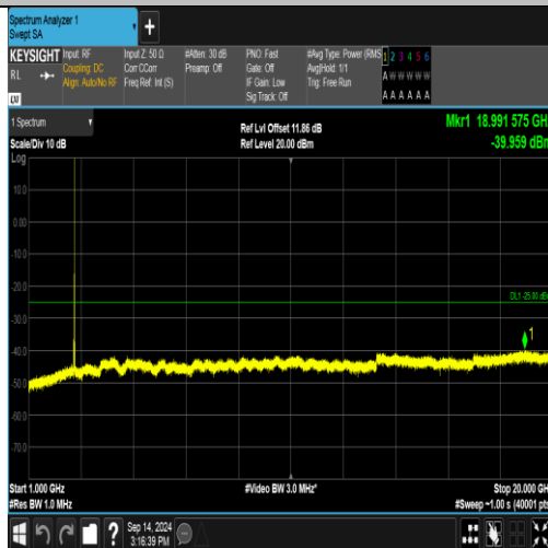
Band41_15MHz_16QAM_41165_1RB#74_1000-20000_1000-20000
