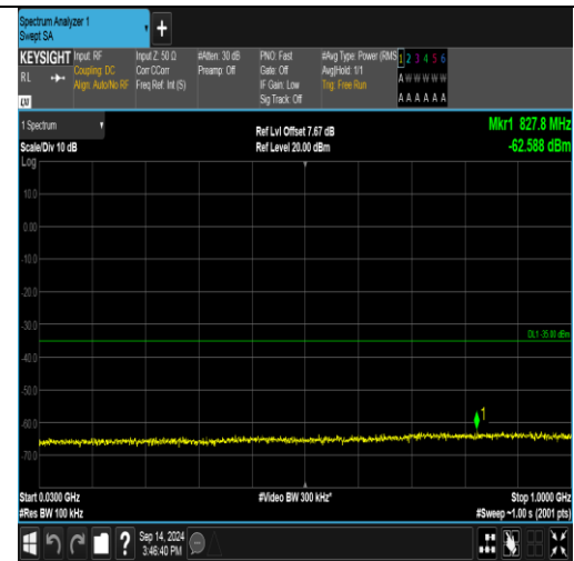
Band41_20MHz_16QAM_40140_100RB#0_30~1000_30~1000
