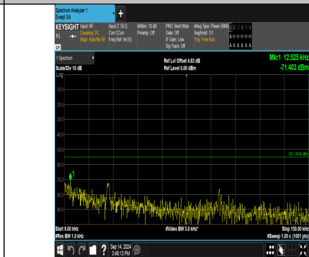
Band41_20MHz_16QAM_40590_1RB#0_0.009~0.15_0.009~0.15
