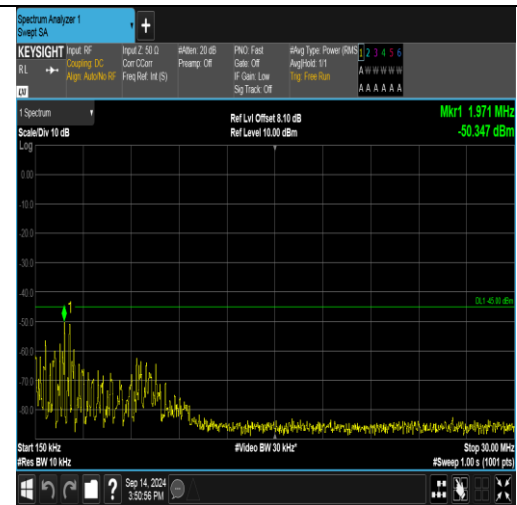
Band41_20MHz_QPSK_40590_100RB#0_0.15~30_0.15~30
