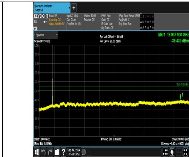
Band41_15MHz_QPSK_41165_1RB#0_1000~20000_1000~20000
