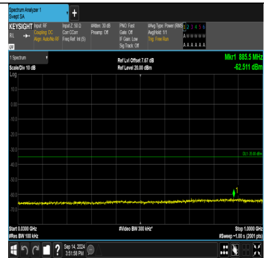
Band41_20MHz_16QAM_40590_100RB#0_30~1000_30~1000
