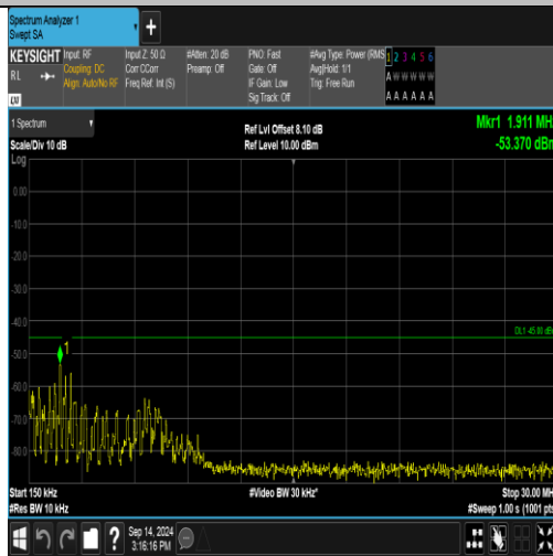
Band41_15MHz_16QAM_41165_1RB#74_0.15-30_0.15-30
