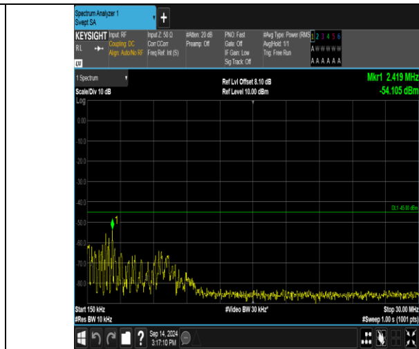
Band41_15MHz_QPSK_41165_75RB#0_0.15-30_0.15-30
