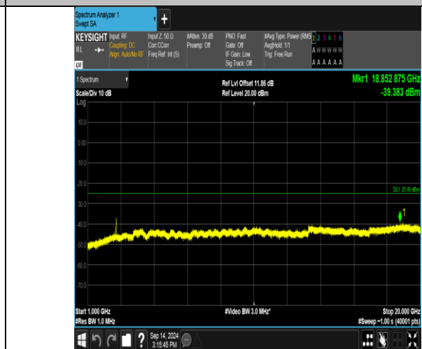
Band41_15MHz_QPSK_41165_1RB#74_1000-20000_1000-20000
