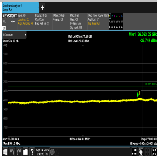
Band41_20MHz_QPSK_40140_100RB#0_20000-27000_20000-27000
