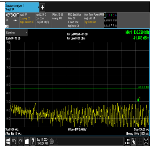
Band41_20MHz_16QAM_40590_1RB#99_0.009~0.15_0.009~0.15
