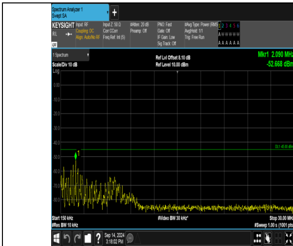
Band41_15MHz_16QAM_41165_75RB#0_0.15~30_0.15~30
