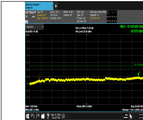
Band41_20MHz_16QAM_40140_1RB#0_1000~20000_1000~20000
