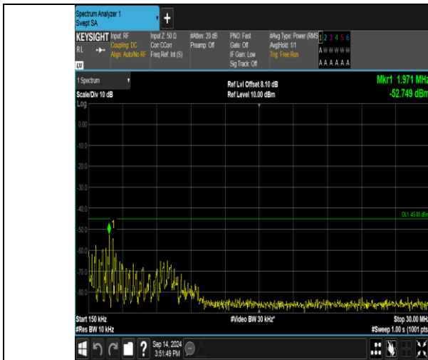
Band41_20MHz_16QAM_40590_100RB#0_0.15~30_0.15~30
