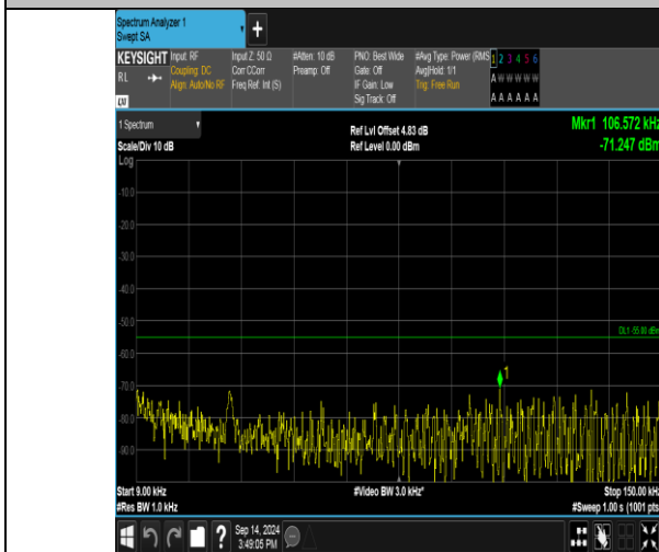
Band41_20MHz_QPSK_40590_1RB#99_0.009~0.15_0.009~0.15
