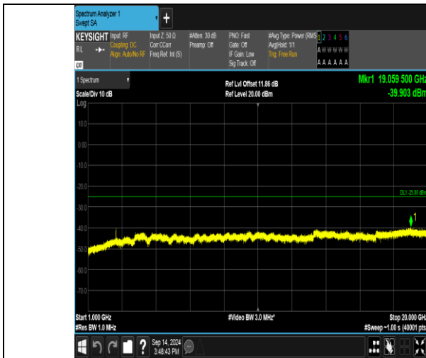
Band41_20MHz_16QAM_40590_1RB#0_1000~20000_1000~20000
