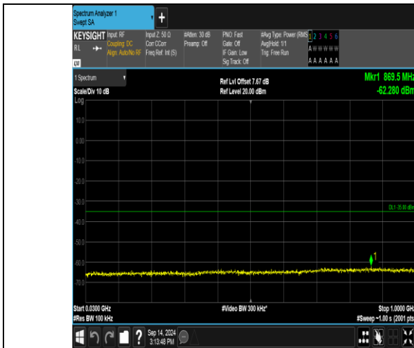
Band41_15MHz_QPSK_41165_1RB#0_30~1000_30~1000
