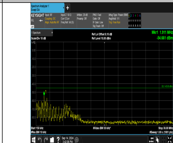
Band41_20MHz_QPSK_40140_1RB#0_0.15~30_0.15~30
