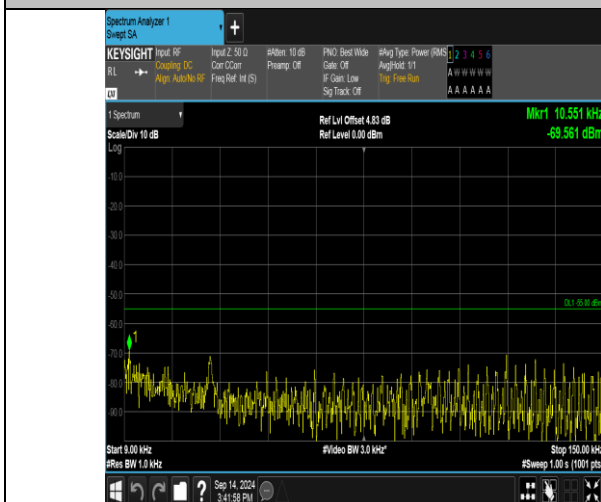
Band41_20MHz_QPSK_40140_1RB#0_0.009~0.15_0.009~0.15
