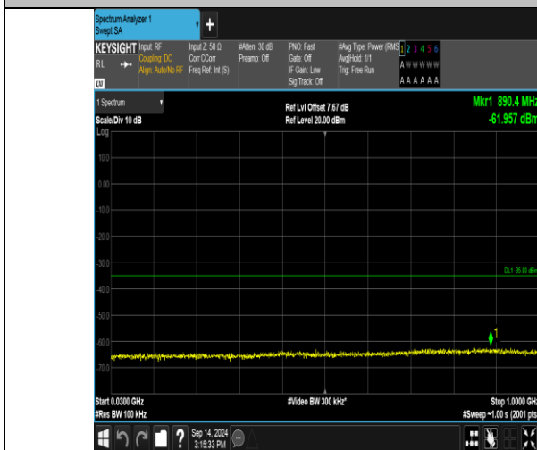
Band41_15MHz_QPSK_41165_1RB#74_30-1000_30-1000
