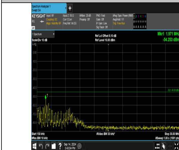
Band41_20MHz_16QAM_40140_1RB#0_0.15~30_0.15~30
