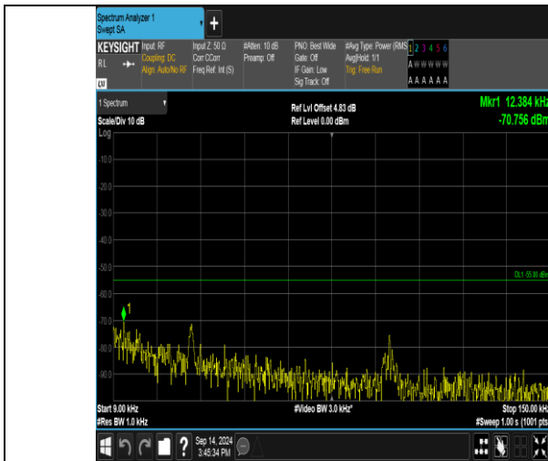
Band41_20MHz_QPSK_40140_100RB#0_0.009-0.15_0.009-0.15
