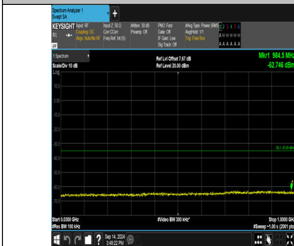
Band41_20MHz_QPSK_40590_1RB#99_30~1000_30~1000
