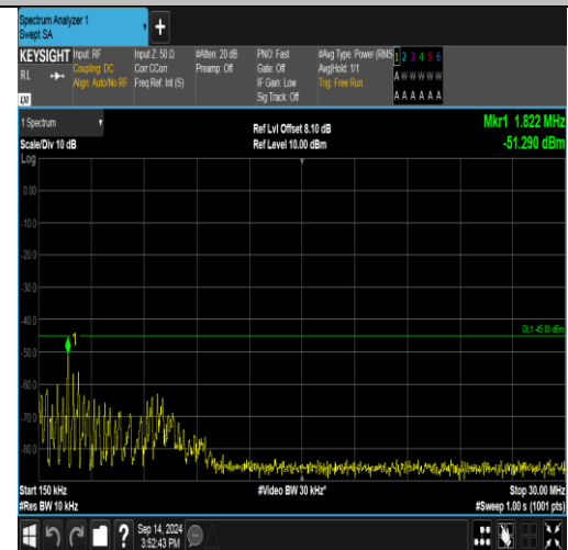
Band41_20MHz_QPSK_41140_1RB#0_0.15~30_0.15~30
