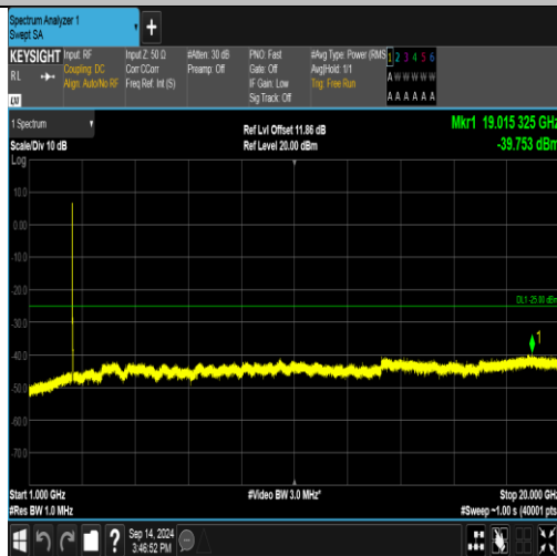
Band41_20MHz_16QAM_40140_100RB#0_1000~20000_1000~20000
