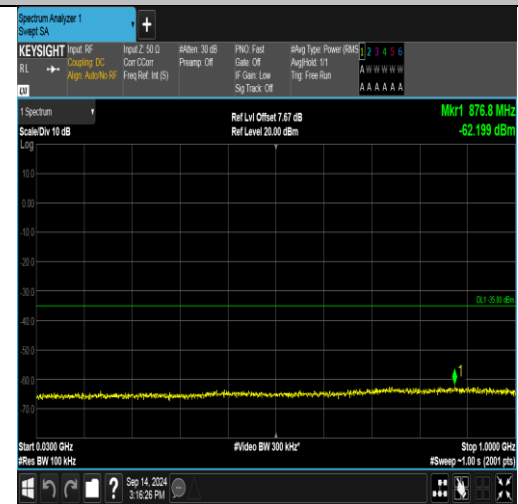
Band41_15MHz_16QAM_41165_1RB#74_30-1000_30-1000
