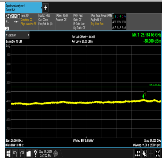
Band41_20MHz_16QAM_40140_100RB#0_20000~27000_20000~27000
