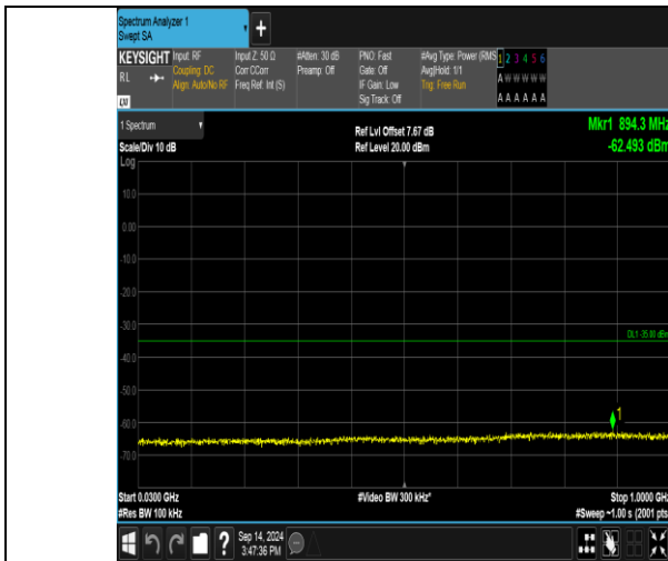
Band41_20MHz_QPSK_40590_1RB#0_30~1000_30~1000
