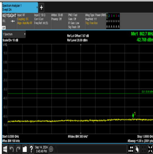
Band41_20MHz_QPSK_40140_100RB#0_30-1000_30-1000
