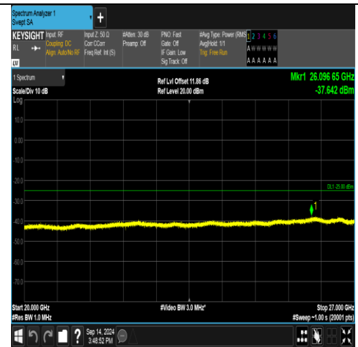
Band41_20MHz_16QAM_40590_1RB#0_20000~27000_20000~27000
